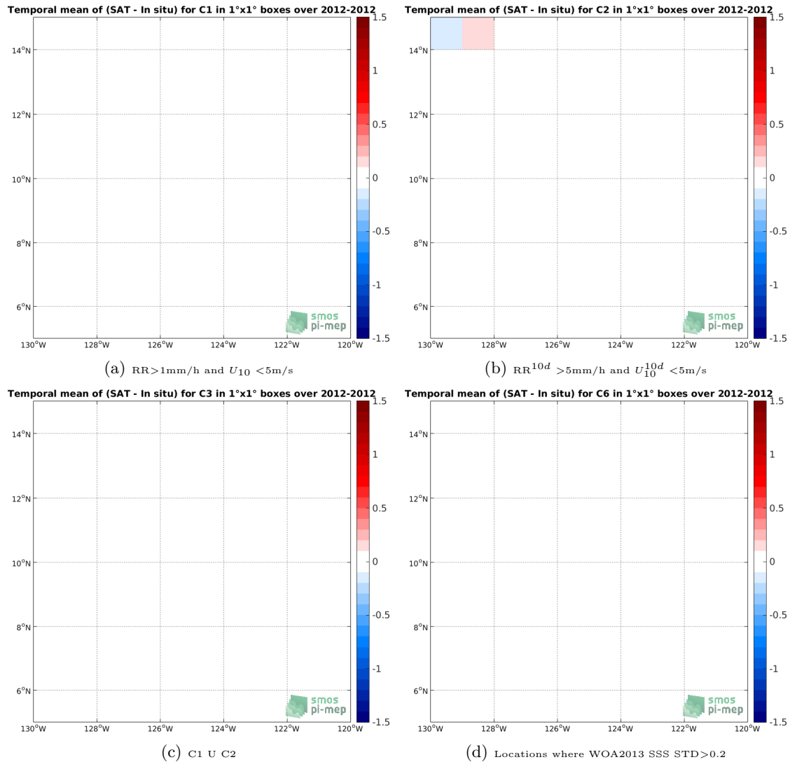
Figure 12: Temporal mean gridded over spatial boxes of size 1^\circ \times 1^\circ of \Delta SSS (SMOS-L4-CATDS-CECOS-IFREMER-V2-WEEKLY-0.5DEG - TSG-GOSUD-Research-vessel) for 4 different sub-datasets corresponding to: RR > 1\text{mm/h} and U_{10} < 5\text{m/s} (a), RR^{10d} > 5\text{mm/h} and U_{10}^{10d} < 5\text{m/s} (b), C1 U C2 (c), Locations where WOA2013 SSS STD > 0.2 (d).
