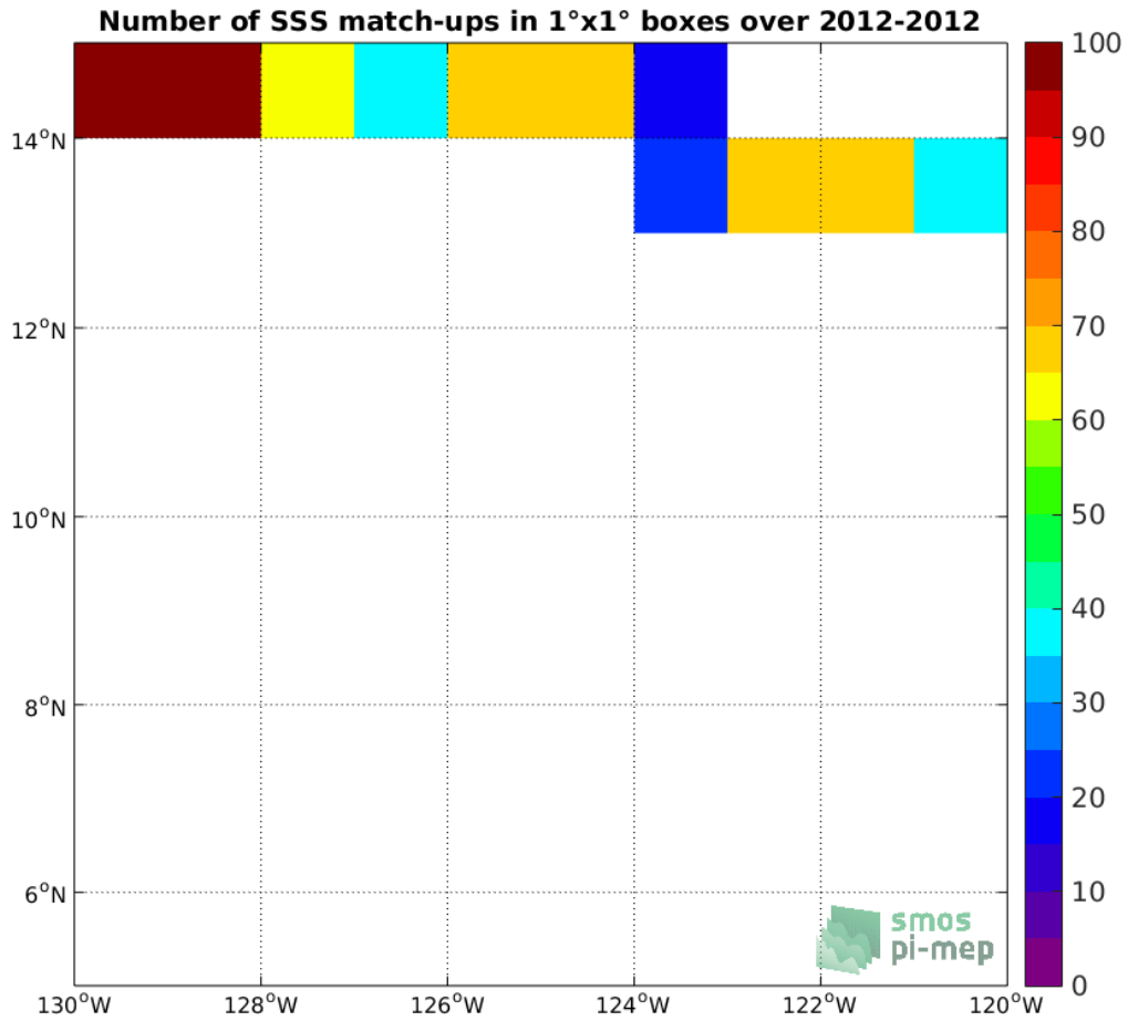
Figure 4: Number of SSS match-ups between TSG-GOSUD-Research-vessel SSS and the SMOS-L4-CATDS-CECOS-IFREMER-V2-WEEKLY-0.5DEG SSS product for the SPURS 2 Pi-MEP region over 1°x1° boxes and for the full satellite product period.
