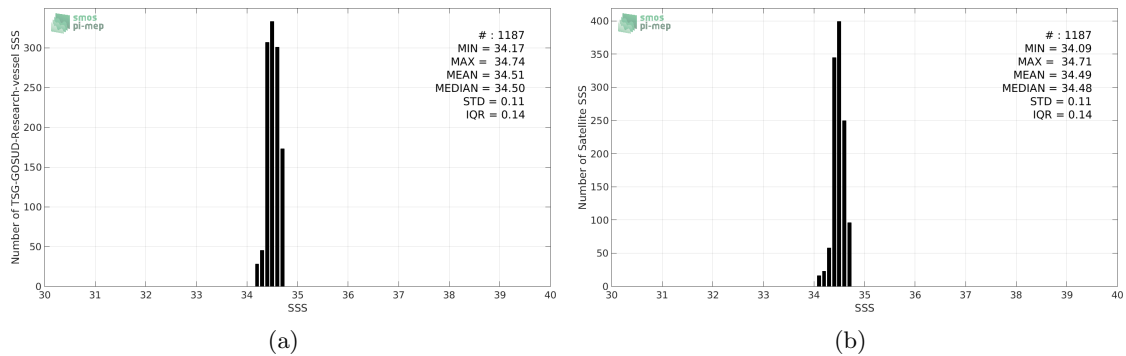
Figure 2: Histograms of SSS from TSG-GOSUD-Research-vessel (a) and SMOS-L4-CATDS-CECOS-IFREMER-V2-WEEKLY-0.5DEG (b) considering all match-up pairs per bins of 0.1 over the SPURS 2 Pi-MEP region and for the full satellite product period.
