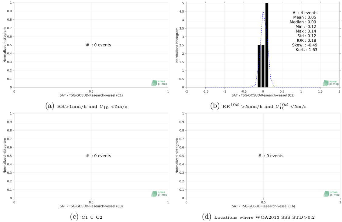
Figure 13: Normalized histogram of \Delta\text{SSS} (SMOS-L4-CATDS-CECOS-IFREMER-V2-WEEKLY-0.5DEG - TSG-GOSUD-Research-vessel) for 6 different subdatasets corresponding to: RR > 1\text{mm/h} and U_{10} < 5\text{m/s} (a), RR^{10d} > 5\text{mm/h} and U_{10}^{10d} < 5\text{m/s} (b), C1 \cup C2 (c), Locations where WOA2013 SSS STD > 0.2 (d).
