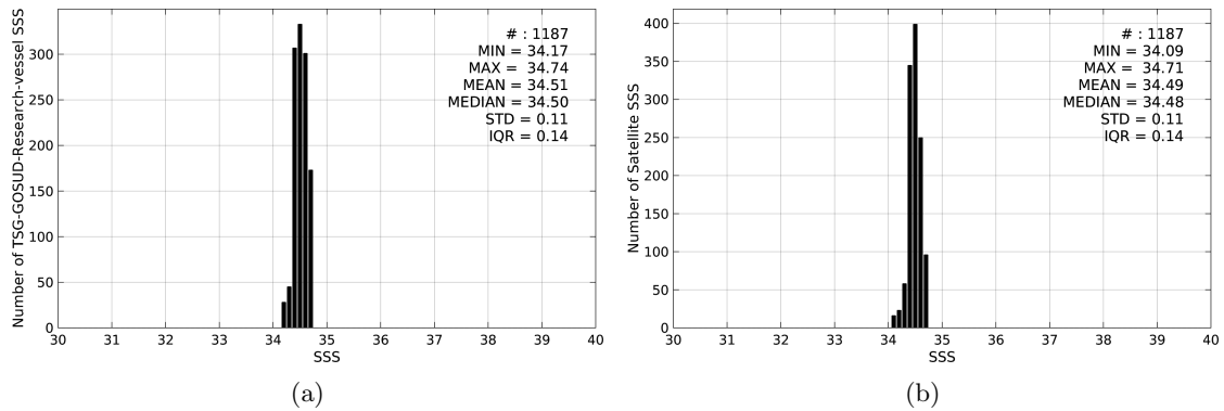
Figure 2: Histograms of SSS from TSG-GOSUD-Research-vessel (a) and SMOS-L4-CATDS-CECOS-IFREMER-V2-WEEKLY-0.5DEG (b) considering all match-up pairs per bins of 0.1 over the SPURS 2 Pi-MEP region and for the full satellite product period.
