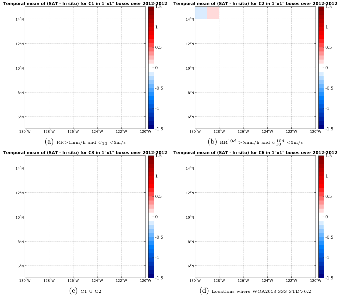
Figure 12: Temporal mean gridded over spatial boxes of size 1^\circ \times 1^\circ of \Delta SSS (SMOS-L4-CATDS-CECOS-IFREMER-V2-WEEKLY-0.5DEG - TSG-GOSUD-Research-vessel) for 4 different sub-datasets corresponding to: RR > 1\text{mm/h} and U_{10} < 5\text{m/s} (a), RR^{10d} > 5\text{mm/h} and U_{10}^{10d} < 5\text{m/s} (b), C1 U C2 (c), Locations where WOA2013 SSS STD > 0.2 (d).
