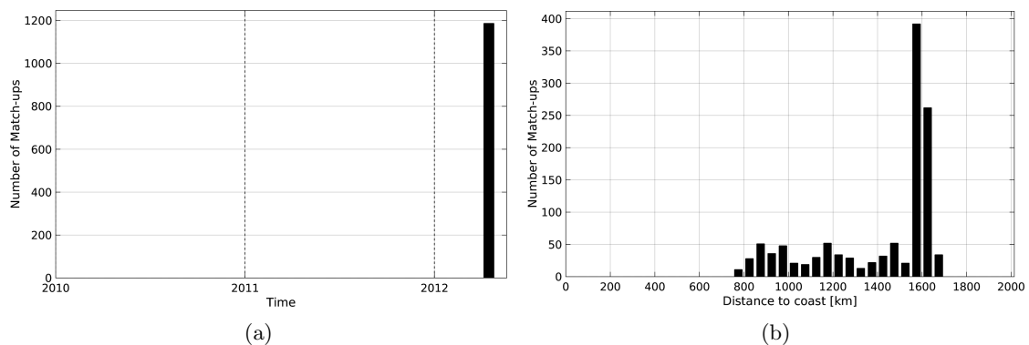
Figure 1: Number of match-ups between TSG-GOSUD-Research-vessel and SMOS-L4-CATDS-CECOS-IFREMER-V2-WEEKLY-0.5DEG SSS as a function of time (a) and as function of the distance to coast (b) over the SPURS 2 Pi-MEP region and for the full satellite product period.
