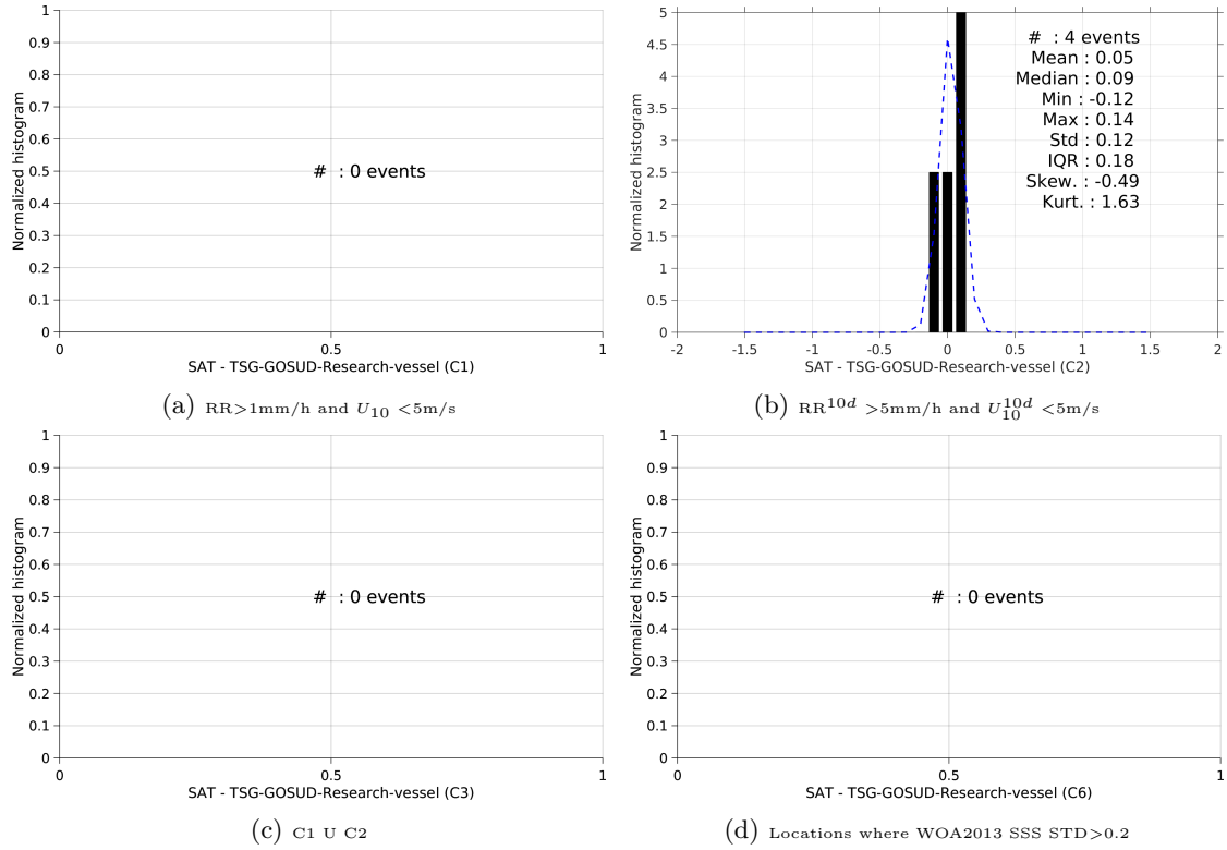
Figure 13: Normalized histogram of \Delta\text{SSS} (SMOS-L4-CATDS-CECOS-IFREMER-V2-WEEKLY-0.5DEG - TSG-GOSUD-Research-vessel) for 6 different subdatasets corresponding to: RR > 1\text{mm/h} and U_{10} < 5\text{m/s} (a), RR^{10d} > 5\text{mm/h} and U_{10}^{10d} < 5\text{m/s} (b), C1 \cup C2 (c), Locations where WOA2013 SSS STD > 0.2 (d).
