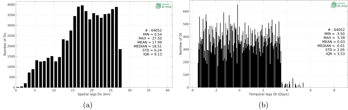
Figure 5: Histograms of the spatial (a) and temporal (b) lags between the time of the Seaglider measurements and the date of the corresponding SMOS L4 v2 Weekly (CATDS-CECOS-IFREMER) SSS product.
