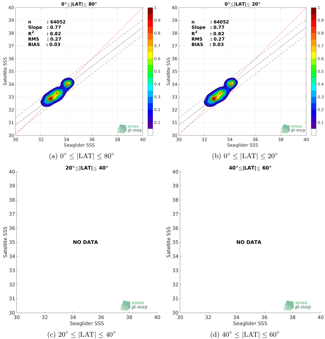
Figure 9: Contour maps of the concentration of SMOS L4 v2 Weekly (CATDS-CECOS-IFREMER) SSS (y-axis) versus Seaglider SSS (x-axis) at match-up pairs for different latitude bands. For each plot, the red line shows x=y . The black thin and dashed lines indicate a linear fit through the data cloud and the \pm 95\% confidence levels, respectively. The number match-up pairs n , the slope and R^2 coefficient of the linear fit, the root mean square (RMS) and the mean bias between satellite and in situ data are indicated for each latitude band in each plots.
