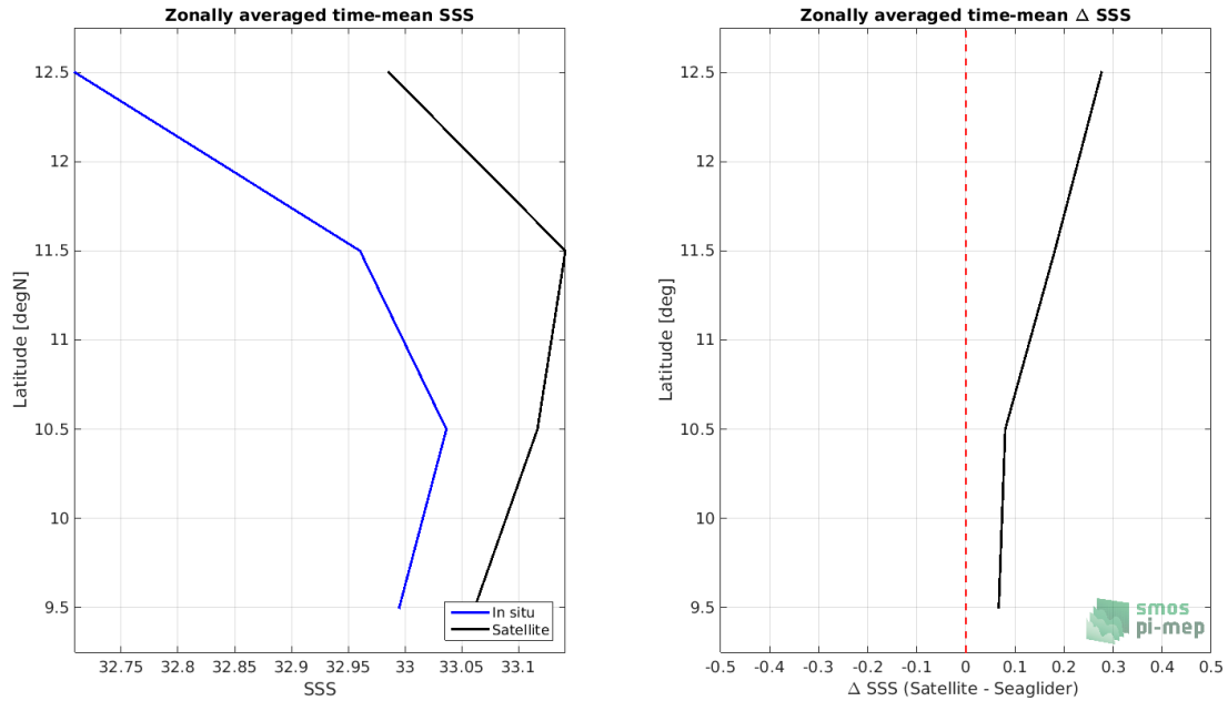
Figure 8: Left panel: Zonal mean SSS from SMOS L4 v2 Weekly (CATDS-CECOS-IFREMER) satellite product (black) and from Seaglider (blue). Right panel: Zonal mean of \Delta SSS (Satellite - Seaglider) for all the collected Pi-MEP match-up pairs estimated over the full satellite product period.
