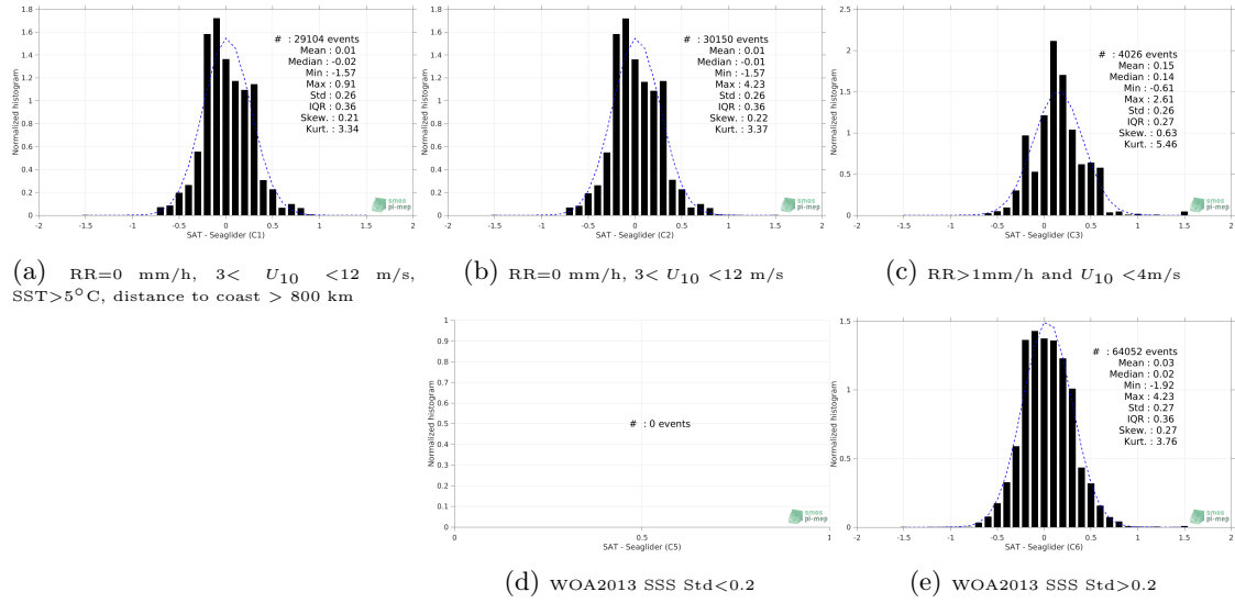
Figure 13: Normalized histogram of \Delta SSS (SMOS L4 v2 Weekly (CATDS-CECOS-IFREMER) - Seaglider) for 5 different subdatasets corresponding to: RR=0 mm/h, 3 < U_{10} < 12 m/s, SST > 5°C, distance to coast > 800 km (a), RR=0 mm/h, 3 < U_{10} < 12 m/s (b), RR > 1mm/h and U_{10} < 4 m/s (c), WOA2013 SSS Std < 0.2 (d), WOA2013 SSS Std > 0.2 (e).
