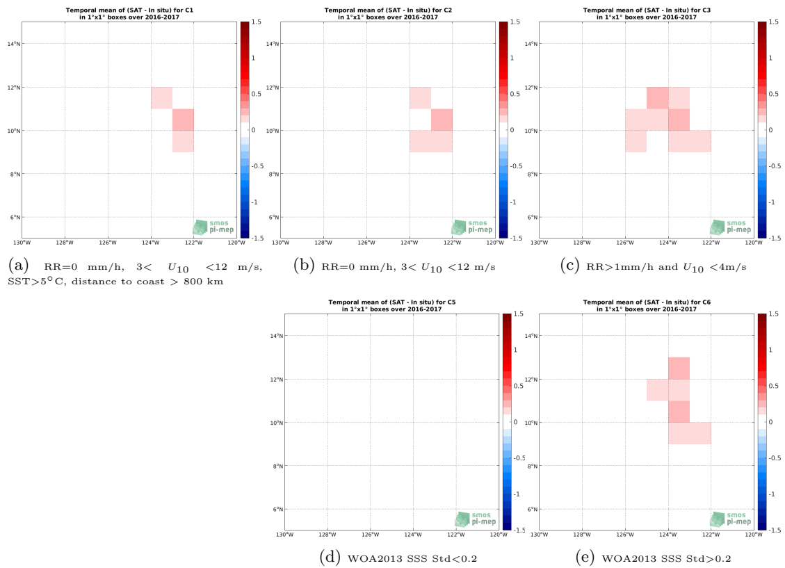
Figure 12: Temporal mean gridded over spatial boxes of size 1^\circ \times 1^\circ of \Delta SSS (SMOS L4 v2 Weekly (CATDS-CECOS-IFREMER) - Seaglider) for 5 different subdatasets corresponding to:RR=0 mm/h, 3 < U_{10} < 12 m/s, SST >5^\circ\text{C} , distance to coast > 800 km (a), RR=0 mm/h, 3 < U_{10} < 12 m/s (b), RR >1 mm/h and U_{10} < 4 m/s (c), WOA2013 SSS Std <0.2 (d), WOA2013 SSS Std >0.2 (e).
