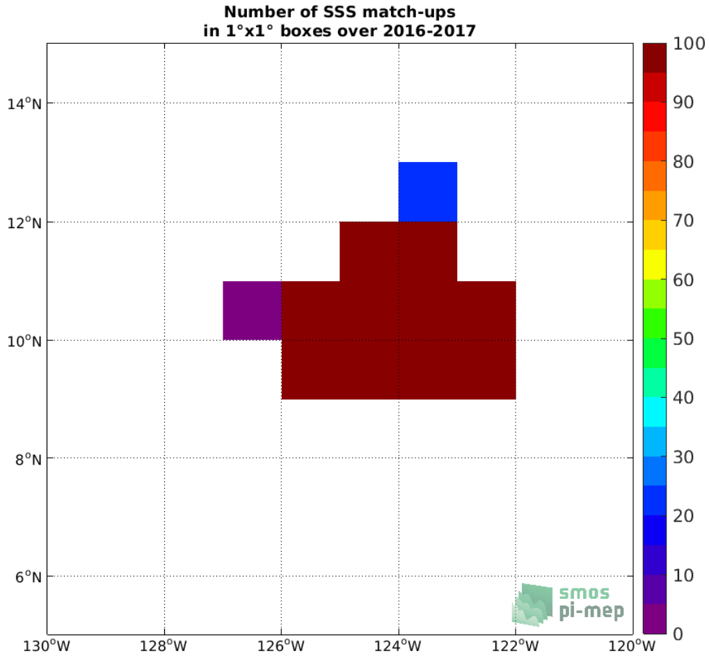
Figure 4: Number of SSS match-ups between Seaglider SSS and the SMOS L4 v2 Weekly (CATDS-CECOS-IFREMER) SSS product for the SPURS 2 Pi-MEP region over 1°x1° boxes and for the full satellite product period.
