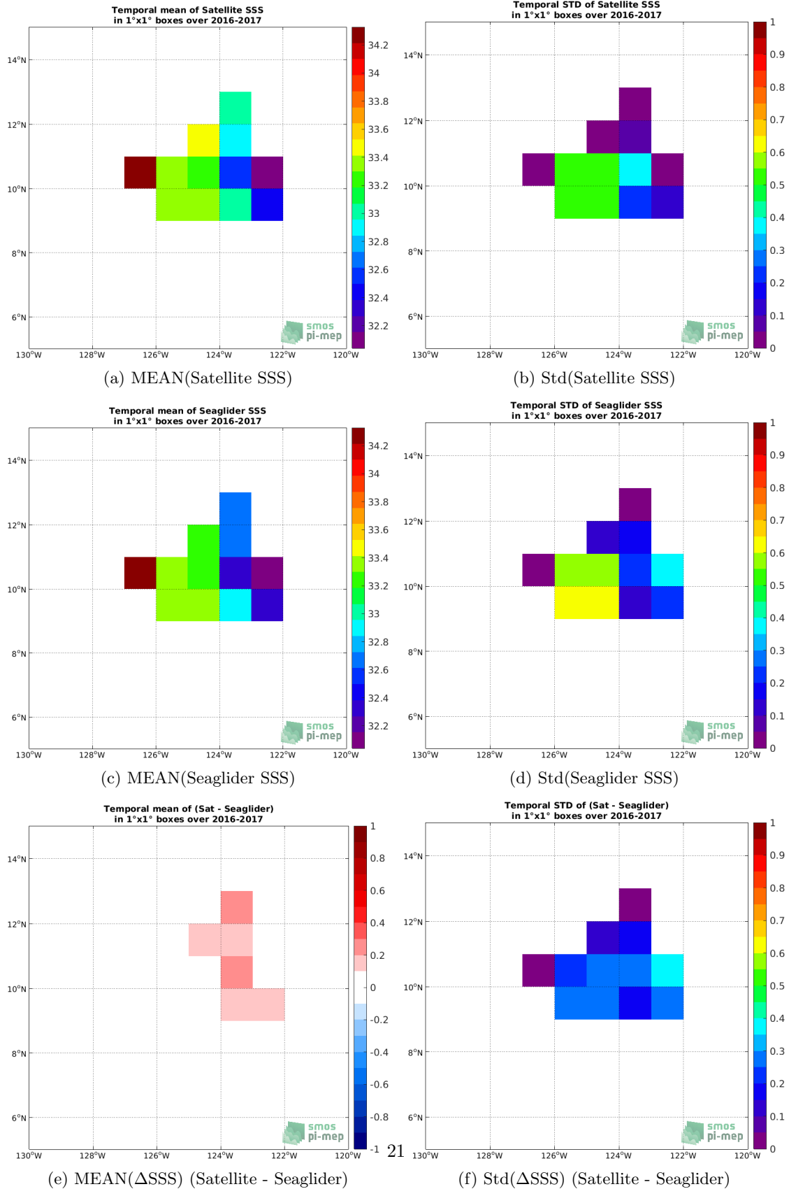
Figure 6: Temporal mean (left) and Std (right) of SSS from SMOS L4 v2 Weekly (CATDS-CECOS-IFREMER) (top), Seaglider (middle), and of \Delta SSS (Satellite - Seaglider). Only match-up pairs are used to generate these maps.
