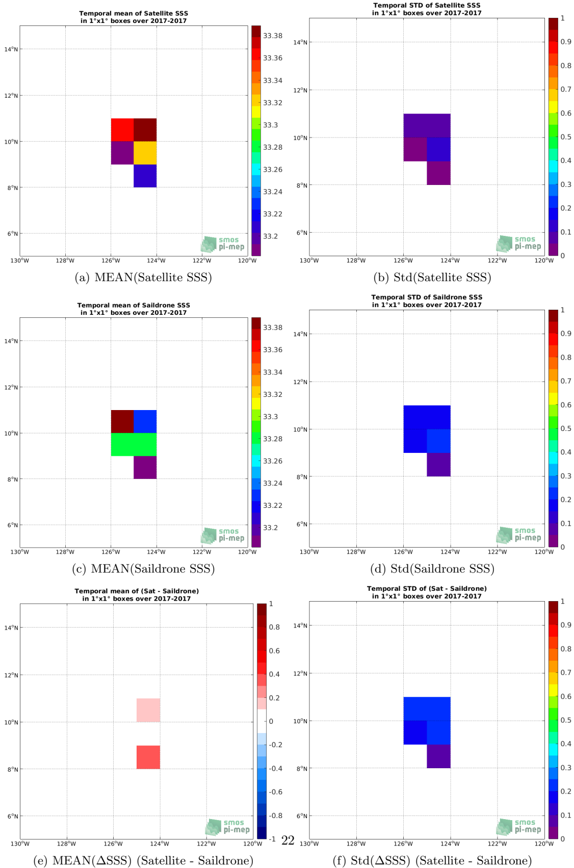
Figure 6: Temporal mean (left) and Std (right) of SSS from SMOS L4 v2 Weekly (CATDS-CECOS-IFREMER) (top), Saildrone (middle), and of \Delta SSS (Satellite - Saildrone). Only match-pairs are used to generate these maps.
