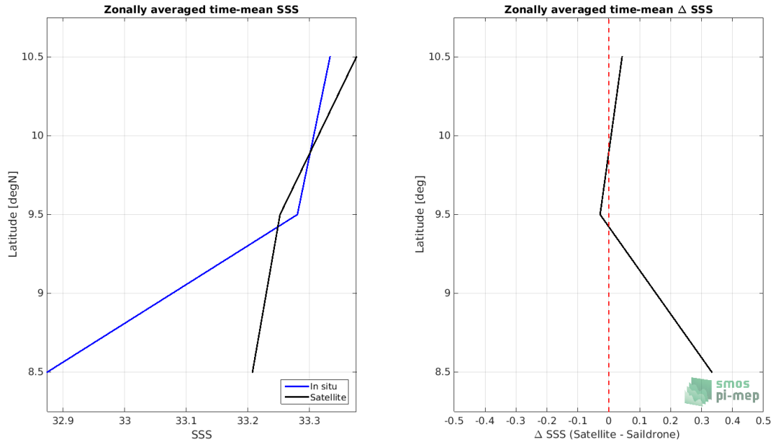
Figure 8: Left panel: Zonal mean SSS from SMOS L4 v2 Weekly (CATDS-CECOS-IFREMER) satellite product (black) and from Saildrone (blue). Right panel: Zonal mean of \Delta SSS (Satellite - Saildrone) for all the collected Pi-MEP match-up pairs estimated over the full satellite product period.
