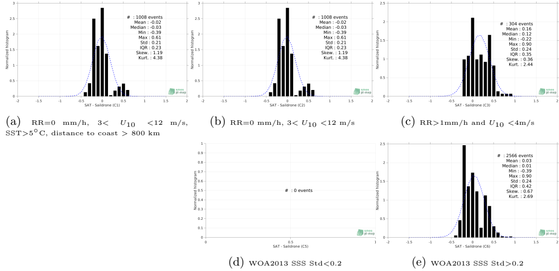
Figure 13: Normalized histogram of \Delta SSS (SMOS L4 v2 Weekly (CATDS-CECOS-IFREMER) - Saildrone) for 5 different subdatasets corresponding to: RR=0 mm/h, 3 < U_{10} < 12 m/s, SST > 5°C, distance to coast > 800 km (a), RR=0 mm/h, 3 < U_{10} < 12 m/s (b), RR > 1mm/h and U_{10} < 4 m/s (c), WOA2013 SSS Std < 0.2 (d), WOA2013 SSS Std > 0.2 (e).
