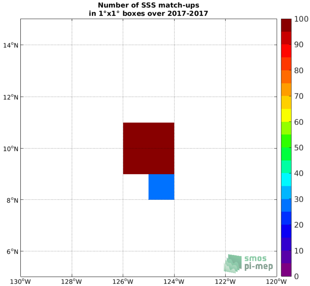
Figure 4: Number of SSS match-ups between Saildrone SSS and the SMOS L4 v2 Weekly (CATDS-CECOS-IFREMER) SSS product for the SPURS 2 Pi-MEP region over 1°x1° boxes and for the full satellite product period.
