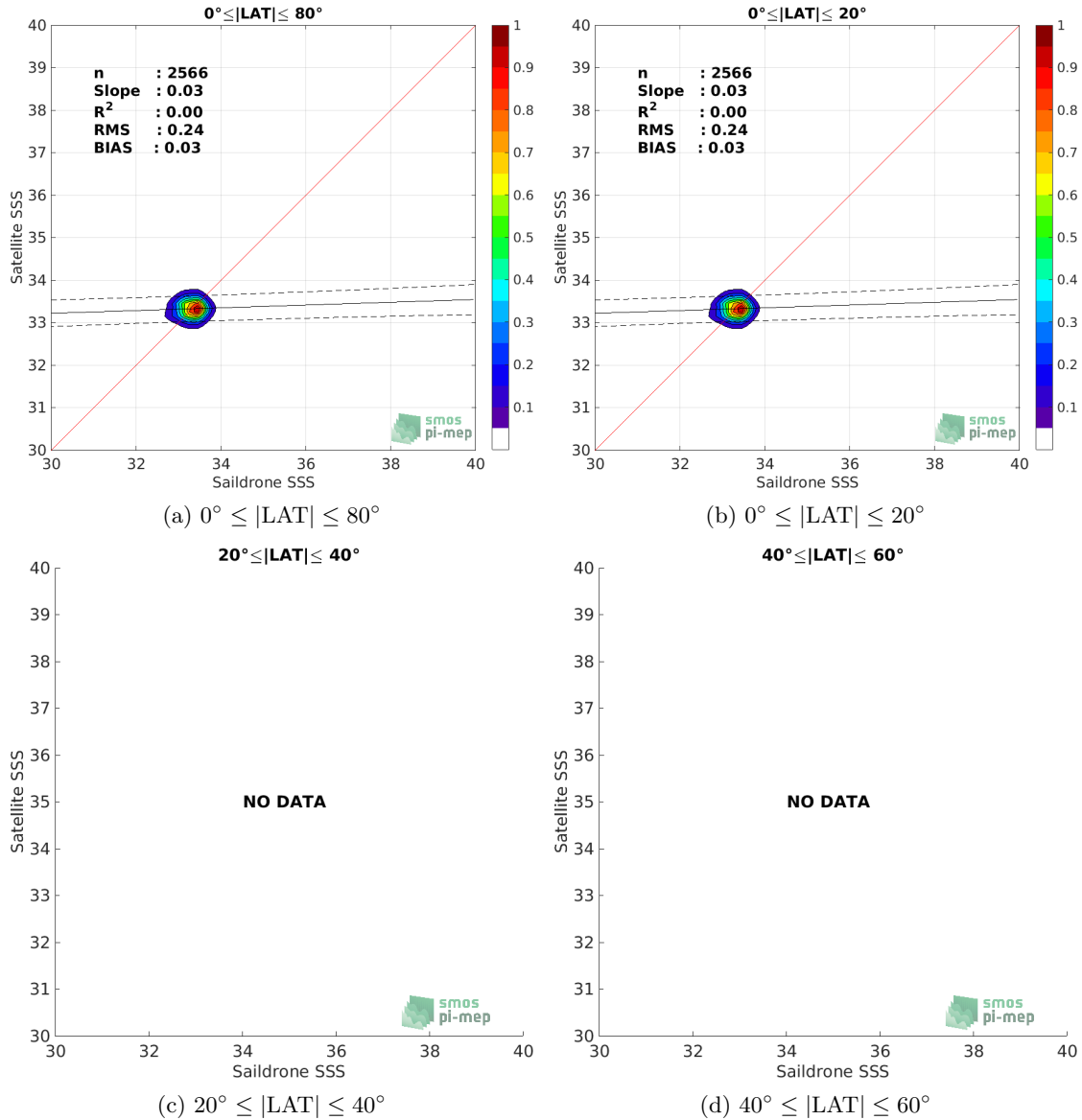
Figure 9: Contour maps of the concentration of SMOS L4 v2 Weekly (CATDS-CECOS-IFREMER) SSS (y-axis) versus Saildrone SSS (x-axis) at match-up pairs for different latitude bands. For each plot, the red line shows x=y . The black thin and dashed lines indicate a linear fit through the data cloud and the \pm 95\% confidence levels, respectively. The number match-up pairs n , the slope and R^2 coefficient of the linear fit, the root mean square (RMS) and the mean bias between satellite and in situ data are indicated for each latitude band in each plots.
