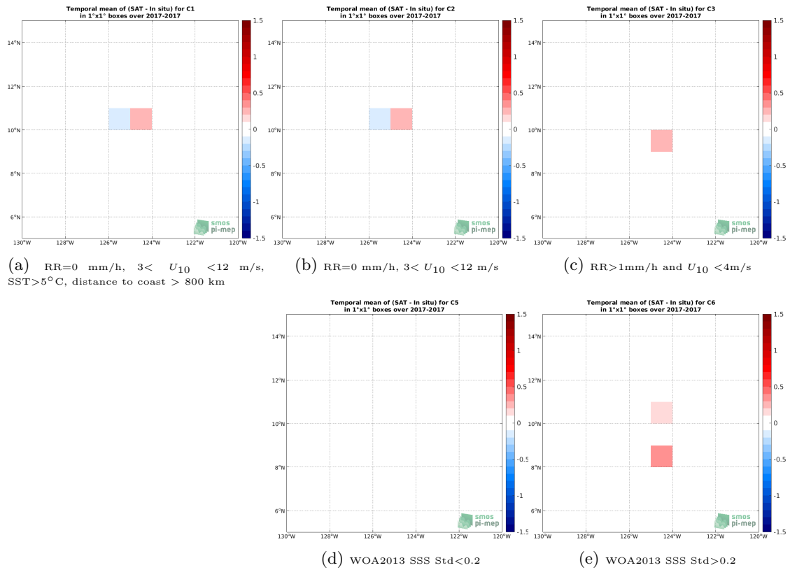
Figure 12: Temporal mean gridded over spatial boxes of size 1^\circ \times 1^\circ of \Delta SSS (SMOS L4 v2 Weekly (CATDS-CECOS-IFREMER) - Saildrone) for 5 different subdatasets corresponding to:RR=0 mm/h, 3 < U_{10} < 12 m/s, SST >5^\circ\text{C} , distance to coast > 800 km (a), RR=0 mm/h, 3 < U_{10} < 12 m/s (b), RR >1 mm/h and U_{10} < 4 m/s (c), WOA2013 SSS Std <0.2 (d), WOA2013 SSS Std >0.2 (e).
