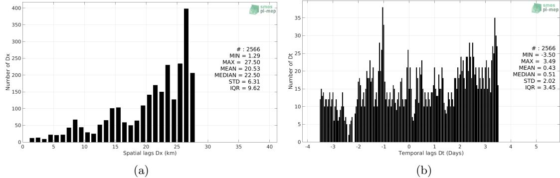
Figure 5: Histograms of the spatial (a) and temporal (b) lags between the time of the Sail-drone measurements and the date of the corresponding SMOS L4 v2 Weekly (CATDS-CECOS-IFREMER) SSS product.
