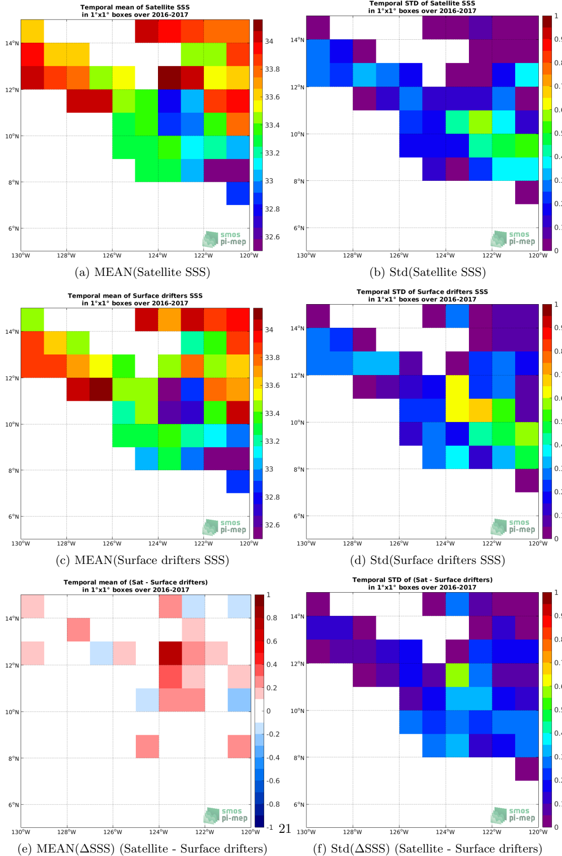
Figure 5: Temporal mean (left) and Std (right) of SSS from SMOS L4 v2 Weekly (CATDS-CECOS-IFREMER) (top), Surface drifters (middle), and of \Delta SSS (Satellite - Surface drifters). Only match-up pairs are used to generate these maps.
