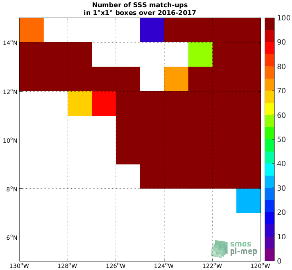
Figure 3: Number of SSS match-ups between Surface drifters SSS and the SMOS L4 v2 Weekly (CATDS-CECOS-IFREMER) SSS product for the SPURS 2 Pi-MEP region over 1°x1° boxes and for the full satellite product period.
