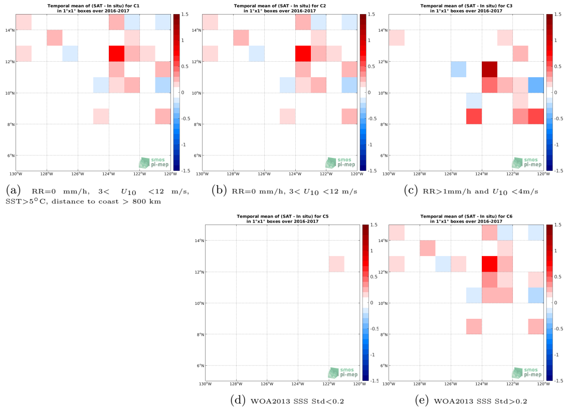
Figure 11: Temporal mean gridded over spatial boxes of size 1^{\circ}\times 1^{\circ} of \Delta\text{SSS} (SMOS L4 v2 Weekly (CATDS-CECOS-IFREMER) - Surface drifters) for 5 different subdatasets corresponding to: \text{RR}=0 mm/h, 3 < U_{10} < 12 m/s, \text{SST} > 5^{\circ}\text{C} , distance to coast > 800 km (a), \text{RR}=0 mm/h, 3 < U_{10} < 12 m/s (b), \text{RR} > 1\text{mm/h} and U_{10} < 4\text{m/s} (c), WOA2013 SSS Std < 0.2 (d), WOA2013 SSS Std > 0.2 (e).
