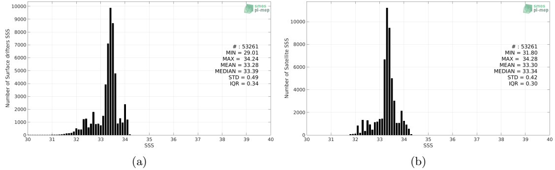
Figure 2: Histograms of SSS from Surface drifters (a) and SMOS L4 v2 Weekly (CATDS-CECOS-IFREMER) (b) considering all match-up pairs per bins of 0.1 over the SPURS 2 Pi-MEP region and for the full satellite product period.
