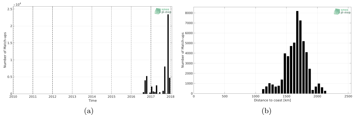
Figure 1: Number of match-ups between Surface drifters and SMOS L4 v2 Weekly (CATDS-CECOS-IFREMER) SSS as a function of time (a) and as function of the distance to coast (b) over the SPURS 2 Pi-MEP region and for the full satellite product period.
