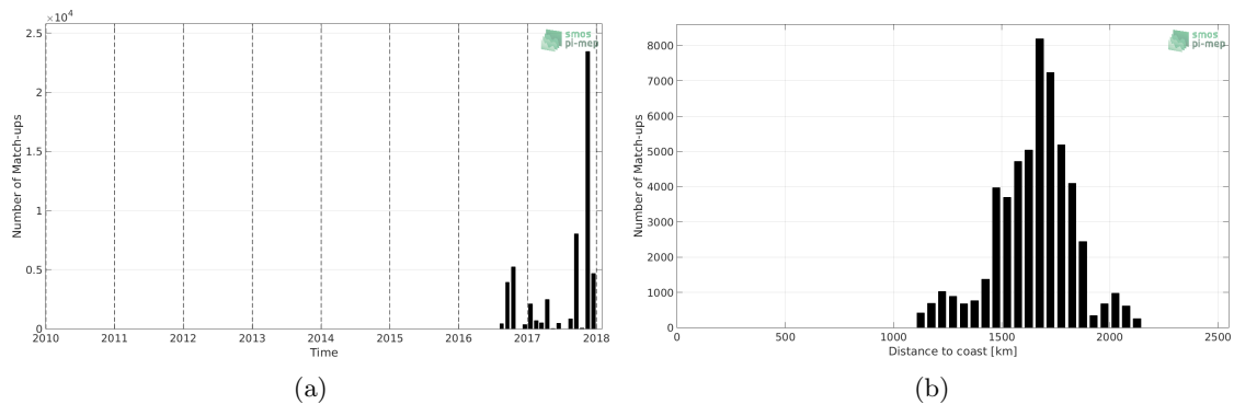
Figure 1: Number of match-ups between Surface drifters and SMOS-L4-CATDS-CECOS-IFREMER-V2-WEEKLY-0.5DEG SSS as a function of time (a) and as function of the distance to coast (b) over the SPURS 2 Pi-MEP region and for the full satellite product period.
