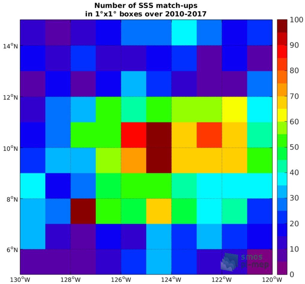
Figure 4: Number of SSS match-ups between Argo SSS and the SMOS-L4-CATDS-CECOS-IFREMER-V2-WEEKLY-0.5DEG SSS product for the SPURS 2 Pi-MEP region over 1°x1° boxes and for the full satellite product period.
