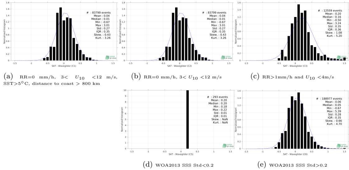
Figure 12: Normalized histogram of \Delta SSS (SMOS SSS L3 v3 Monthly (ICDC) - Waveglider) for 5 different subdatasets corresponding to: RR=0 mm/h, 3 < U_{10} < 12 m/s, SST > 5°C, distance to coast > 800 km (a), RR=0 mm/h, 3 < U_{10} < 12 m/s (b), RR > 1mm/h and U_{10} < 4 m/s (c), WOA2013 SSS Std < 0.2 (d), WOA2013 SSS Std > 0.2 (e).
