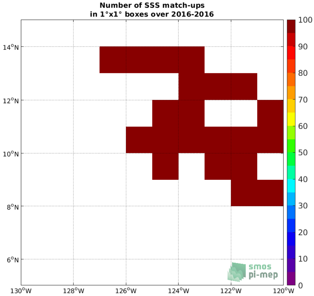
Figure 3: Number of SSS match-ups between Waveglider SSS and the SMOS SSS L3 v3 Monthly (ICDC) SSS product for the SPURS 2 Pi-MEP region over 1^\circ \times 1^\circ boxes and for the full satellite product period.
