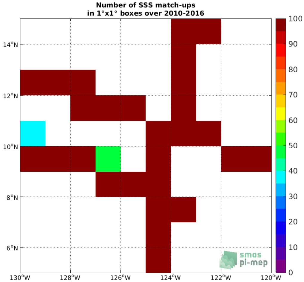
Figure 4: Number of SSS match-ups between TSG (SAMOS) SSS and the SMOS SSS L3 v3 Monthly (ICDC) SSS product for the SPURS 2 Pi-MEP region over 1°x1° boxes and for the full satellite product period.
