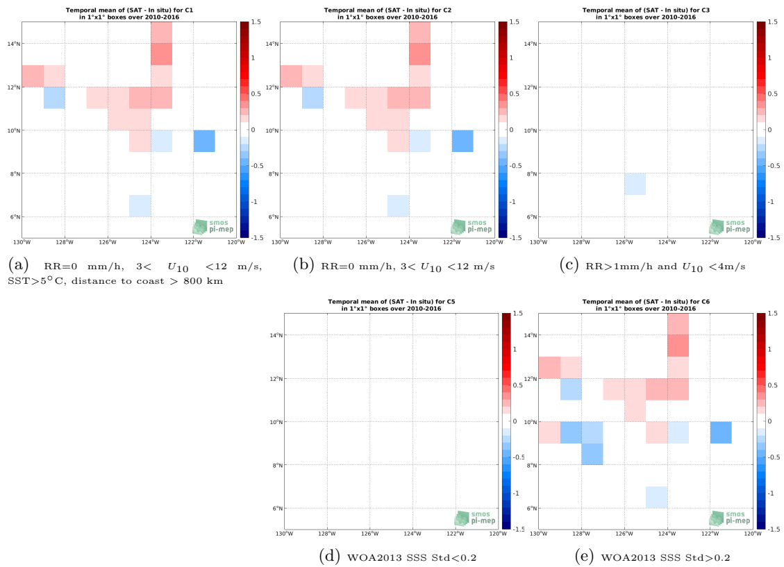
Figure 12: Temporal mean gridded over spatial boxes of size 1^\circ \times 1^\circ of \Delta SSS (SMOS SSS L3 v3 Monthly (ICDC) - TSG (SAMOS)) for 5 different subdatasets corresponding to: RR=0 mm/h, 3 < U_{10} < 12 m/s, SST > 5^\circ C , distance to coast > 800 km (a), RR=0 mm/h, 3 < U_{10} < 12 m/s (b), RR > 1 mm/h and U_{10} < 4 m/s (c), WOA2013 SSS Std < 0.2 (d), WOA2013 SSS Std > 0.2 (e).
