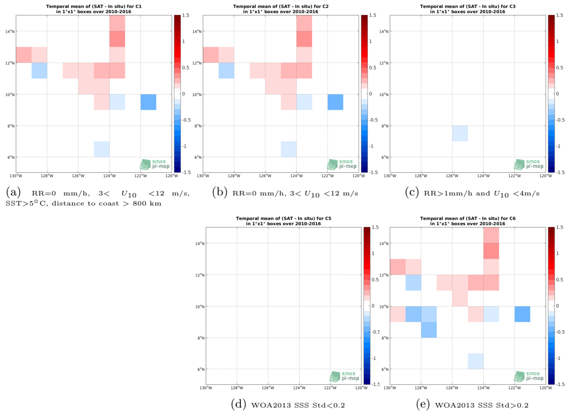
Figure 12: Temporal mean gridded over spatial boxes of size 1^\circ \times 1^\circ of \Delta\text{SSS} (SMOS-L3-ICDC-V3-MONTHLY-0.5DEG - TSG-SAMOS) for 5 different subdatasets corresponding to: \text{RR}=0 mm/h, 3 < U_{10} < 12 m/s, \text{SST} > 5^\circ\text{C} , distance to coast > 800 km (a), \text{RR}=0 mm/h, 3 < U_{10} < 12 m/s (b), \text{RR} > 1\text{mm/h} and U_{10} < 4\text{m/s} (c), WOA2013 SSS Std < 0.2 (d), WOA2013 SSS Std > 0.2 (e).
