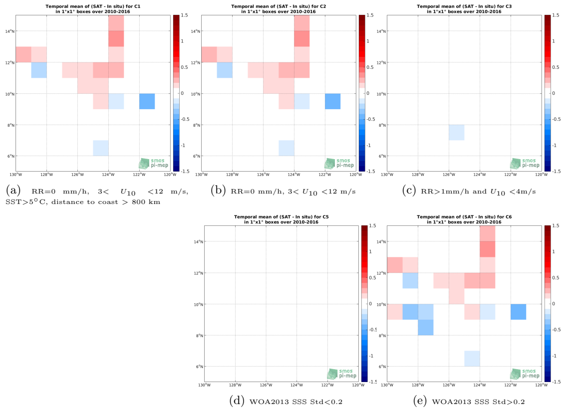
Figure 12: Temporal mean gridded over spatial boxes of size 1^\circ \times 1^\circ of \Delta SSS (SMOS-L3-ICDC-V3-MONTHLY-0.5DEG - TSG-SAMOS) for 5 different subdatasets corresponding to:RR=0 mm/h, 3 < U_{10} < 12 m/s, SST >5^\circ\text{C} , distance to coast > 800 km (a), RR=0 mm/h, 3 < U_{10} < 12 m/s (b), RR >1 mm/h and U_{10} < 4 m/s (c), WOA2013 SSS Std <0.2 (d), WOA2013 SSS Std >0.2 (e).
