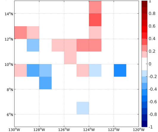
(e) MEAN( \Delta SSS) (Satellite - TSG-SAMOS)
