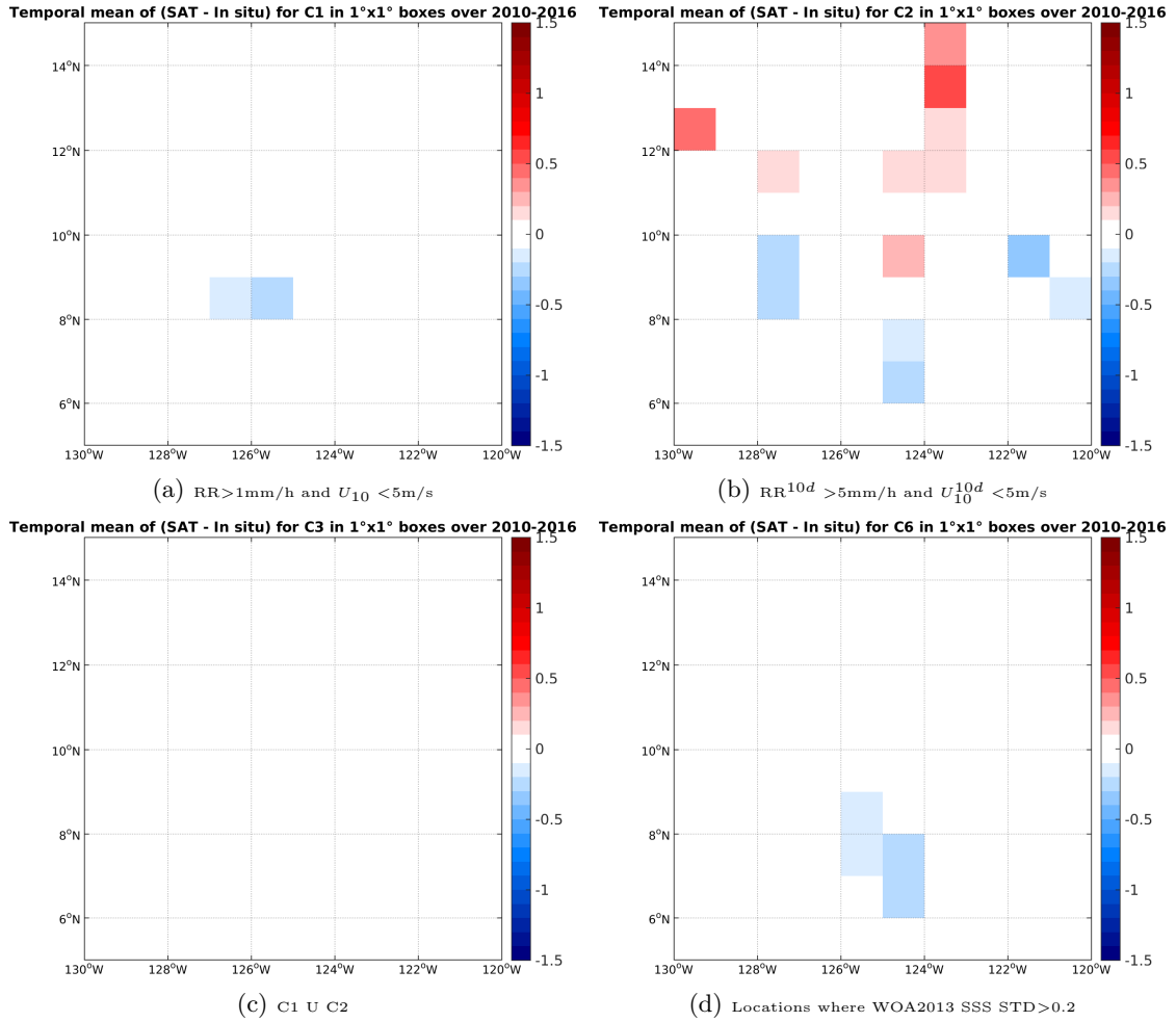
Figure 12: Temporal mean gridded over spatial boxes of size 1°x1° of \Delta SSS (SMOS-L3-ICDC-V3-MONTHLY-0.5DEG - TSG-SAMOS) for 4 different subdatasets corresponding to:RR>1mm/h and U_{10} < 5m/s (a), RR^{10d} > 5mm/h and U_{10}^{10d} < 5m/s (b), C1 U C2 (c),Locations where WOA2013 SSS STD>0.2 (d).
