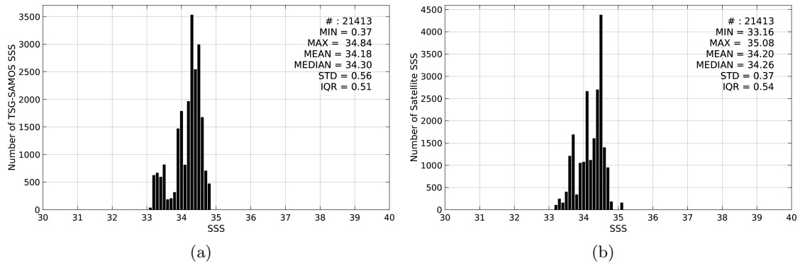
Figure 2: Histograms of SSS from TSG-SAMOS (a) and SMOS-L3-ICDC-V3-MONTHLY-0.5DEG (b) considering all match-up pairs per bins of 0.1 over the SPURS 2 Pi-MEP region and for the full satellite product period.
