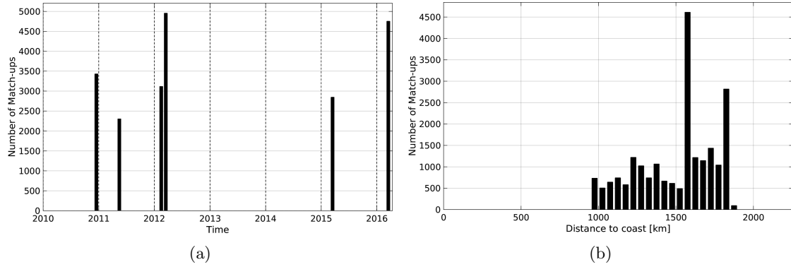
Figure 1: Number of match-ups between TSG-SAMOS and SMOS-L3-ICDC-V3-MONTHLY-0.5DEG SSS as a function of time (a) and as function of the distance to coast (b) over the SPURS 2 Pi-MEP region and for the full satellite product period.
