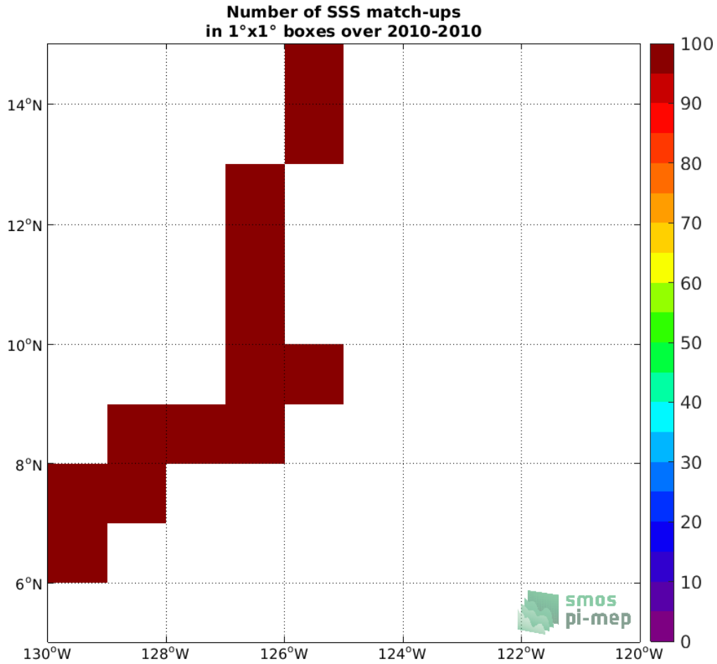
Figure 4: Number of SSS match-ups between TSG (GOSUD-Sailing-ship) SSS and the SMOS SSS L3 v3 Monthly (ICDC) SSS product for the SPURS 2 Pi-MEP region over 1°x1° boxes and for the full satellite product period.
