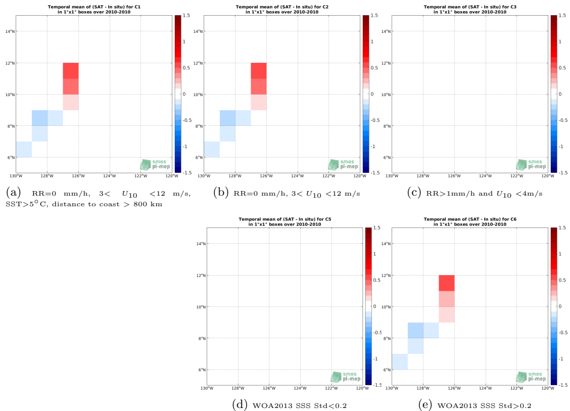
Figure 12: Temporal mean gridded over spatial boxes of size 1^\circ \times 1^\circ of \Delta\text{SSS} (SMOS SSS L3 v3 Monthly (ICDC) - TSG (GOSUD-Sailing-ship)) for 5 different subdatasets corresponding to:RR=0 mm/h, 3 < U_{10} < 12 m/s, SST>5°C, distance to coast > 800 km (a), RR=0 mm/h, 3 < U_{10} < 12 m/s (b), RR>1mm/h and U_{10} < 4 m/s (c), WOA2013 SSS Std<0.2 (d), WOA2013 SSS Std>0.2 (e).
