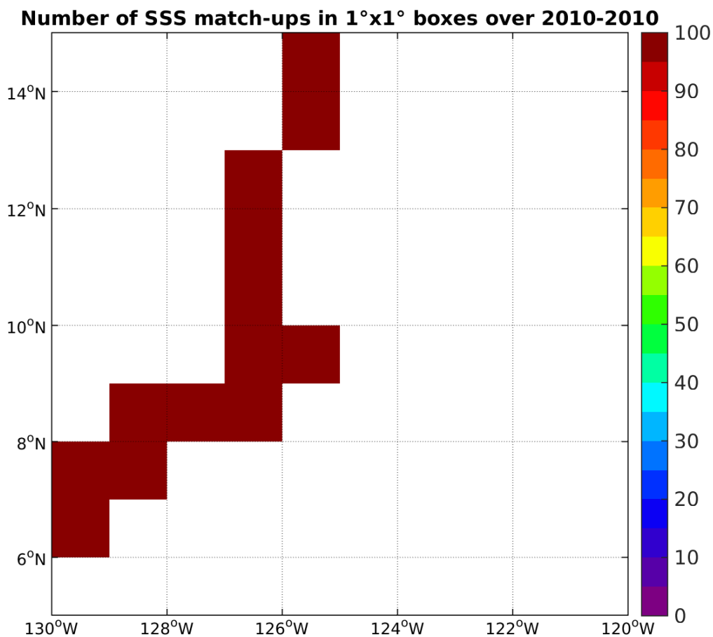
Figure 4: Number of SSS match-ups between TSG-GOSUD-Sailing-ship SSS and the SMOS-L3-ICDC-V3-MONTHLY-0.5DEG SSS product for the SPURS 2 Pi-MEP region over 1°x1° boxes and for the full satellite product period.
