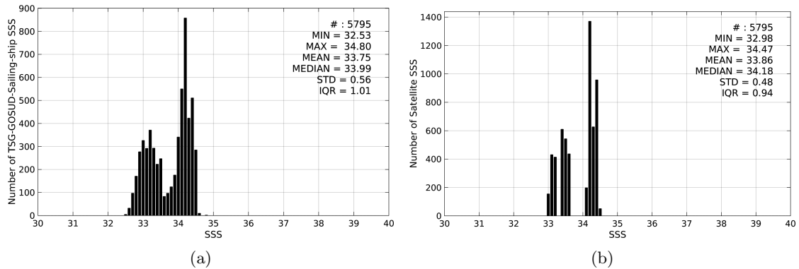
Figure 2: Histograms of SSS from TSG-GOSUD-Sailing-ship (a) and SMOS-L3-ICDC-V3-MONTHLY-0.5DEG (b) considering all match-up pairs per bins of 0.1 over the SPURS 2 Pi-MEP region and for the full satellite product period.
