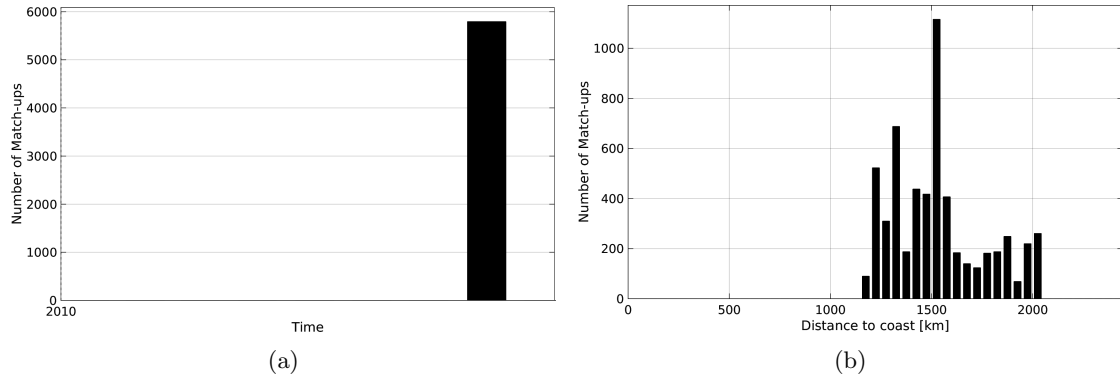
Figure 1: Number of match-ups between TSG-GOSUD-Sailing-ship and SMOS-L3-ICDC-V3-MONTHLY-0.5DEG SSS as a function of time (a) and as function of the distance to coast (b) over the SPURS 2 Pi-MEP region and for the full satellite product period.
