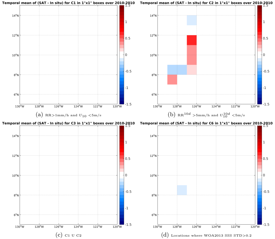
Figure 12: Temporal mean gridded over spatial boxes of size 1°x1° of \Delta SSS (SMOS-L3-ICDC-V3-MONTHLY-0.5DEG - TSG-GOSUD-Sailing-ship) for 4 different subdatasets corresponding to:RR>1mm/h and U_{10} < 5m/s (a), RR^{10d} > 5mm/h and U_{10}^{10d} < 5m/s (b), C1 U C2 (c),Locations where WOA2013 SSS STD>0.2 (d).
