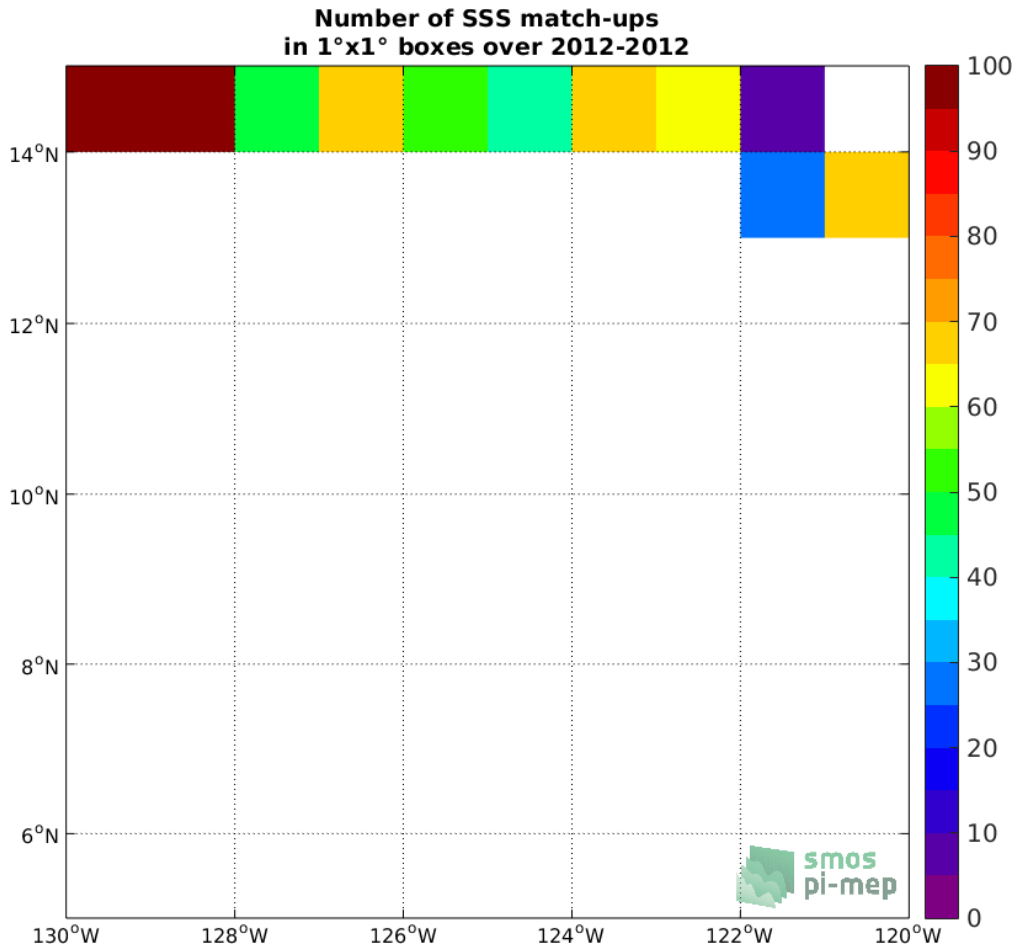
Figure 4: Number of SSS match-ups between TSG-GOSUD-Research-vessel SSS and the SMOS-L3-ICDC-V3-MONTHLY-0.5DEG SSS product for the SPURS 2 Pi-MEP region over 1°x1° boxes and for the full satellite product period.
