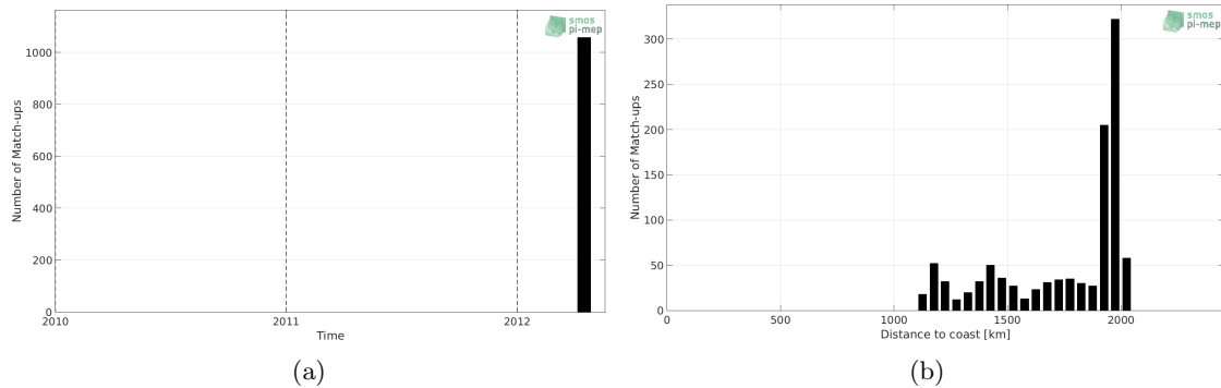
Figure 1: Number of match-ups between TSG-GOSUD-Research-vessel and SMOS-L3-ICDC-V3-MONTHLY-0.5DEG SSS as a function of time (a) and as function of the distance to coast (b) over the SPURS 2 Pi-MEP region and for the full satellite product period.
