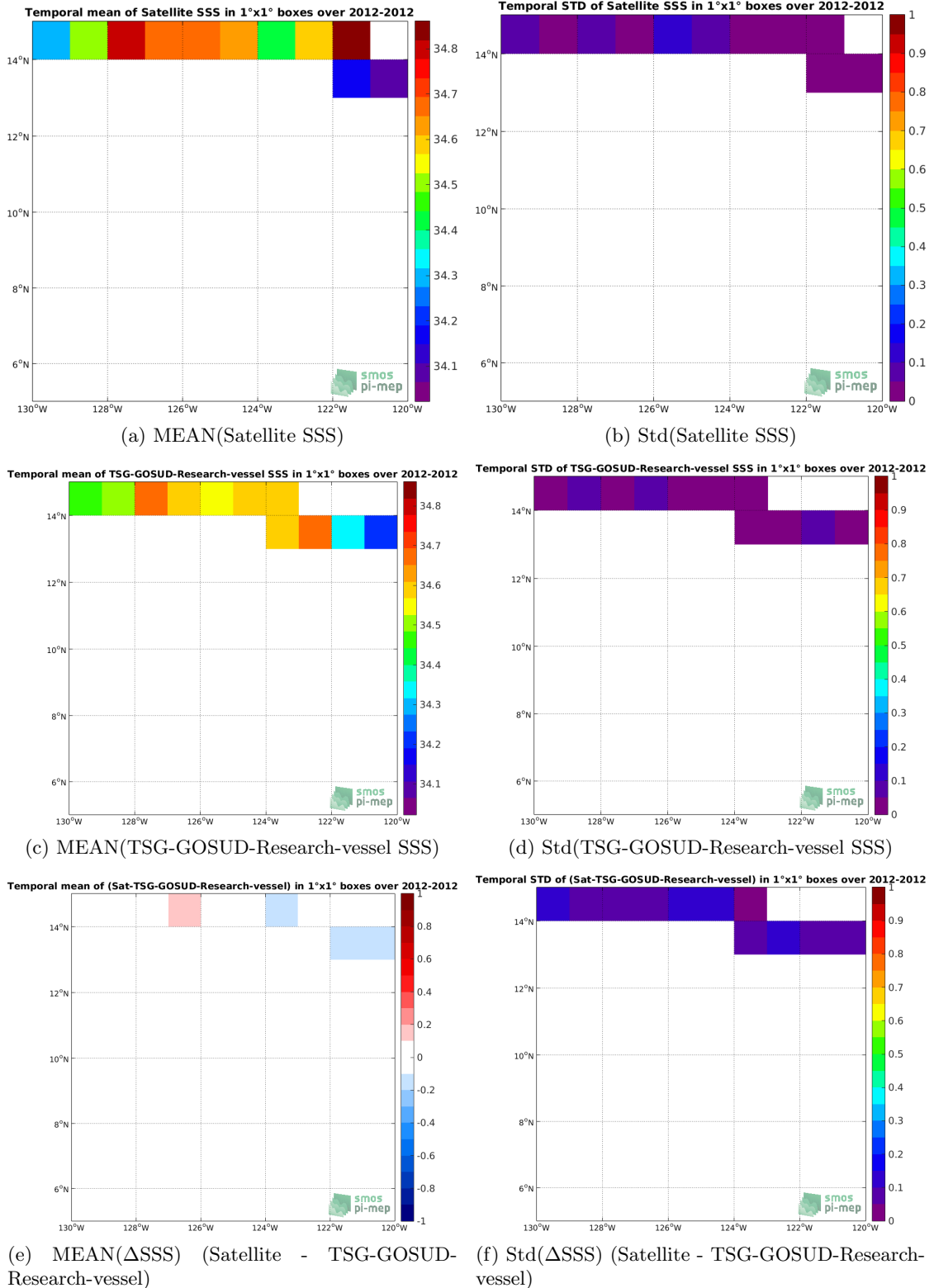
Figure 6: Temporal mean (left) and Std (right) of SSS from SMOS-L3-ICDC-V3-MONTHLY-0.5DEG (top), TSG-GOSUD-Research-vessel (middle), and of \Delta SSS (Satellite - TSG-GOSUD-Research-vessel). Only match-up pairs are used to generate these maps.
