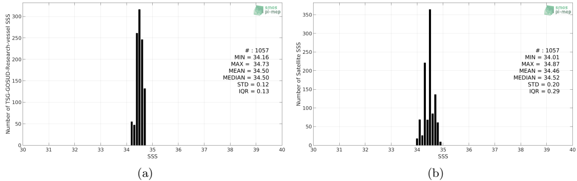
Figure 2: Histograms of SSS from TSG-GOSUD-Research-vessel (a) and SMOS-L3-ICDC-V3-MONTHLY-0.5DEG (b) considering all match-up pairs per bins of 0.1 over the SPURS 2 Pi-MEP region and for the full satellite product period.
