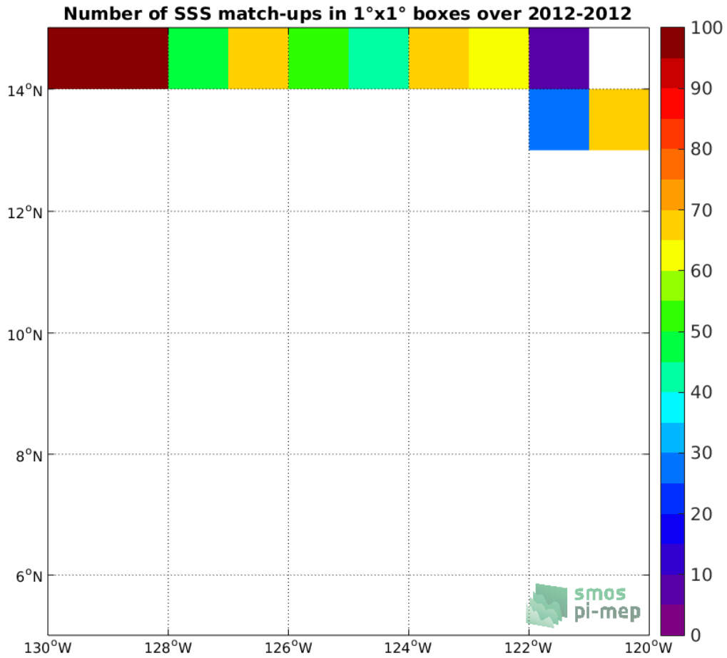
Figure 4: Number of SSS match-ups between TSG-GOSUD-Research-vessel SSS and the SMOS-L3-ICDC-V3-MONTHLY-0.5DEG SSS product for the SPURS 2 Pi-MEP region over 1°x1° boxes and for the full satellite product period.
