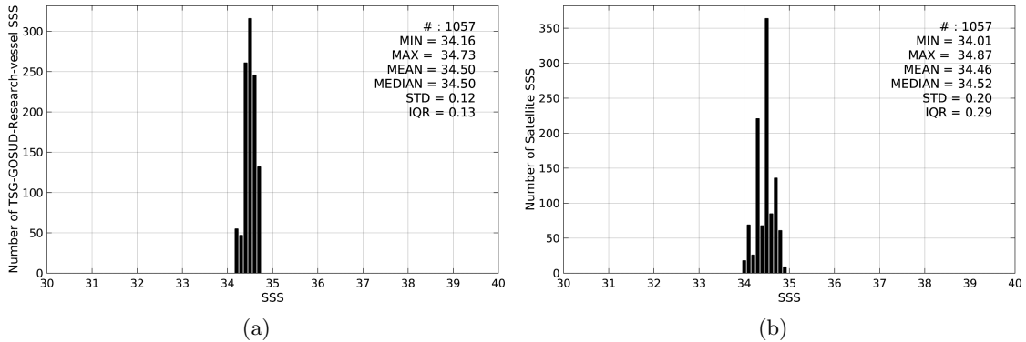
Figure 2: Histograms of SSS from TSG-GOSUD-Research-vessel (a) and SMOS-L3-ICDC-V3-MONTHLY-0.5DEG (b) considering all match-up pairs per bins of 0.1 over the SPURS 2 Pi-MEP region and for the full satellite product period.
