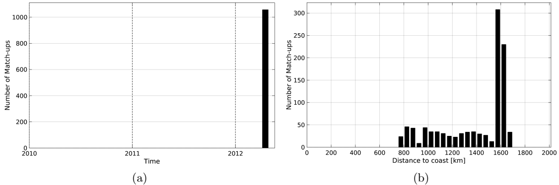
Figure 1: Number of match-ups between TSG-GOSUD-Research-vessel and SMOS-L3-ICDC-V3-MONTHLY-0.5DEG SSS as a function of time (a) and as function of the distance to coast (b) over the SPURS 2 Pi-MEP region and for the full satellite product period.
