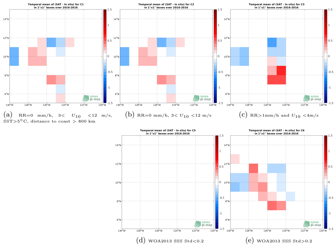
Figure 11: Temporal mean gridded over spatial boxes of size 1^\circ \times 1^\circ of \Delta SSS (SMOS SSS L3 v3 Monthly (ICDC) - Salinity Snake) for 5 different subdatasets corresponding to:RR=0 mm/h, 3 < U_{10} < 12 m/s, SST >5^\circ C, distance to coast > 800 km (a), RR=0 mm/h, 3 < U_{10} < 12 m/s (b), RR >1 mm/h and U_{10} < 4 m/s (c), WOA2013 SSS Std <0.2 (d), WOA2013 SSS Std >0.2 (e).
