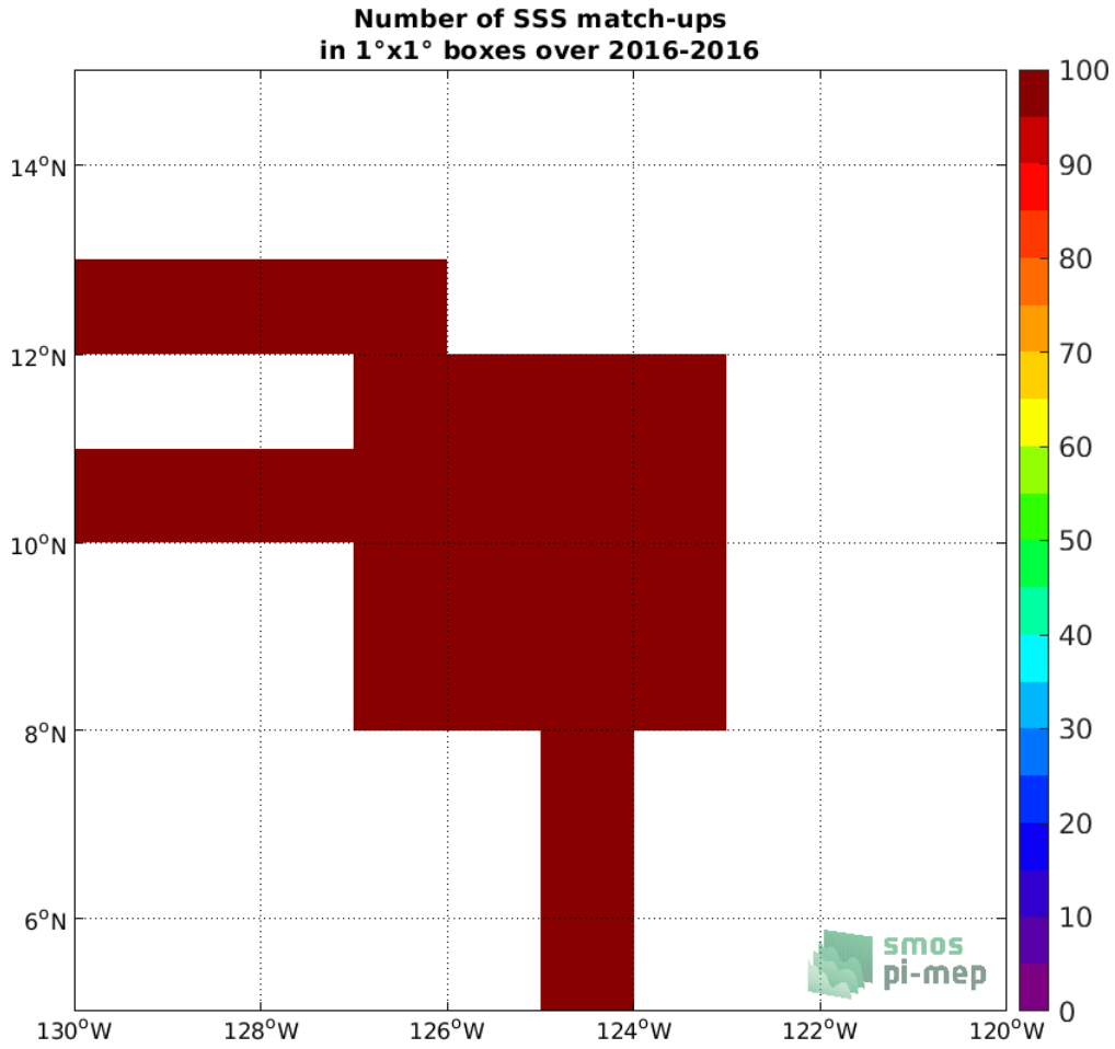
Figure 3: Number of SSS match-ups between Salinity Snake SSS and the SMOS SSS L3 v3 Monthly (ICDC) SSS product for the SPURS 2 Pi-MEP region over 1°×1° boxes and for the full satellite product period.
