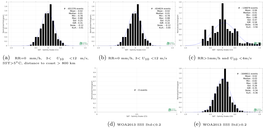
Figure 12: Normalized histogram of \Delta SSS (SMOS SSS L3 v3 Monthly (ICDC) - Salinity Snake) for 5 different subdatasets corresponding to: RR=0 mm/h, 3 < U_{10} < 12 m/s, SST > 5°C, distance to coast > 800 km (a), RR=0 mm/h, 3 < U_{10} < 12 m/s (b), RR > 1mm/h and U_{10} < 4 m/s (c), WOA2013 SSS Std < 0.2 (d), WOA2013 SSS Std > 0.2 (e).
