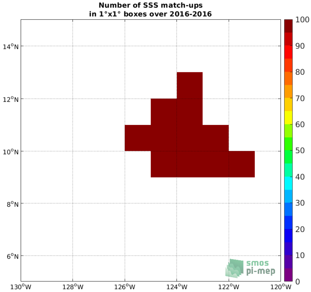
Figure 3: Number of SSS match-ups between Seagliders SSS and the SMOS SSS L3 v3 Monthly (ICDC) SSS product for the SPURS 2 Pi-MEP region over 1°×1° boxes and for the full satellite product period.
