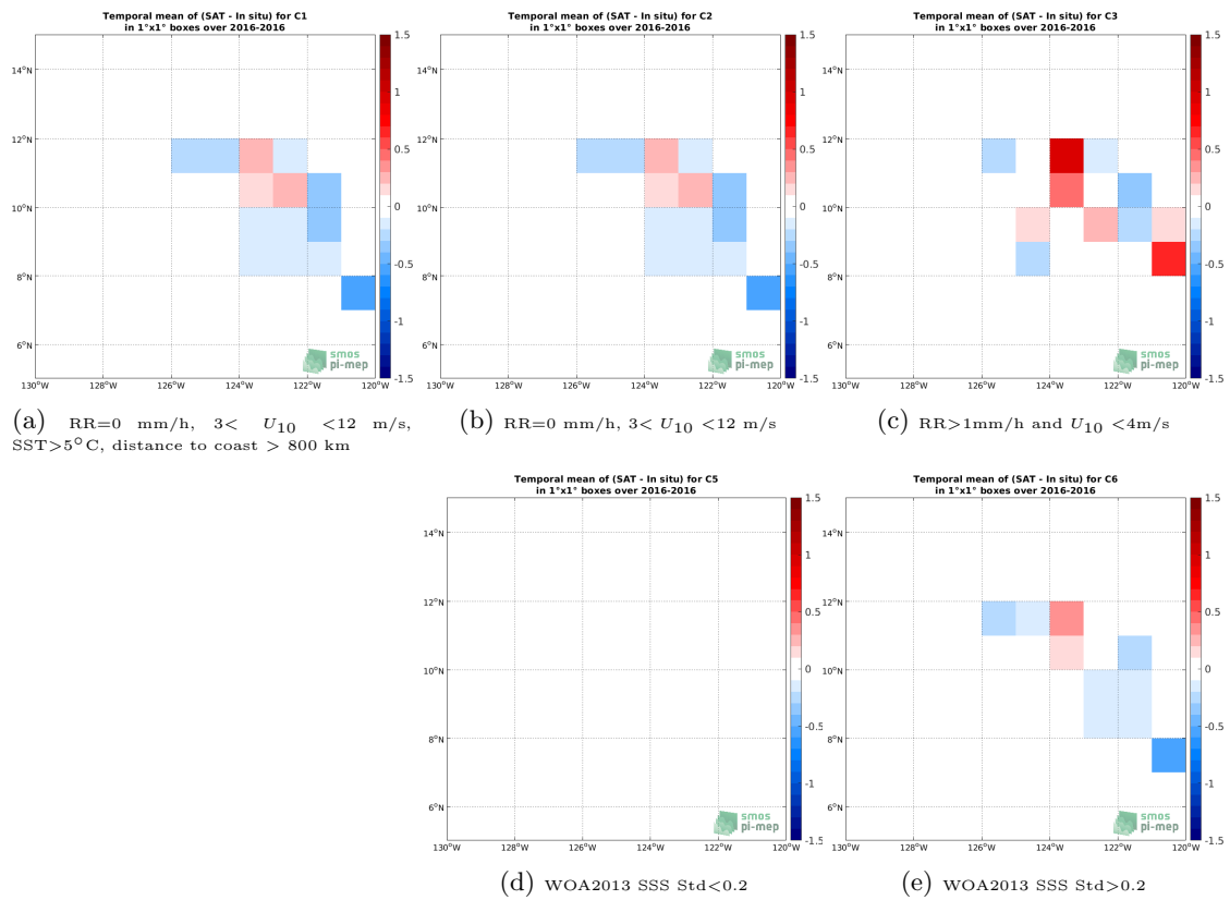
Figure 11: Temporal mean gridded over spatial boxes of size 1^\circ \times 1^\circ of \Delta SSS (SMOS SSS L3 v3 Monthly (ICDC) - Surface drifters) for 5 different subdatasets corresponding to:RR=0 mm/h, 3 < U_{10} < 12 m/s, SST >5^\circ\text{C} , distance to coast > 800 km (a), RR=0 mm/h, 3 < U_{10} < 12 m/s (b), RR >1 mm/h and U_{10} < 4 m/s (c), WOA2013 SSS Std <0.2 (d), WOA2013 SSS Std >0.2 (e).
