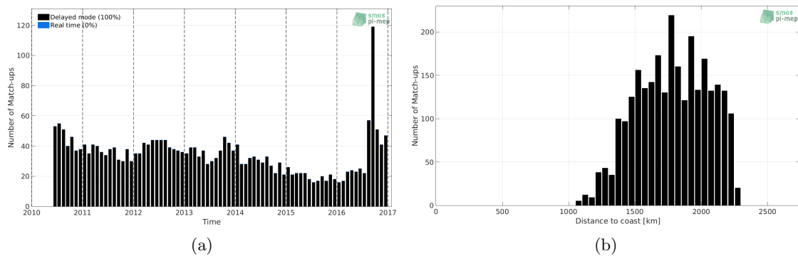
Figure 1: Number of match-ups between Argo and SMOS SSS L3 v3 Monthly (ICDC) SSS as a function of time (a) and as function of the distance to coast (b) over the SPURS 2 Pi-MEP region and for the full satellite product period.
