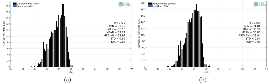
Figure 2: Histograms of SSS from Argo (a) and SMOS SSS L3 v3 Monthly (ICDC) (b) considering all match-up pairs per bins of 0.1 over the SPURS 2 Pi-MEP region and for the full satellite product period.
