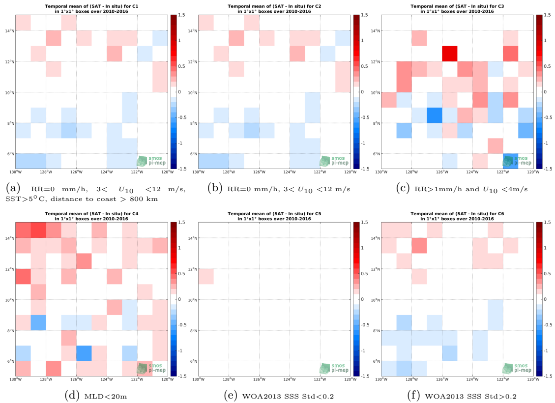
Figure 12: Temporal mean gridded over spatial boxes of size 1^\circ \times 1^\circ of \Delta SSS (SMOS SSS L3 v3 Monthly (ICDC) - Argo) for 6 different subdatasets corresponding to:RR=0 mm/h, 3 < U_{10} < 12 m/s, SST >5^\circ C, distance to coast > 800 km (a), RR=0 mm/h, 3 < U_{10} < 12 m/s (b), RR >1 mm/h and U_{10} < 4 m/s (c),MLD <20 m (d),WOA2013 SSS Std <0.2 (e),WOA2013 SSS Std >0.2 (f).
