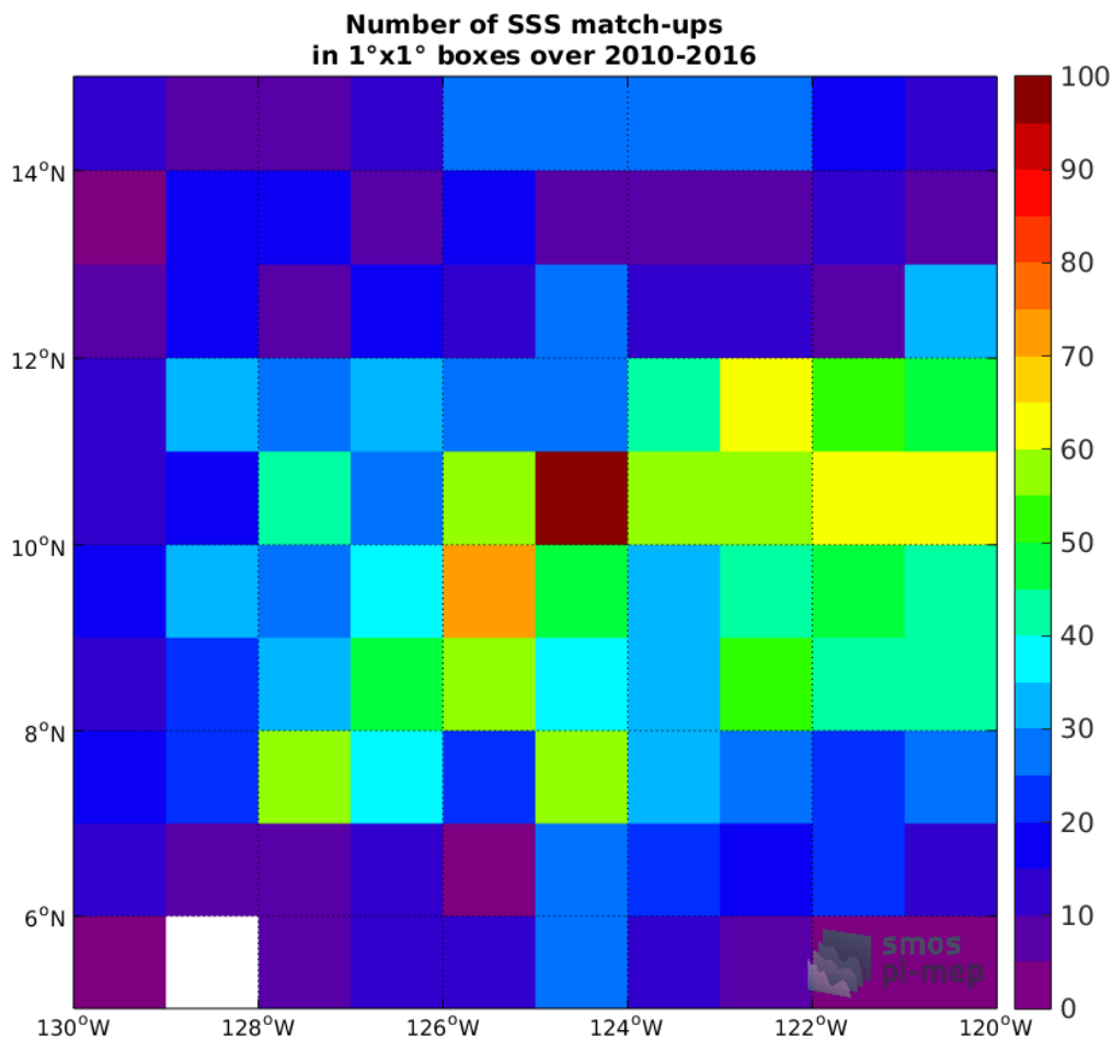
Figure 4: Number of SSS match-ups between Argo SSS and the SMOS SSS L3 v3 Monthly (ICDC) SSS product for the SPURS 2 Pi-MEP region over 1^\circ \times 1^\circ boxes and for the full satellite product period.
