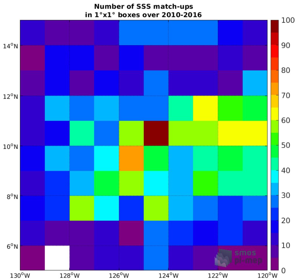
Figure 4: Number of SSS match-ups between Argo SSS and the SMOS SSS L3 v3 Monthly (ICDC) SSS product for the SPURS 2 Pi-MEP region over 1°x1° boxes and for the full satellite product period.
