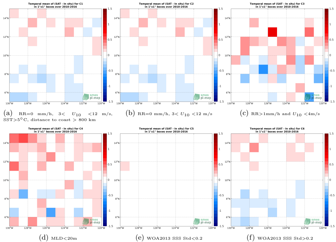
Figure 12: Temporal mean gridded over spatial boxes of size 1^\circ \times 1^\circ of \Delta SSS (SMOS SSS L3 v3 Monthly (ICDC) - Argo) for 6 different subdatasets corresponding to:RR=0 mm/h, 3 < U_{10} < 12 m/s, SST >5^\circ C, distance to coast > 800 km (a), RR=0 mm/h, 3 < U_{10} < 12 m/s (b), RR >1 mm/h and U_{10} < 4 m/s (c),MLD <20 m (d),WOA2013 SSS Std <0.2 (e),WOA2013 SSS Std >0.2 (f).
