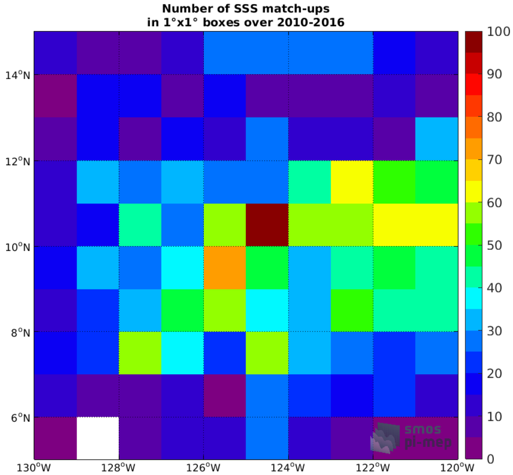
Figure 4: Number of SSS match-ups between Argo SSS and the SMOS SSS L3 v3 Monthly (ICDC) SSS product for the SPURS 2 Pi-MEP region over 1°x1° boxes and for the full satellite product period.
