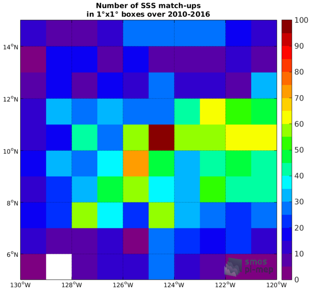
Figure 4: Number of SSS match-ups between Argo SSS and the SMOS-L3-ICDC-V3-MONTHLY-0.5DEG SSS product for the SPURS 2 Pi-MEP region over 1°x1° boxes and for the full satellite product period.
