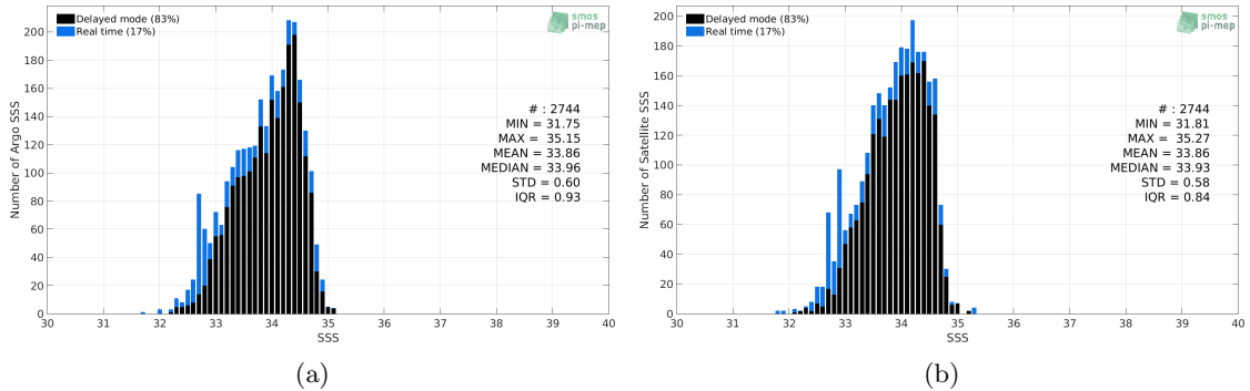
Figure 2: Histograms of SSS from Argo (a) and SMOS-L3-ICDC-V3-MONTHLY-0.5DEG (b) considering all match-up pairs per bins of 0.1 over the SPURS 2 Pi-MEP region and for the full satellite product period.
