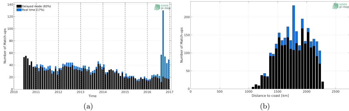
Figure 1: Number of match-ups between Argo and SMOS-L3-ICDC-V3-MONTHLY-0.5DEG SSS as a function of time (a) and as function of the distance to coast (b) over the SPURS 2 Pi-MEP region and for the full satellite product period.
