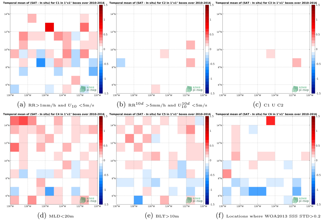
Figure 12: Temporal mean gridded over spatial boxes of size 1^\circ \times 1^\circ of \Delta\text{SSS} (SMOS-L3-ICDC-V3-MONTHLY-0.5DEG - Argo) for 6 different subdatasets corresponding to: RR > 1\text{mm/h} and U_{10} < 5\text{m/s} (a), RR^{10d} > 5\text{mm/h} and U_{10}^{10d} < 5\text{m/s} (b), C1 U C2 (c), MLD < 20\text{m} (d), BLT > 10\text{m} (e), Locations where WOA2013 SSS STD > 0.2 (f).
