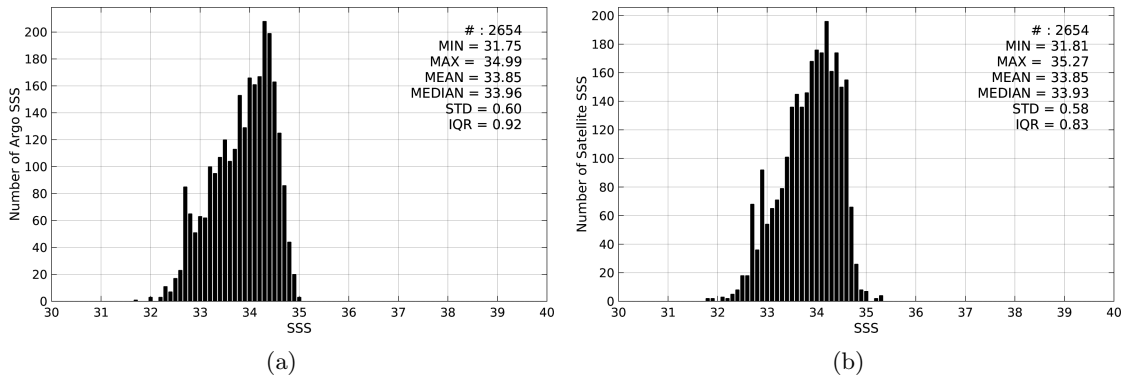
Figure 2: Histograms of SSS from Argo (a) and SMOS-L3-ICDC-V3-MONTHLY-0.5DEG (b) considering all match-up pairs per bins of 0.1 over the SPURS 2 Pi-MEP region and for the full satellite product period.
