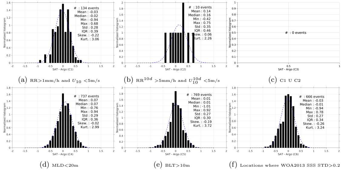
Figure 13: Normalized histogram of \Delta SSS (SMOS-L3-ICDC-V3-MONTHLY-0.5DEG - Argo) for 6 different subdatasets corresponding to: RR>1mm/h and U_{10} < 5\text{m/s} (a), RR^{10d} > 5\text{mm/h} and U_{10}^{10d} < 5\text{m/s} (b), C1 U C2 (c),MLD<20m (d),BLT>10m (e),Locations where WOA2013 SSS STD>0.2 (f).
