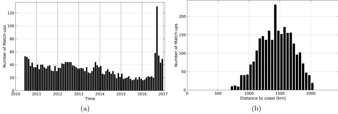
Figure 1: Number of match-ups between Argo and SMOS-L3-ICDC-V3-MONTHLY-0.5DEG SSS as a function of time (a) and as function of the distance to coast (b) over the SPURS 2 Pi-MEP region and for the full satellite product period.
