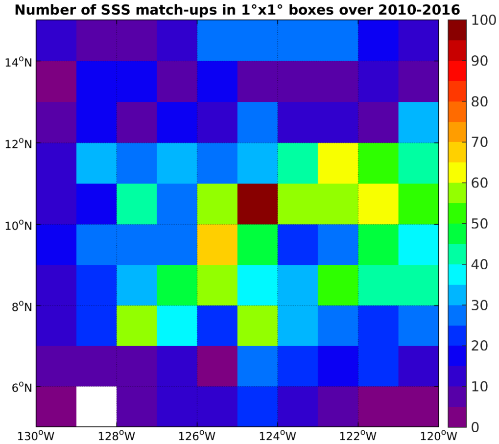
Figure 4: Number of SSS match-ups between Argo SSS and the SMOS-L3-ICDC-V3-MONTHLY-0.5DEG SSS product for the SPURS 2 Pi-MEP region over 1°x1° boxes and for the full satellite product period.
