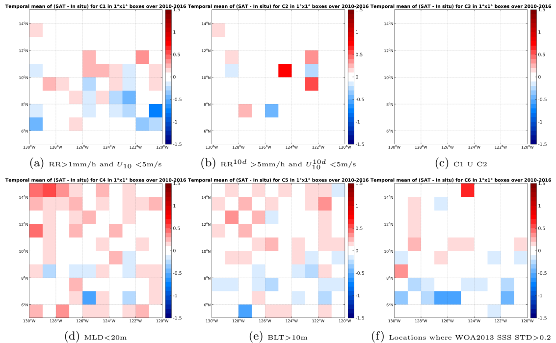
Figure 12: Temporal mean gridded over spatial boxes of size 1^\circ \times 1^\circ of \Delta SSS (SMOS-L3-ICDC-V3-MONTHLY-0.5DEG - Argo) for 6 different subdatasets corresponding to: RR > 1\text{mm/h} and U_{10} < 5\text{m/s} (a), RR^{10d} > 5\text{mm/h} and U_{10}^{10d} < 5\text{m/s} (b), C1 U C2 (c), MLD < 20\text{m} (d), BLT > 10\text{m} (e), Locations where WOA2013 SSS STD > 0.2 (f).
