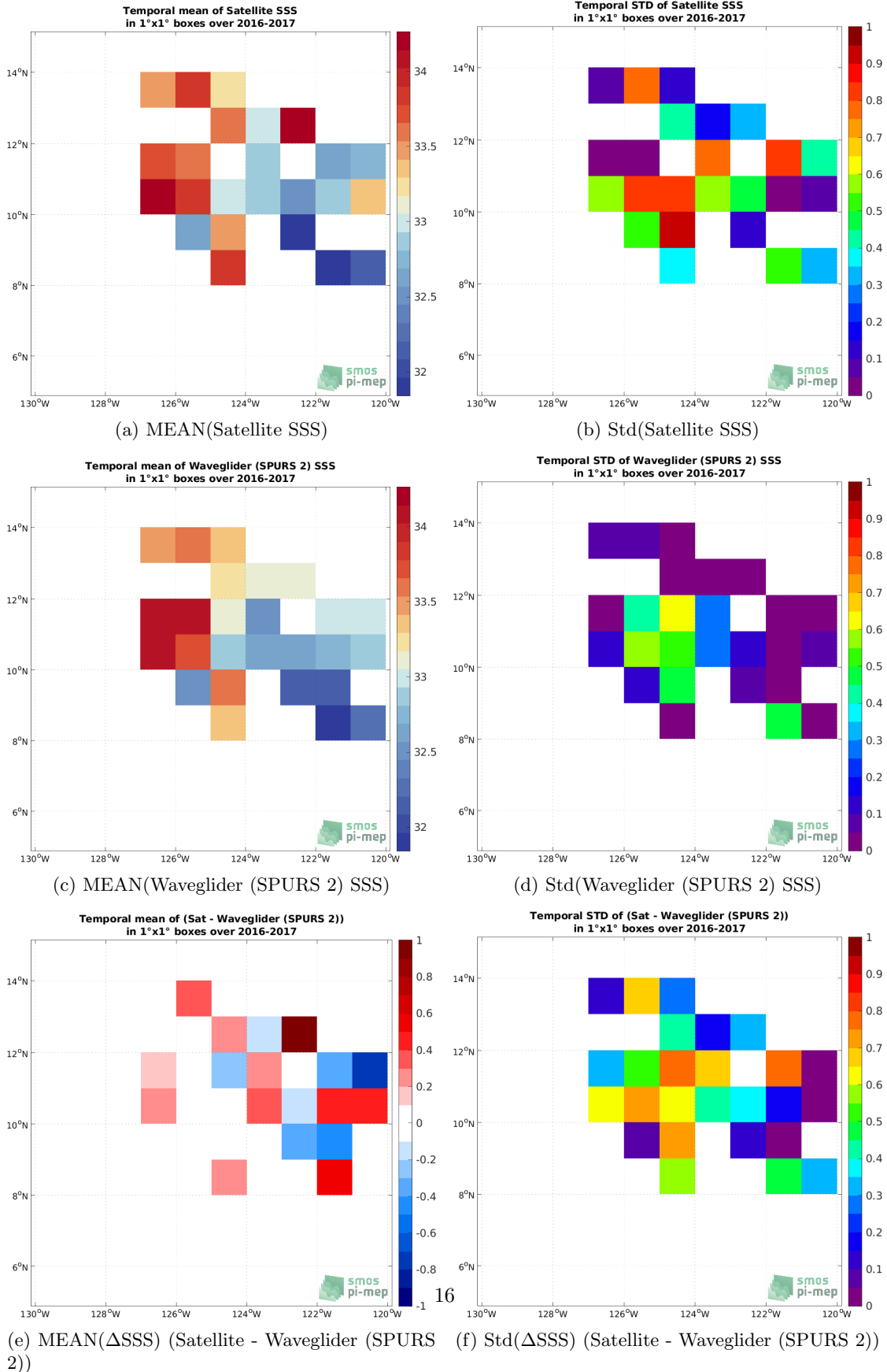
Figure 6: Temporal mean (left) and Std (right) of SSS from SMOS SSS L2Q v331 - With FLAG (CMEMS-CATDS-CPDC) (top), Waveglider (SPURS 2) (middle), and of \Delta SSS (Satellite - Waveglider (SPURS 2)). Only match-up pairs are used to generate these maps.
