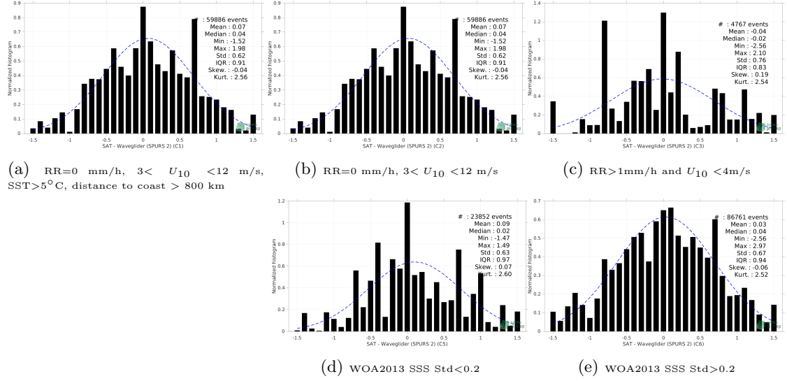
Figure 13: Normalized histogram of \Delta SSS (SMOS SSS L2Q v331 - With FLAG (CMEMS-CATDS-CPDC) - Waveglider (SPURS 2)) for 5 different subdatasets corresponding to: RR=0 mm/h, 3 < U_{10} < 12 m/s, SST>5°C, distance to coast > 800 km (a), RR=0 mm/h, 3 < U_{10} < 12 m/s (b), RR>1mm/h and U_{10} < 4 m/s (c), WOA2013 SSS Std<0.2 (d), WOA2013 SSS Std>0.2 (e).
