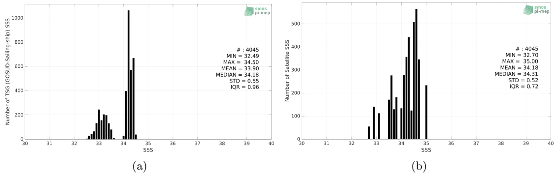
Figure 2: Histograms of SSS from TSG (GOSUD-Sailing-ship) (a) and SMOS SSS L2Q v331 - With FLAG (CMEMS-CATDS-CPDC) (b) considering all match-up pairs per bins of 0.1 over the SPURS 2 Pi-MEP region and for the full satellite product period.
