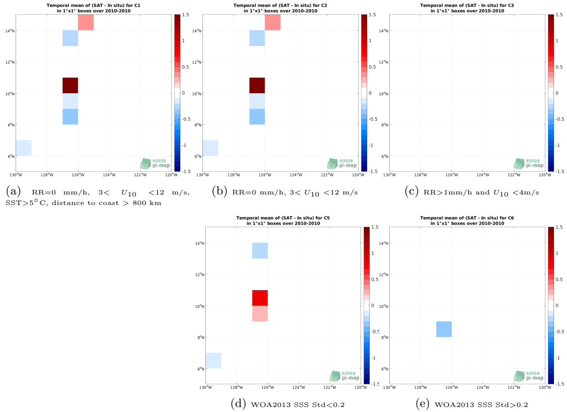
Figure 12: Temporal mean gridded over spatial boxes of size 1^{\circ} \times 1^{\circ} of \Delta\text{SSS} (SMOS SSS L2Q v331 - With FLAG (CMEMS-CATDS-CPDC) - TSG (GOSUD-Sailing-ship)) for 5 different subdatasets corresponding to: RR=0 mm/h, 3 < U_{10} < 12 m/s, SST > 5^{\circ}\text{C} , distance to coast > 800 km (a), RR=0 mm/h, 3 < U_{10} < 12 m/s (b), RR > 1\text{mm/h} and U_{10} < 4\text{m/s} (c), WOA2013 SSS Std < 0.2 (d), WOA2013 SSS Std > 0.2 (e).
