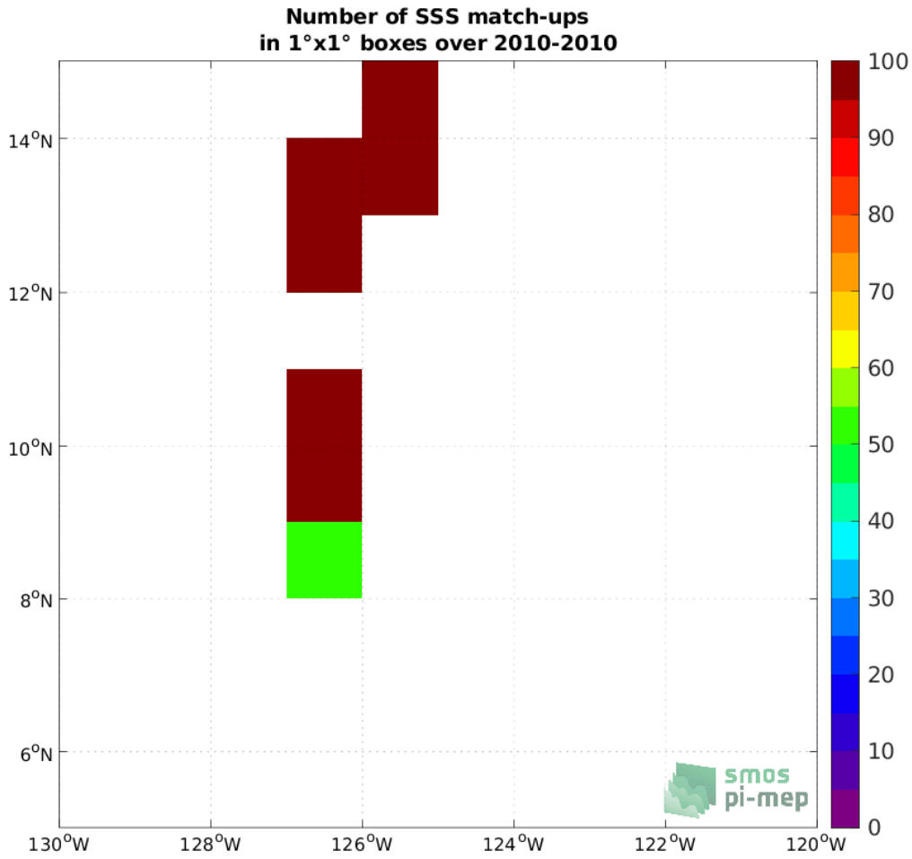
Figure 4: Number of SSS match-ups between TSG (GOSUD-Sailing-ship) SSS and the SMOS SSS L2Q v331 - With FLAG (CMEMS-CATDS-CPDC) SSS product for the SPURS 2 Pi-MEP region over 1^\circ \times 1^\circ boxes and for the full satellite product period.
