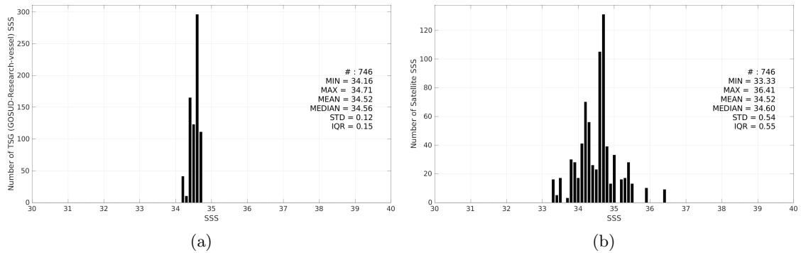
Figure 3: Histograms of SSS from TSG (GOSUD-Research-vessel) (a) and SMOS SSS L2Q v331 - With FLAG (CMEMS-CATDS-CPDC) (b) considering all match-up pairs per bins of 0.1 over the SPURS 2 Pi-MEP region and for the full satellite product period.
