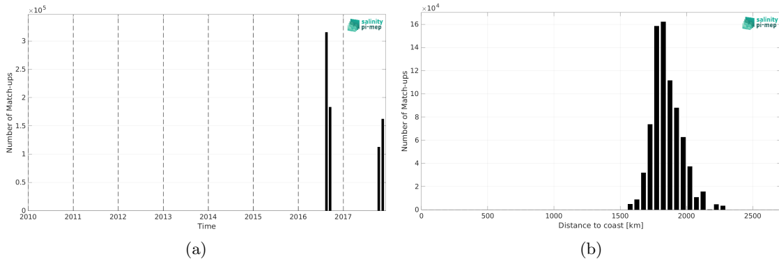
Figure 2: Number of match-ups between Salinity Snake (SPURS 2) and SMOS SSS L2Q v331 - With FLAG (CMEMS-CATDS-CPDC) SSS as a function of time (a) and as function of the distance to coast (b) over the SPURS 2 Pi-MEP region and for the full satellite product period.
