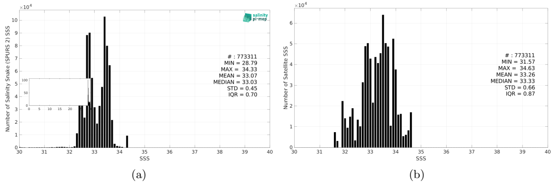
Figure 3: Histograms of SSS from Salinity Snake (SPURS 2) (a) and SMOS SSS L2Q v331 - With FLAG (CMEMS-CATDS-CPDC) (b) considering all match-up pairs per bins of 0.1 over the SPURS 2 Pi-MEP region and for the full satellite product period.
