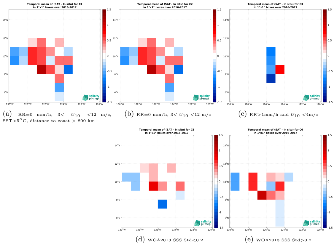
Figure 14: Temporal mean gridded over spatial boxes of size 1^\circ \times 1^\circ of \Delta\text{SSS} (SMOS SSS L2Q v331 - With FLAG (CMEMS-CATDS-CPDC) - Salinity Snake (SPURS 2)) for 5 different sub-datasets corresponding to:RR=0 mm/h, 3 < U_{10} < 12 m/s, SST > 5°C, distance to coast > 800 km (a), RR=0 mm/h, 3 < U_{10} < 12 m/s (b), RR > 1mm/h and U_{10} < 4 m/s (c), WOA2013 SSS Std < 0.2 (d), WOA2013 SSS Std > 0.2 (e).
