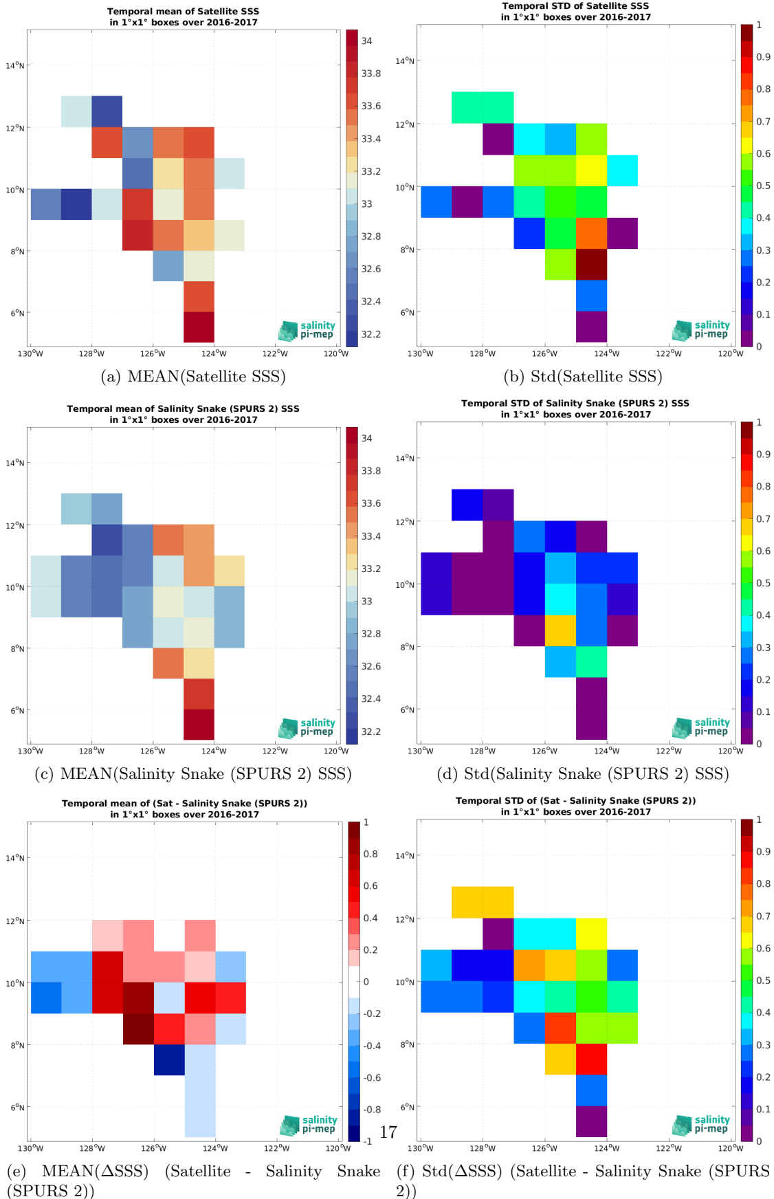
Figure 7: Temporal mean (left) and Std (right) of SSS from SMOS SSS L2Q v331 - With FLAG (CMEMS-CATDS-CPDC) (top), Salinity Snake (SPURS 2) (middle), and of \Delta SSS (Satellite - Salinity Snake (SPURS 2)). Only match-up pairs are used to generate these maps.
