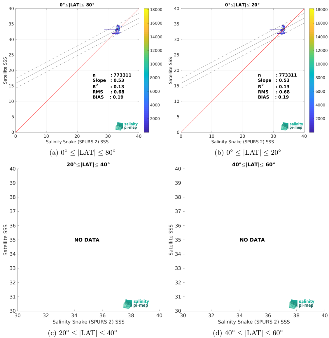
Figure 10: Contour maps of the concentration of SMOS SSS L2Q v331 - With FLAG (CMEMS-CATDS-CPDC) SSS (y-axis) versus Salinity Snake (SPURS 2) SSS (x-axis) at match-up pairs for different latitude bands. For each plot, the red line shows x=y . The black thin and dashed lines indicate a linear fit through the data cloud and the \pm 95\% confidence levels, respectively. The number match-up pairs n , the slope and R^2 coefficient of the linear fit, the root mean square (RMS) and the mean bias between satellite and in situ data are indicated for each latitude band in each plots.
