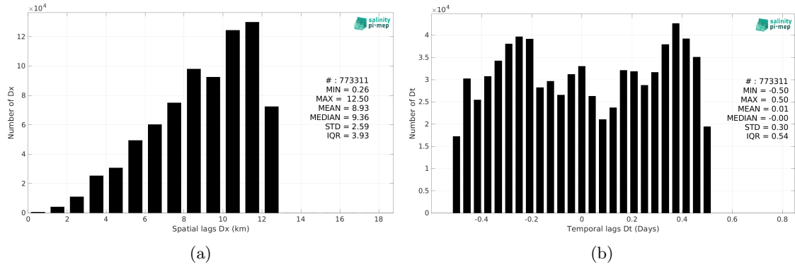
Figure 6: Histograms of the spatial (a) and temporal (b) lags between the location/time of the Salinity Snake (SPURS 2) measurement and the date of the corresponding SMOS SSS L2Q v331 - With FLAG (CMEMS-CATDS-CPDC) SSS pixel.
