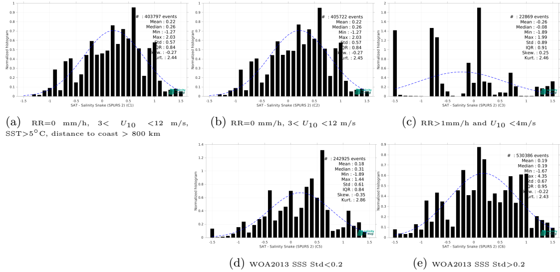
Figure 15: Normalized histogram of \Delta SSS (SMOS SSS L2Q v331 - With FLAG (CMEMS-CATDS-CPDC) - Salinity Snake (SPURS 2)) for 5 different subdatasets corresponding to: RR=0 mm/h, 3 < U_{10} < 12 m/s, SST>5°C, distance to coast > 800 km (a), RR=0 mm/h, 3 < U_{10} < 12 m/s (b), RR>1mm/h and U_{10} < 4 m/s (c), WOA2013 SSS Std<0.2 (d), WOA2013 SSS Std>0.2 (e).
