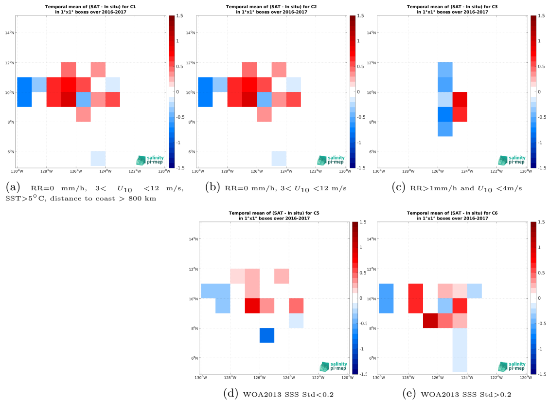
Figure 12: Temporal mean gridded over spatial boxes of size 1^\circ \times 1^\circ of \Delta SSS (SMOS SSS L2Q v331 - With FLAG (CMEMS-CATDS-CPDC) - Salinity Snake (SPURS 2)) for 5 different sub-datasets corresponding to:RR=0 mm/h, 3 < U_{10} < 12 m/s, SST>5°C, distance to coast > 800 km (a), RR=0 mm/h, 3 < U_{10} < 12 m/s (b), RR>1mm/h and U_{10} < 4 m/s (c), WOA2013 SSS Std<0.2 (d), WOA2013 SSS Std>0.2 (e).
