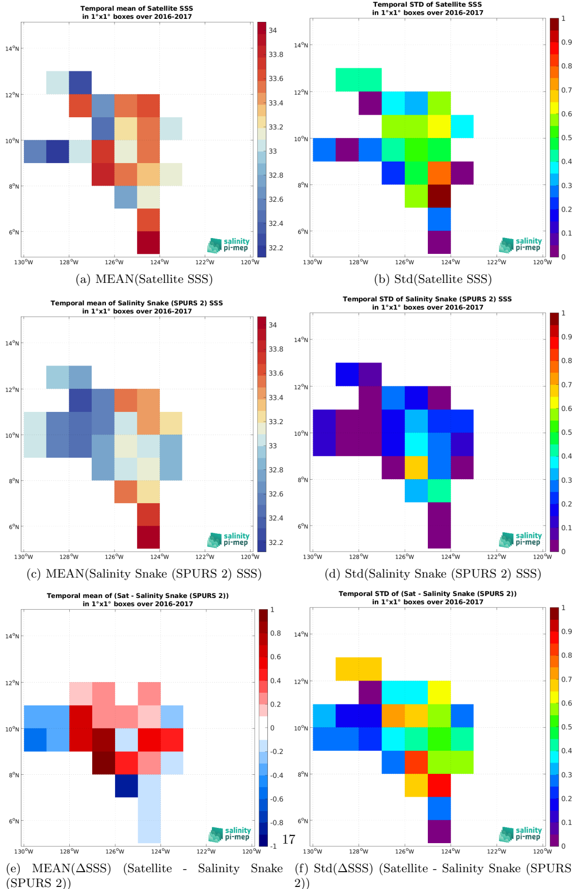
Figure 6: Temporal mean (left) and Std (right) of SSS from SMOS SSS L2Q v331 - With FLAG (CMEMS-CATDS-CPDC) (top), Salinity Snake (SPURS 2) (middle), and of \Delta SSS (Satellite - Salinity Snake (SPURS 2)). Only match-up pairs are used to generate these maps.
