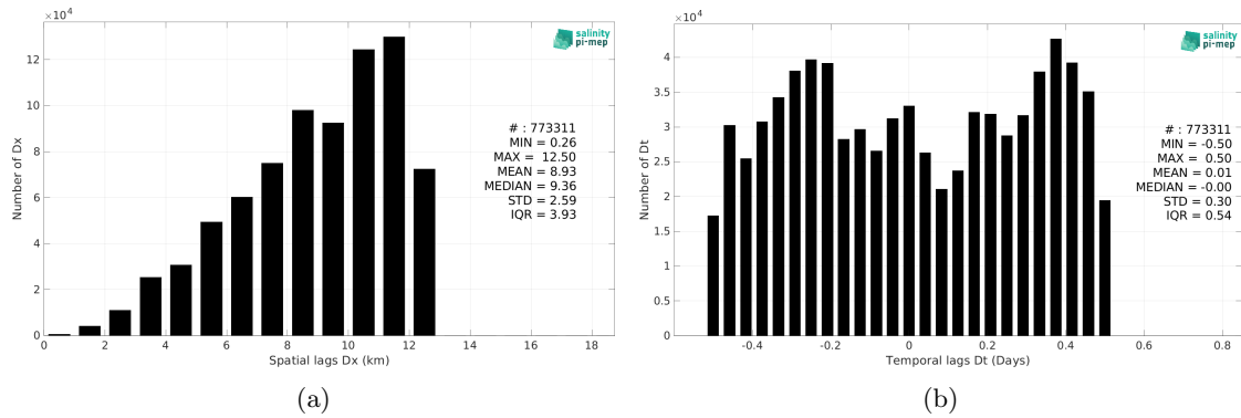
Figure 5: Histograms of the spatial (a) and temporal (b) lags between the location/time of the Salinity Snake (SPURS 2) measurement and the date of the corresponding SMOS SSS L2Q v331 - With FLAG (CMEMS-CATDS-CPDC) SSS pixel.
