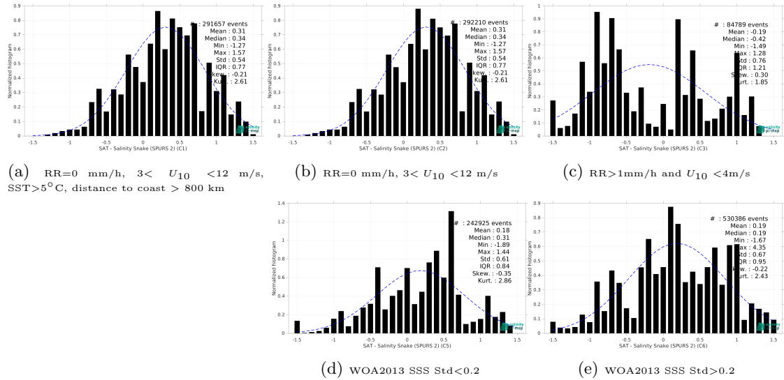
Figure 13: Normalized histogram of \Delta SSS (SMOS SSS L2Q v331 - With FLAG (CMEMS-CATDS-CPDC) - Salinity Snake (SPURS 2)) for 5 different subdatasets corresponding to: RR=0 mm/h, 3 < U_{10} < 12 m/s, SST > 5°C, distance to coast > 800 km (a), RR=0 mm/h, 3 < U_{10} < 12 m/s (b), RR > 1mm/h and U_{10} < 4 m/s (c), WOA2013 SSS Std < 0.2 (d), WOA2013 SSS Std > 0.2 (e).
