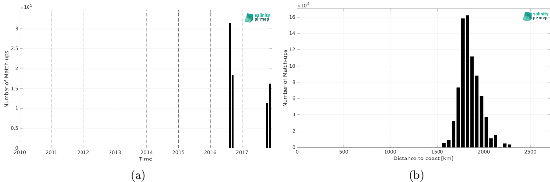
Figure 1: Number of match-ups between Salinity Snake (SPURS 2) and SMOS SSS L2Q v331 - With FLAG (CMEMS-CATDS-CPDC) SSS as a function of time (a) and as function of the distance to coast (b) over the SPURS 2 Pi-MEP region and for the full satellite product period.
