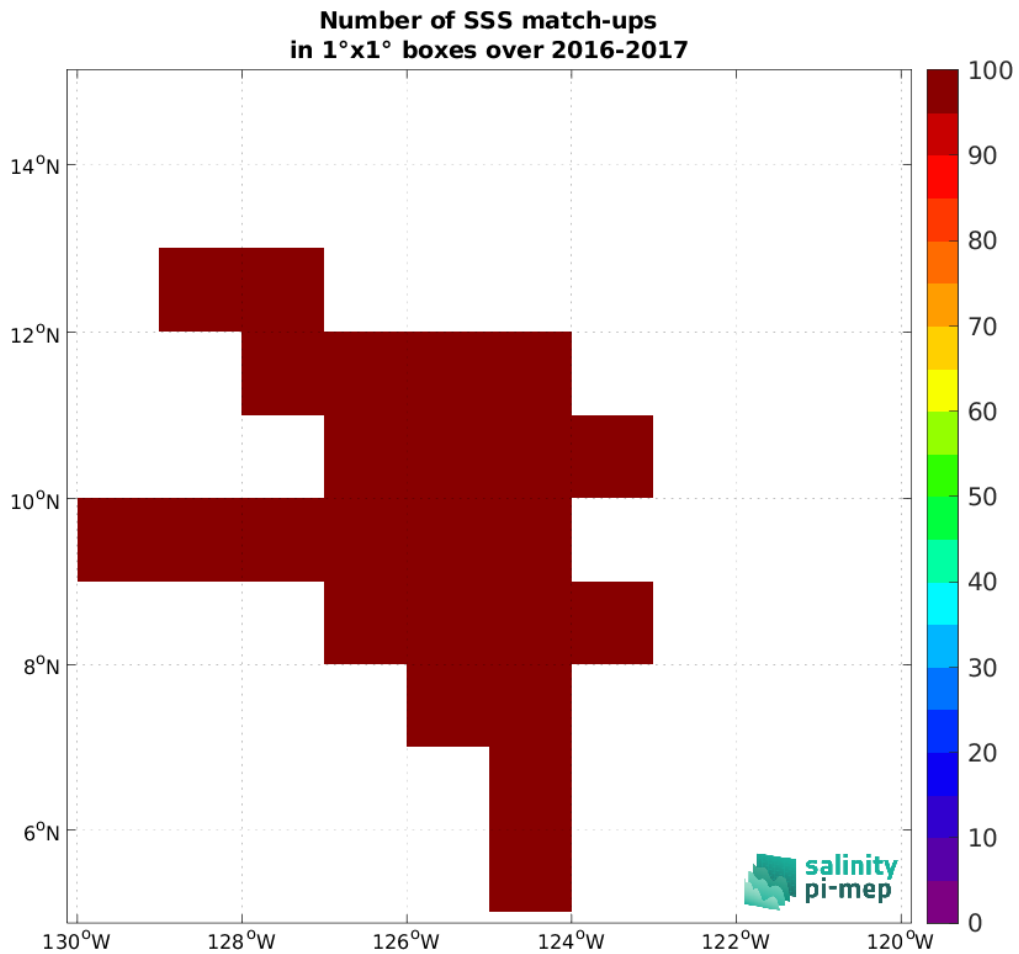
Figure 4: Number of SSS match-ups between Salinity Snake (SPURS 2) SSS and the SMOS SSS L2Q v331 - With FLAG (CMEMS-CATDS-CPDC) SSS product for the SPURS 2 Pi-MEP region over 1°x1° boxes and for the full satellite product period.
