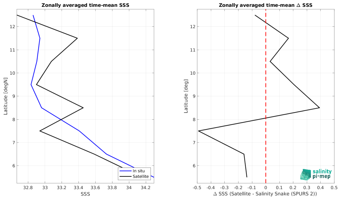
Figure 8: Left panel: Zonal mean SSS from SMOS SSS L2Q v331 - With FLAG (CMEMS-CATDS-CPDC) satellite product (black) and from Salinity Snake (SPURS 2) (blue). Right panel: Zonal mean of \Delta SSS (Satellite - Salinity Snake (SPURS 2)) for all the collected Pi-MEP match-up pairs estimated over the full satellite product period.
