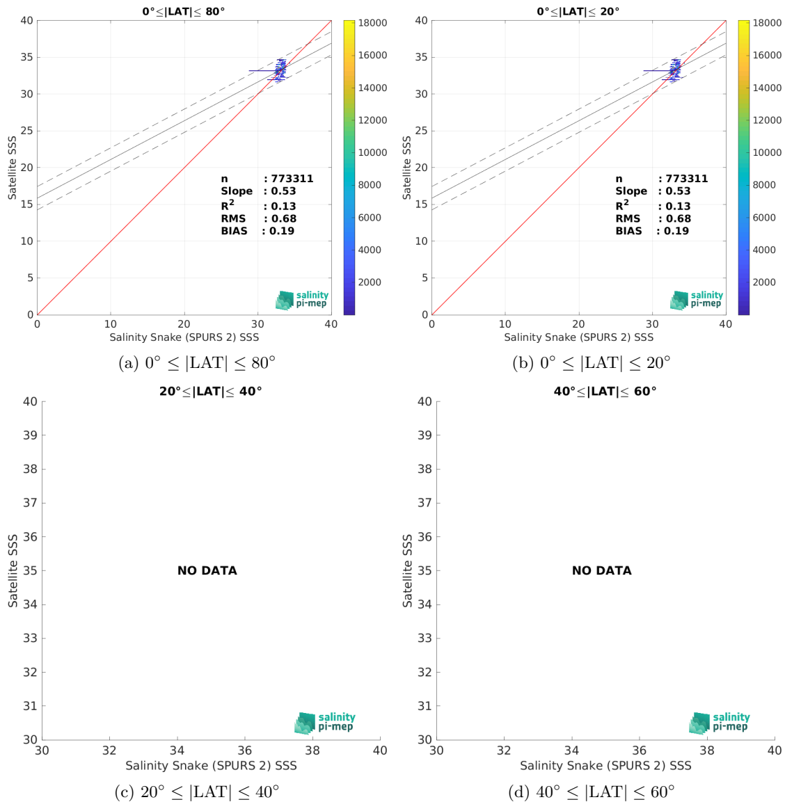
Figure 9: Contour maps of the concentration of SMOS SSS L2Q v331 - With FLAG (CMEMS-CATDS-CPDC) SSS (y-axis) versus Salinity Snake (SPURS 2) SSS (x-axis) at match-up pairs for different latitude bands. For each plot, the red line shows x=y . The black thin and dashed lines indicate a linear fit through the data cloud and the \pm 95\% confidence levels, respectively. The number match-up pairs n , the slope and R^2 coefficient of the linear fit, the root mean square (RMS) and the mean bias between satellite and in situ data are indicated for each latitude band in each plots.
