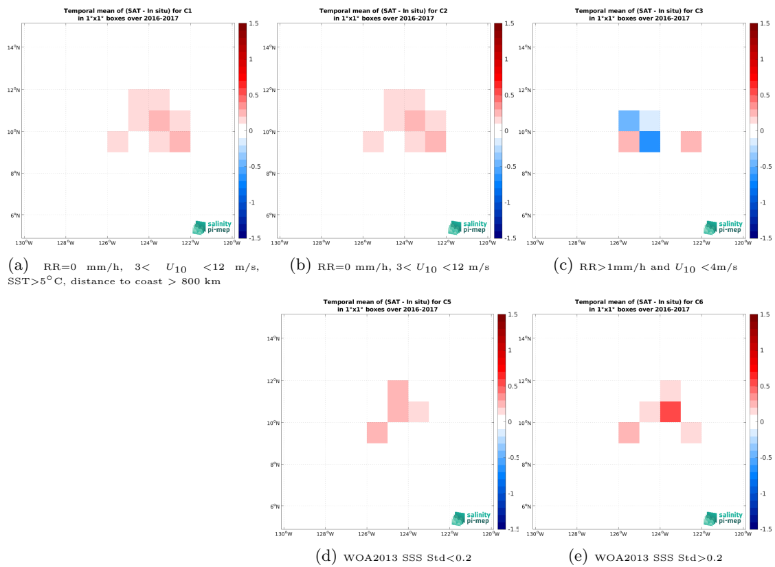
Figure 14: Temporal mean gridded over spatial boxes of size 1^\circ \times 1^\circ of \Delta SSS (SMOS SSS L2Q v331 - With FLAG (CMEMS-CATDS-CPDC) - Seaglider (SPURS 2)) for 5 different subdatasets corresponding to:RR=0 mm/h, 3 < U_{10} < 12 m/s, SST>5°C, distance to coast > 800 km (a), RR=0 mm/h, 3 < U_{10} < 12 m/s (b), RR>1mm/h and U_{10} < 4 m/s (c), WOA2013 SSS Std<0.2 (d), WOA2013 SSS Std>0.2 (e).
