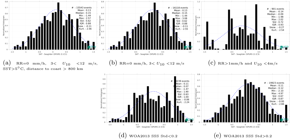
Figure 15: Normalized histogram of \Delta SSS (SMOS SSS L2Q v331 - With FLAG (CMEMS-CATDS-CPDC) - Seaglider (SPURS 2)) for 5 different subdatasets corresponding to: RR=0 mm/h, 3 < U_{10} < 12 m/s, SST>5°C, distance to coast > 800 km (a), RR=0 mm/h, 3 < U_{10} < 12 m/s (b), RR>1mm/h and U_{10} < 4 m/s (c), WOA2013 SSS Std<0.2 (d), WOA2013 SSS Std>0.2 (e).
