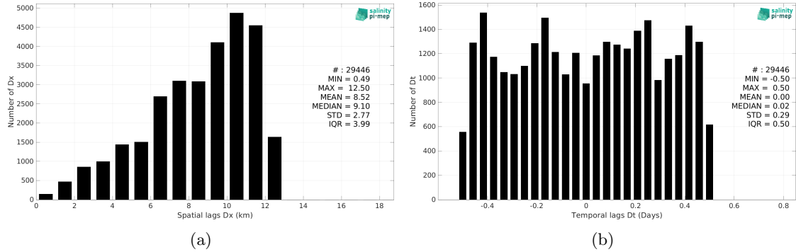
Figure 6: Histograms of the spatial (a) and temporal (b) lags between the location/time of the Seaglider (SPURS 2) measurement and the date of the corresponding SMOS SSS L2Q v331 - With FLAG (CMEMS-CATDS-CPDC) SSS pixel.
