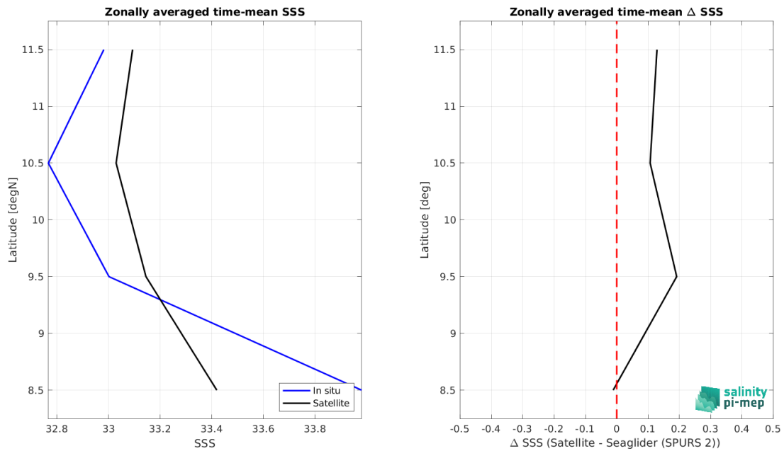
Figure 9: Left panel: Zonal mean SSS from SMOS SSS L2Q v331 - With FLAG (CMEMS-CATDS-CPDC) satellite product (black) and from Seagliders (SPURS 2) (blue). Right panel: Zonal mean of \Delta SSS (Satellite - Seagliders (SPURS 2)) for all the collected Pi-MEP match-up pairs estimated over the full satellite product period.
