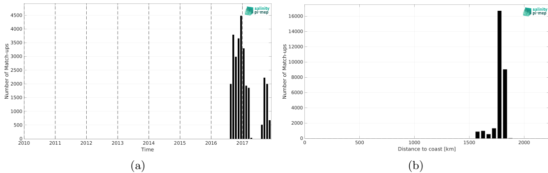
Figure 2: Number of match-ups between Seaglider (SPURS 2) and SMOS SSS L2Q v331 - With FLAG (CMEMS-CATDS-CPDC) SSS as a function of time (a) and as function of the distance to coast (b) over the SPURS 2 Pi-MEP region and for the full satellite product period.
