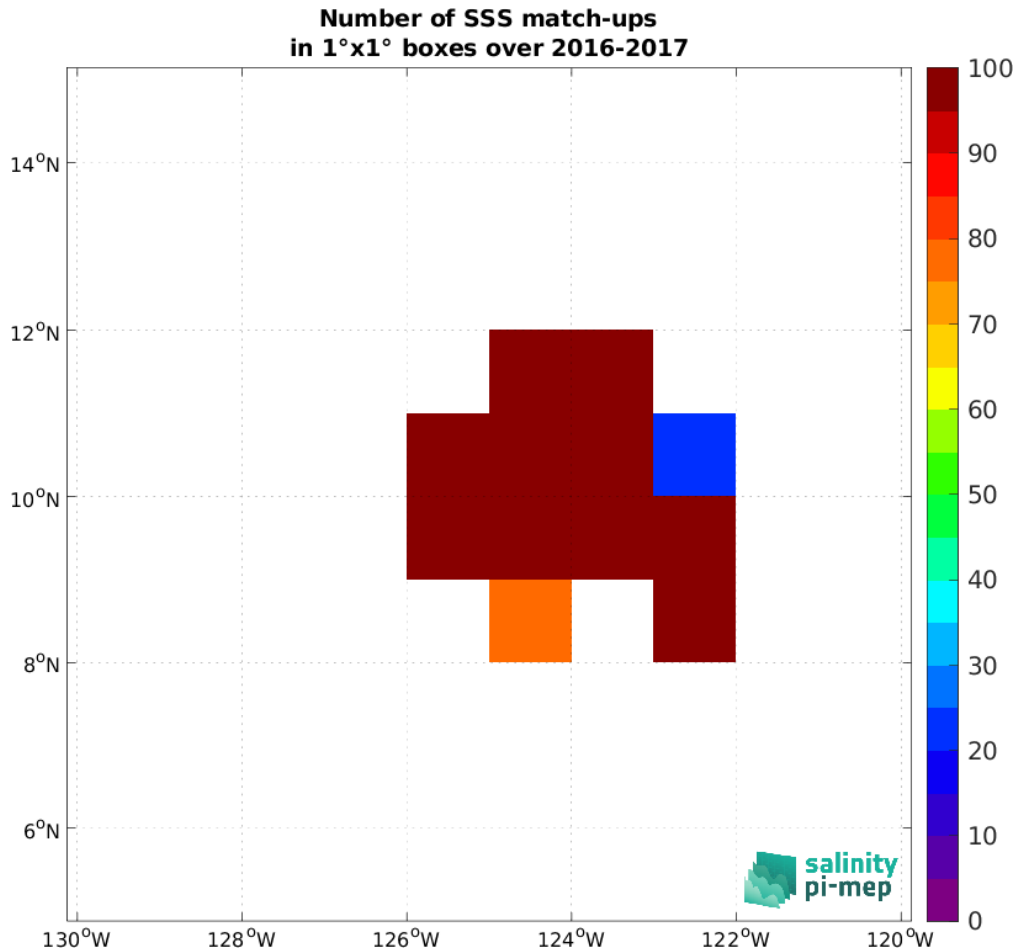
Figure 5: Number of SSS match-ups between Seaglider (SPURS 2) SSS and the SMOS SSS L2Q v331 - With FLAG (CMEMS-CATDS-CPDC) SSS product for the SPURS 2 Pi-MEP region over 1^\circ \times 1^\circ boxes and for the full satellite product period.
