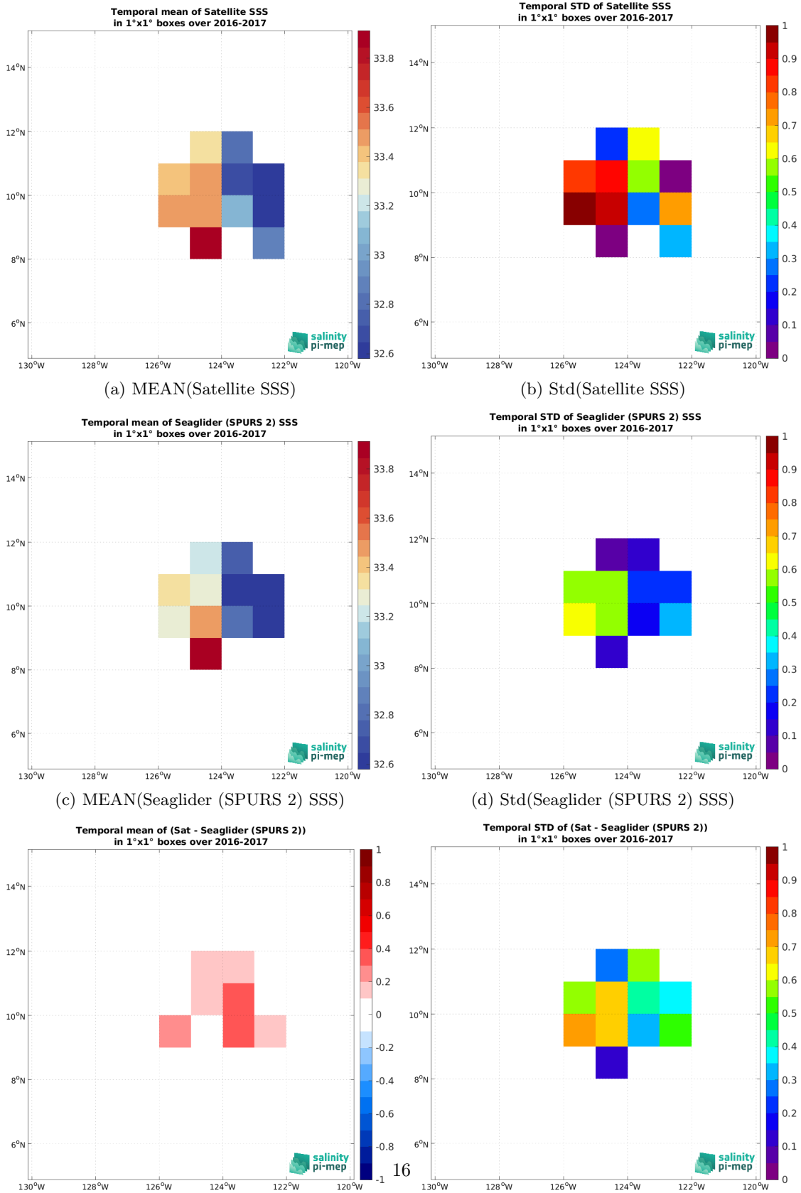
Figure 6: Temporal mean (left) and Std (right) of SSS from SMOS SSS L2Q v331 - With FLAG (CMEMS-CATDS-CPDC) (top), Seaglider (SPURS 2) (middle), and of \Delta SSS (Satellite - Seaglider (SPURS 2)). Only match-up pairs are used to generate these maps.
