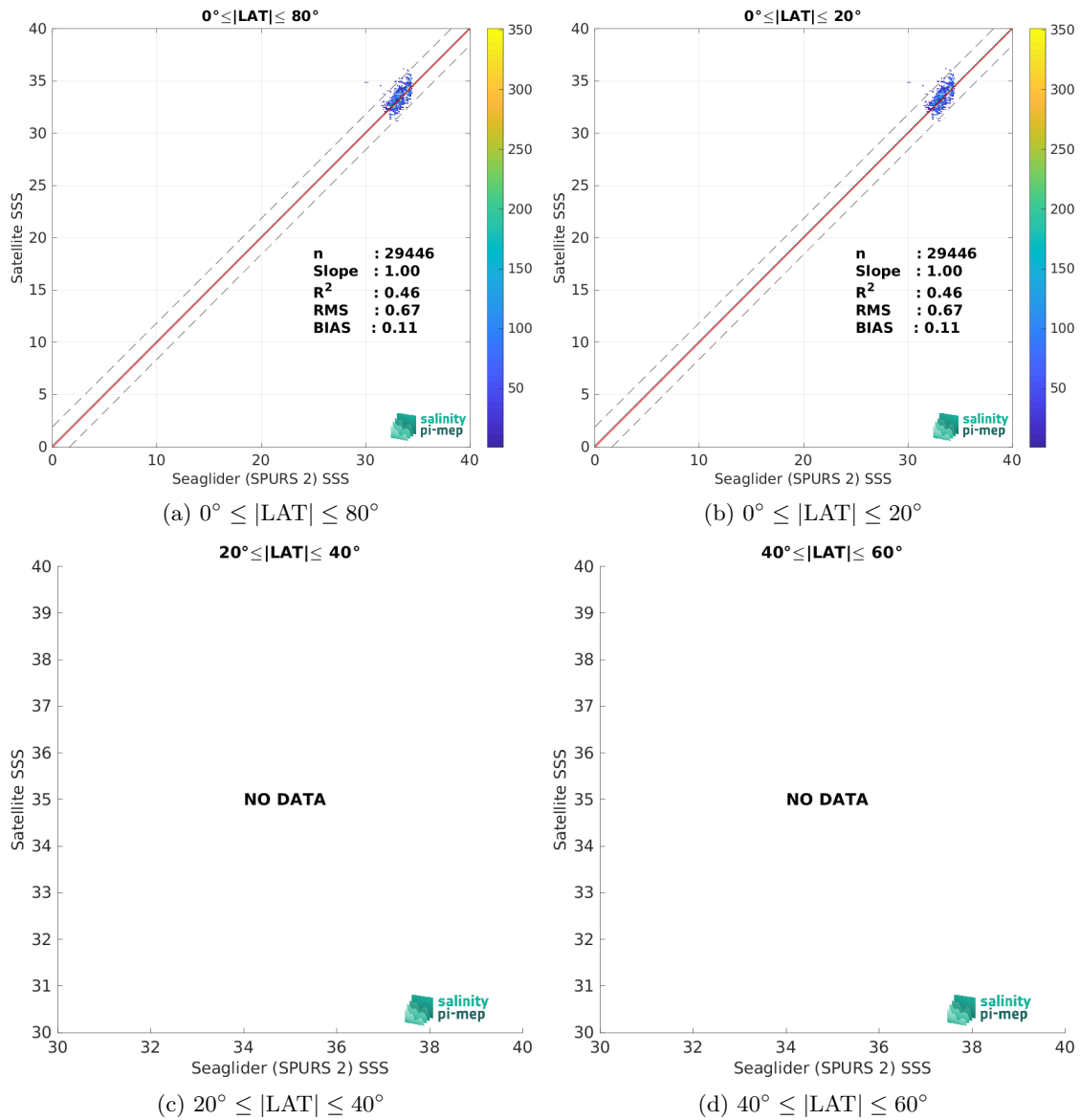
Figure 9: Contour maps of the concentration of SMOS SSS L2Q v331 - With FLAG (CMEMS-CATDS-CPDC) SSS (y-axis) versus Seaglider (SPURS 2) SSS (x-axis) at match-up pairs for different latitude bands. For each plot, the red line shows x=y . The black thin and dashed lines indicate a linear fit through the data cloud and the \pm 95\% confidence levels, respectively. The number match-up pairs n , the slope and R^2 coefficient of the linear fit, the root mean square (RMS) and the mean bias between satellite and in situ data are indicated for each latitude band in each plots.
