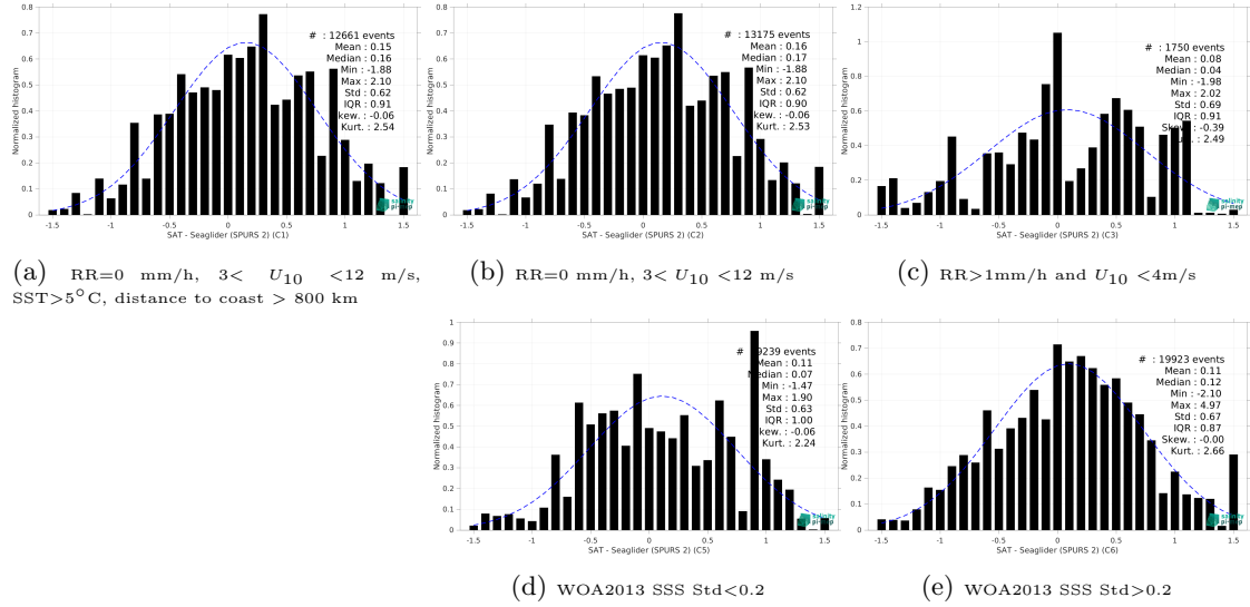
Figure 13: Normalized histogram of \Delta SSS (SMOS SSS L2Q v331 - With FLAG (CMEMS-CATDS-CPDC) - Seaglider (SPURS 2)) for 5 different subdatasets corresponding to: RR=0 mm/h, 3 < U_{10} < 12 m/s, SST >5^{\circ} C, distance to coast > 800 km (a), RR=0 mm/h, 3 < U_{10} < 12 m/s (b), RR >1 mm/h and U_{10} < 4 m/s (c), WOA2013 SSS Std <0.2 (d), WOA2013 SSS Std >0.2 (e).
