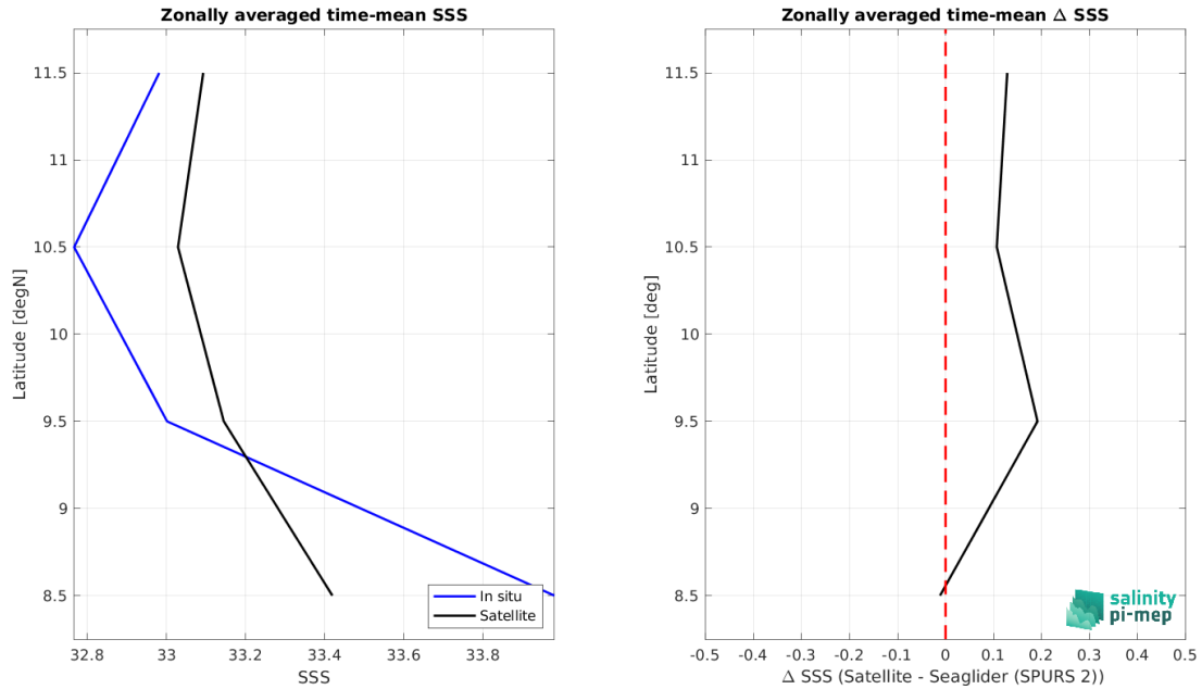
Figure 8: Left panel: Zonal mean SSS from SMOS SSS L2Q v331 - With FLAG (CMEMS-CATDS-CPDC) satellite product (black) and from Seaglider (SPURS 2) (blue). Right panel: Zonal mean of \Delta SSS (Satellite - Seaglider (SPURS 2)) for all the collected Pi-MEP match-up pairs estimated over the full satellite product period.
