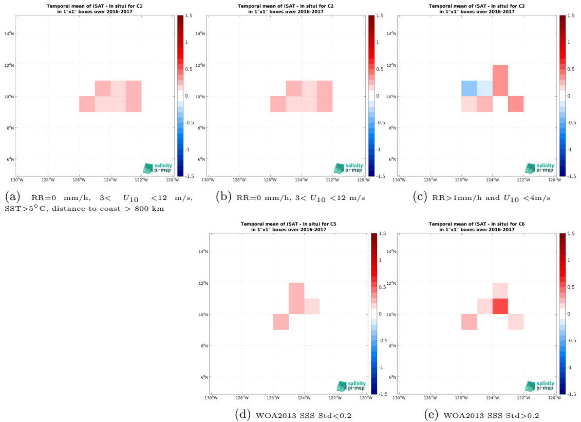
Figure 12: Temporal mean gridded over spatial boxes of size 1^{\circ}\times 1^{\circ} of \Delta\text{SSS} (SMOS SSS L2Q v331 - With FLAG (CMEMS-CATDS-CPDC) - Seaglider (SPURS 2)) for 5 different subdatasets corresponding to:RR=0 mm/h, 3 < U_{10} < 12 m/s, SST >5^{\circ}\text{C} , distance to coast > 800 km (a), RR=0 mm/h, 3 < U_{10} < 12 m/s (b), RR >1 mm/h and U_{10} < 4 m/s (c), WOA2013 SSS Std <0.2 (d), WOA2013 SSS Std >0.2 (e).
