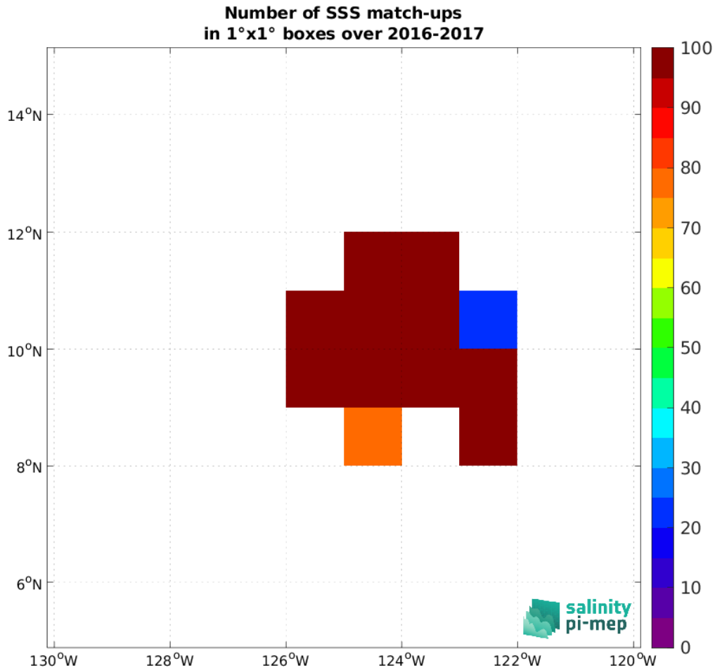
Figure 4: Number of SSS match-ups between Seaglider (SPURS 2) SSS and the SMOS SSS L2Q v331 - With FLAG (CMEMS-CATDS-CPDC) SSS product for the SPURS 2 Pi-MEP region over 1^\circ \times 1^\circ boxes and for the full satellite product period.
