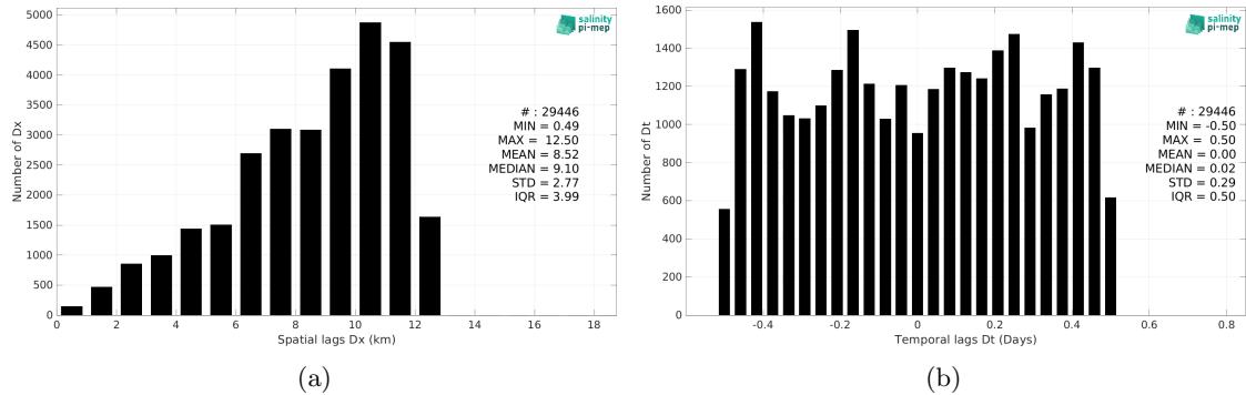
Figure 5: Histograms of the spatial (a) and temporal (b) lags between the location/time of the Seaglider (SPURS 2) measurement and the date of the corresponding SMOS SSS L2Q v331 - With FLAG (CMEMS-CATDS-CPDC) SSS pixel.
