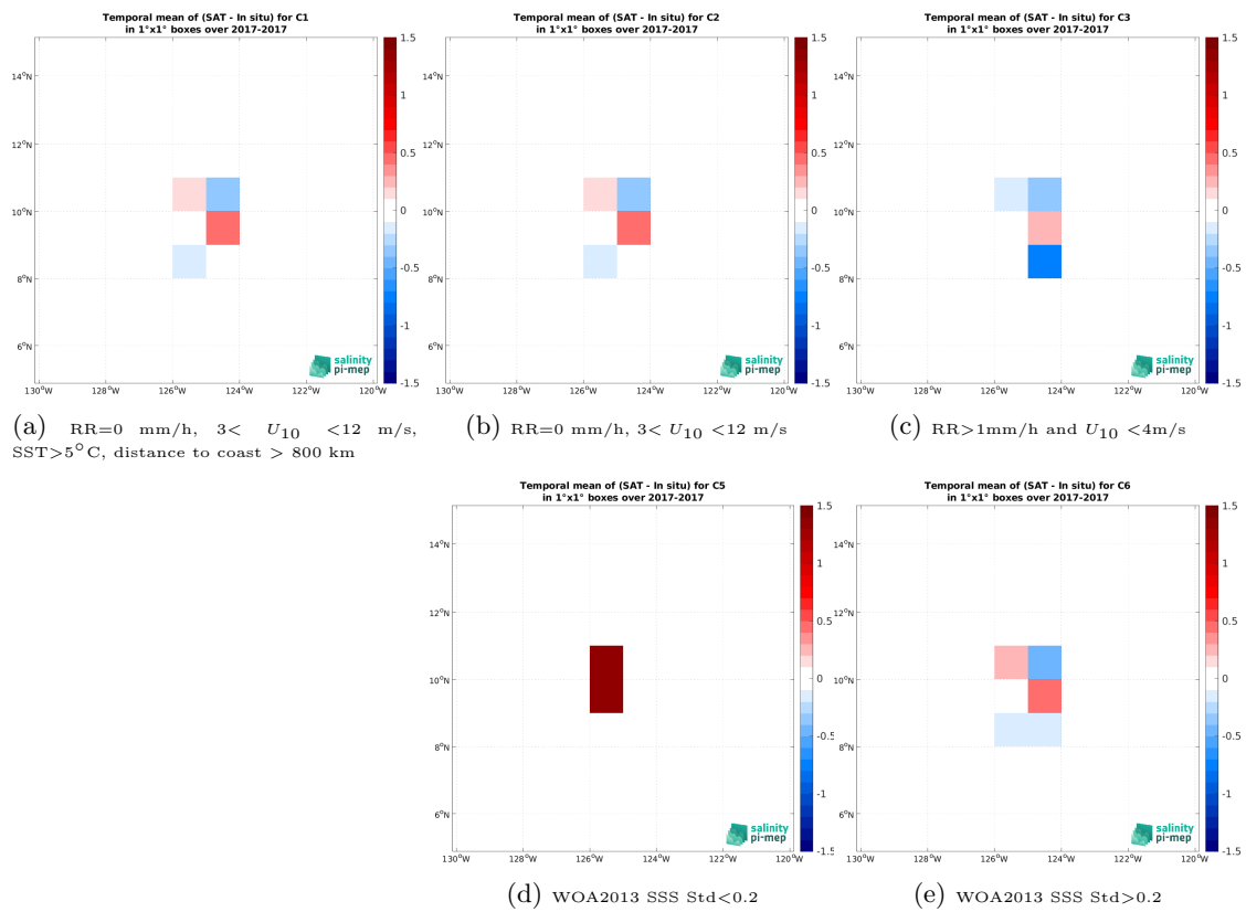
Figure 14: Temporal mean gridded over spatial boxes of size 1^\circ \times 1^\circ of \Delta SSS (SMOS SSS L2Q v331 - With FLAG (CMEMS-CATDS-CPDC) - Sairdrone (SPURS 2)) for 5 different subdatasets corresponding to:RR=0 mm/h, 3 < U_{10} < 12 m/s, SST >5^\circ C, distance to coast > 800 km (a), RR=0 mm/h, 3 < U_{10} < 12 m/s (b), RR >1 mm/h and U_{10} < 4 m/s (c), WOA2013 SSS Std <0.2 (d), WOA2013 SSS Std >0.2 (e).
