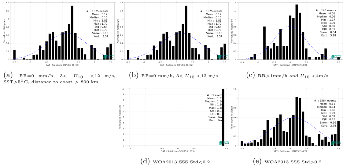
Figure 15: Normalized histogram of \Delta SSS (SMOS SSS L2Q v331 - With FLAG (CMEMS-CATDS-CPDC) - Saildrone (SPURS 2)) for 5 different subdatasets corresponding to: RR=0 mm/h, 3 < U_{10} < 12 m/s, SST > 5°C, distance to coast > 800 km (a), RR=0 mm/h, 3 < U_{10} < 12 m/s (b), RR > 1mm/h and U_{10} < 4 m/s (c), WOA2013 SSS Std < 0.2 (d), WOA2013 SSS Std > 0.2 (e).
