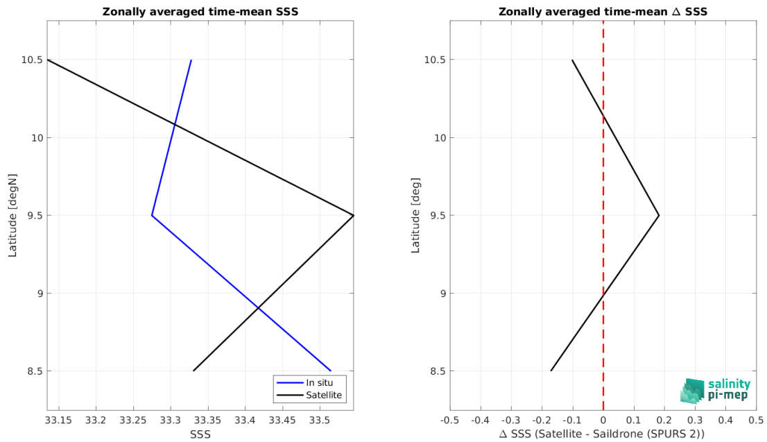
Figure 9: Left panel: Zonal mean SSS from SMOS SSS L2Q v331 - With FLAG (CMEMS-CATDS-CPDC) satellite product (black) and from Sairdron (SPURS 2) (blue). Right panel: Zonal mean of \Delta SSS (Satellite - Sairdron (SPURS 2)) for all the collected Pi-MEP match-up pairs estimated over the full satellite product period.
