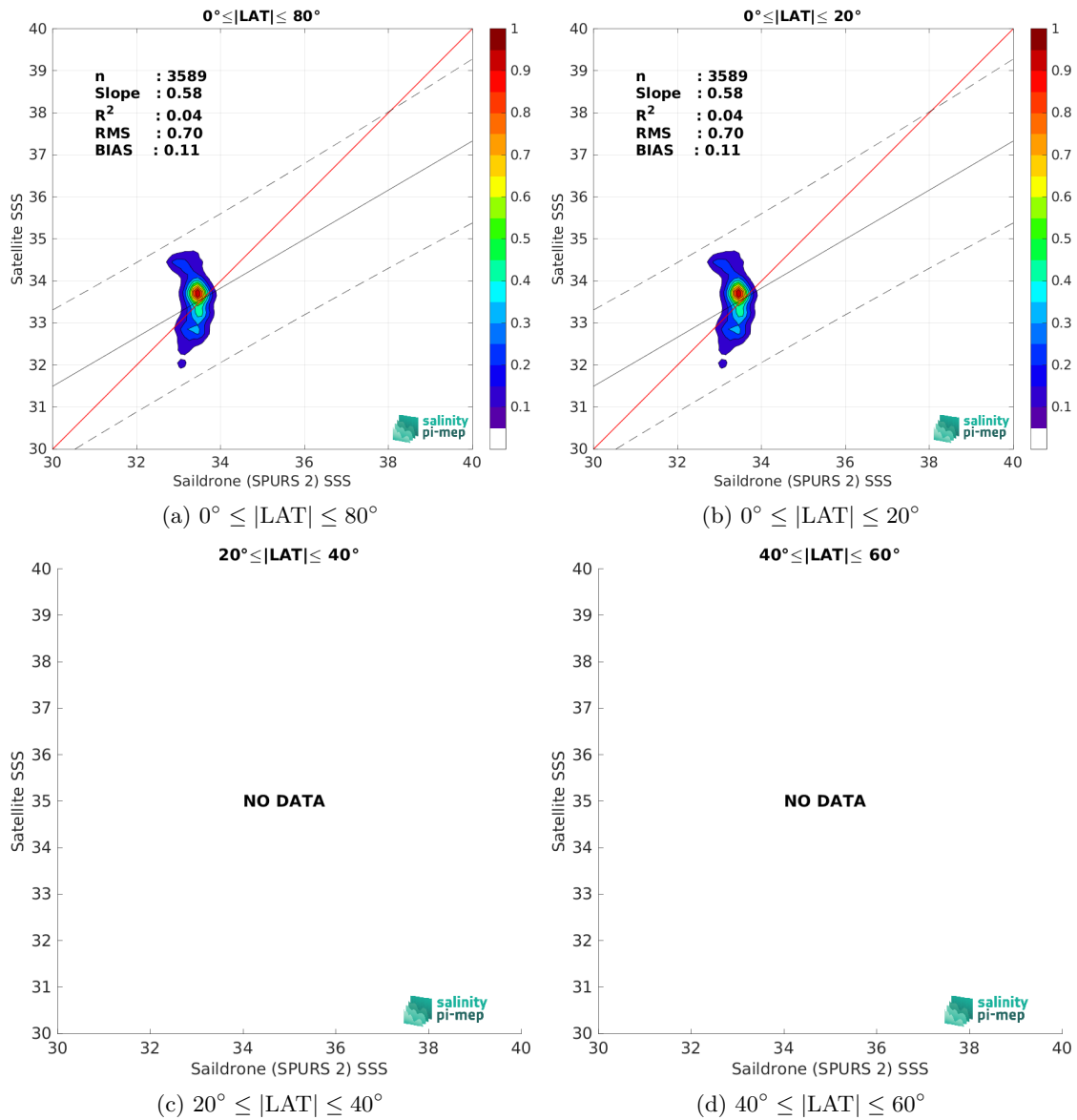
Figure 10: Contour maps of the concentration of SMOS SSS L2Q v331 - With FLAG (CMEMS-CATDS-CPDC) SSS (y-axis) versus Saildrone (SPURS 2) SSS (x-axis) at match-up pairs for different latitude bands. For each plot, the red line shows x=y . The black thin and dashed lines indicate a linear fit through the data cloud and the \pm 95\% confidence levels, respectively. The number match-up pairs n , the slope and R^2 coefficient of the linear fit, the root mean square (RMS) and the mean bias between satellite and in situ data are indicated for each latitude band in each plots.
