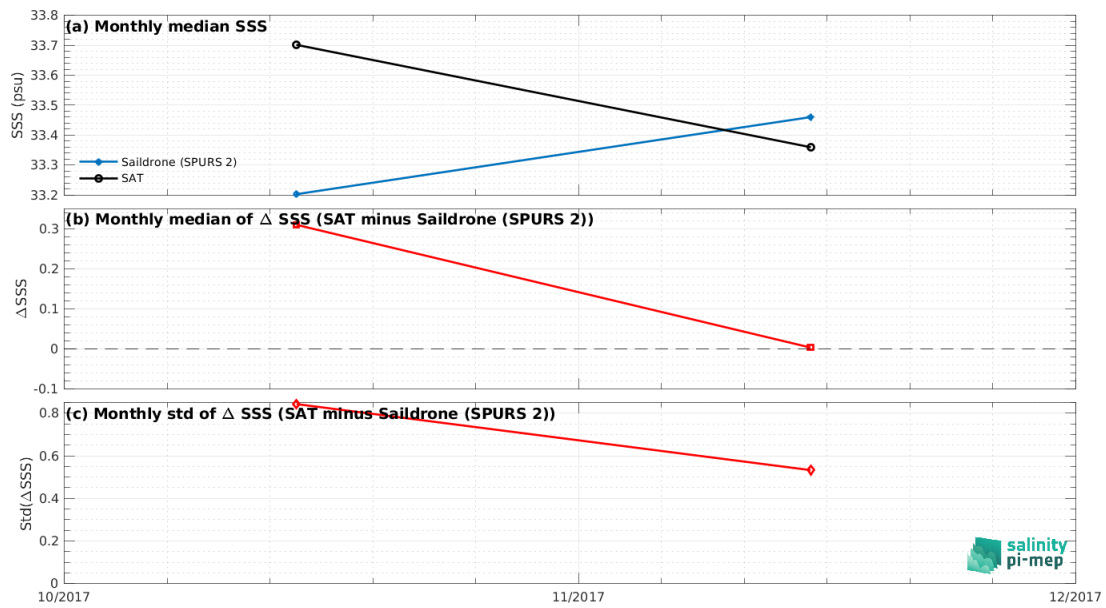
Figure 7: Time series of the monthly median SSS (top), median of \Delta SSS (Satellite - Sairdron (SPURS 2)) and Std of \Delta SSS (Satellite - Sairdron (SPURS 2)) over the SPURS 2 Pi-MEP region considering all match-ups collected by the Pi-MEP.
