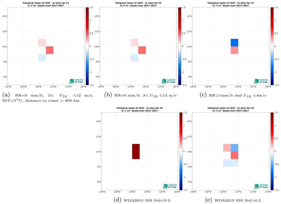
Figure 12: Temporal mean gridded over spatial boxes of size 1^{\circ}\times 1^{\circ} of \Delta\text{SSS} (SMOS SSS L2Q v331 - With FLAG (CMEMS-CATDS-CPDC) - Sairdrone (SPURS 2)) for 5 different subdatasets corresponding to:RR=0 mm/h, 3 < U_{10} < 12 m/s, SST >5^{\circ}\text{C} , distance to coast > 800 km (a), RR=0 mm/h, 3 < U_{10} < 12 m/s (b), RR >1 mm/h and U_{10} < 4 m/s (c), WOA2013 SSS Std <0.2 (d), WOA2013 SSS Std >0.2 (e).
