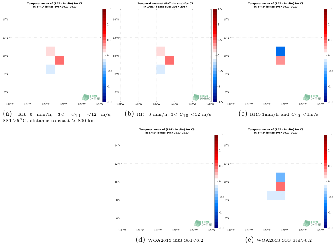
Figure 12: Temporal mean gridded over spatial boxes of size 1^{\circ}\times 1^{\circ} of \Delta\text{SSS} (SMOS SSS L2Q v331 - With FLAG (CMEMS-CATDS-CPDC) - Saildrone (SPURS 2)) for 5 different subdatasets corresponding to:RR=0 mm/h, 3 < U_{10} < 12 m/s, SST >5^{\circ}\text{C} , distance to coast > 800 km (a), RR=0 mm/h, 3 < U_{10} < 12 m/s (b), RR >1 mm/h and U_{10} < 4 m/s (c), WOA2013 SSS Std <0.2 (d), WOA2013 SSS Std >0.2 (e).
