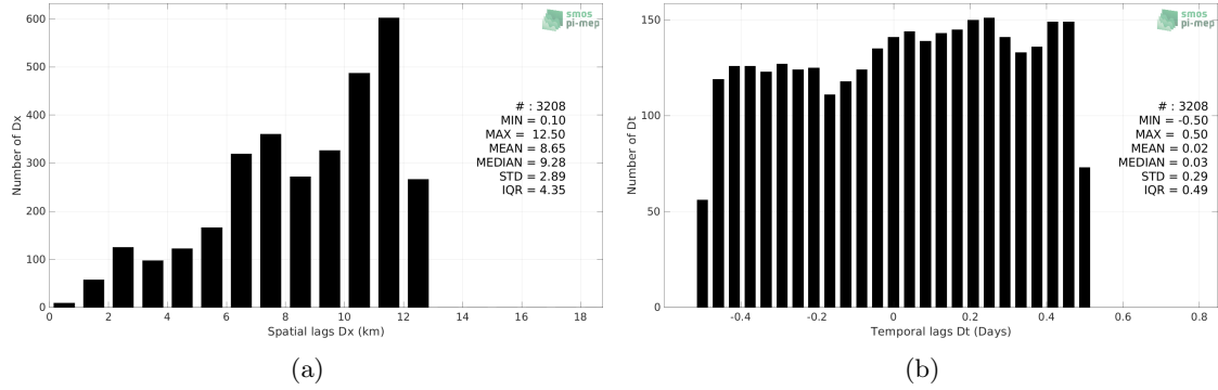
Figure 5: Histograms of the spatial (a) and temporal (b) lags between the location/time of the Saildrone (SPURS 2) measurement and the date of the corresponding SMOS SSS L2Q v331 - With FLAG (CMEMS-CATDS-CPDC) SSS pixel.
