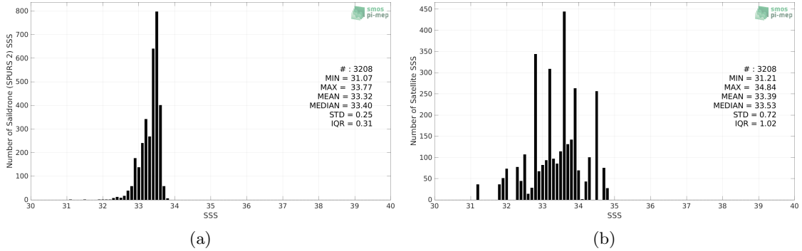
Figure 2: Histograms of SSS from Saildrone (SPURS 2) (a) and SMOS SSS L2Q v331 - With FLAG (CMEMS-CATDS-CPDC) (b) considering all match-up pairs per bins of 0.1 over the SPURS 2 Pi-MEP region and for the full satellite product period.
