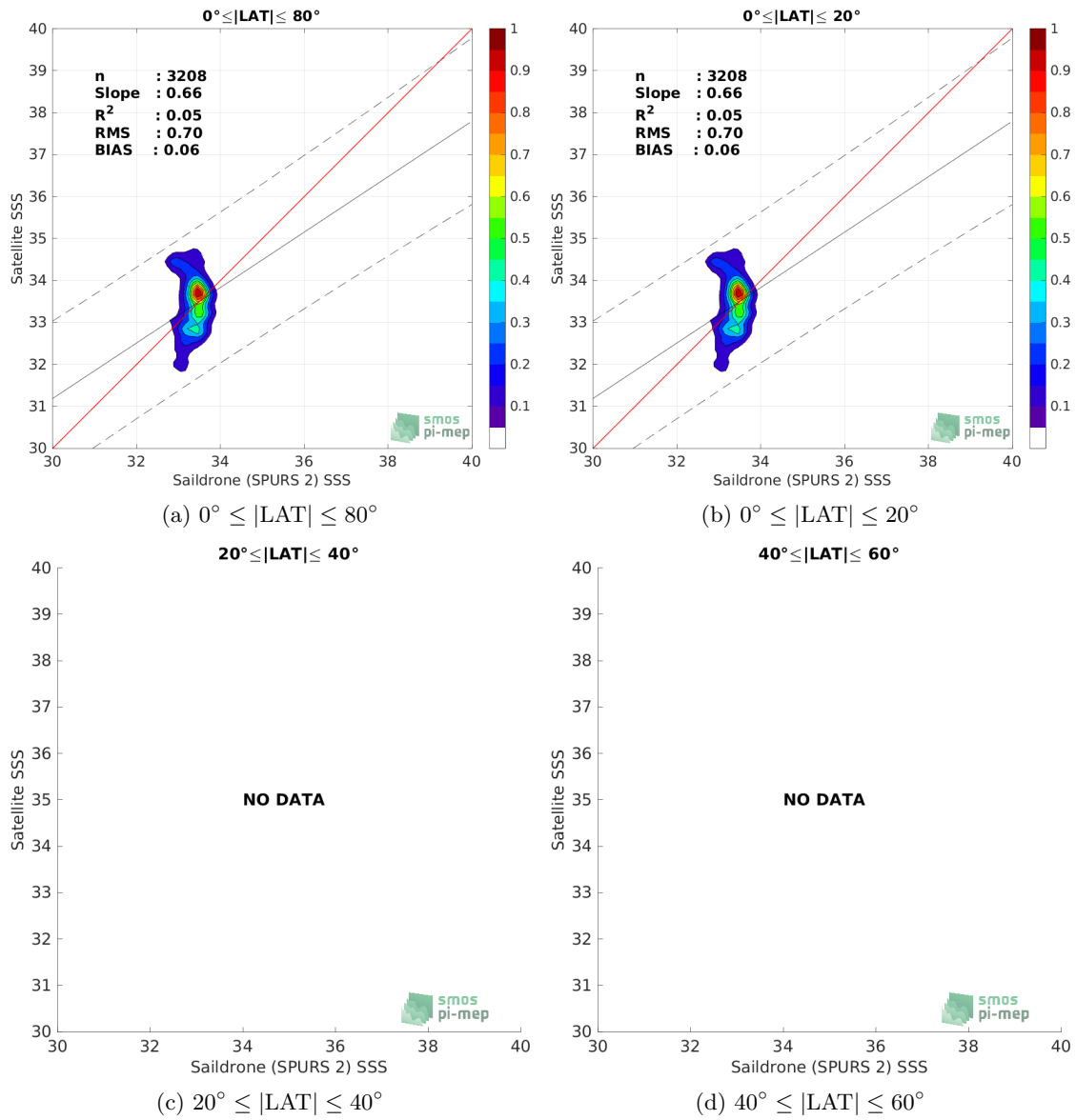
Figure 9: Contour maps of the concentration of SMOS SSS L2Q v331 - With FLAG (CMEMS-CATDS-CPDC) SSS (y-axis) versus Saildrone (SPURS 2) SSS (x-axis) at match-up pairs for different latitude bands. For each plot, the red line shows x=y . The black thin and dashed lines indicate a linear fit through the data cloud and the \pm 95\% confidence levels, respectively. The number match-up pairs n , the slope and R^2 coefficient of the linear fit, the root mean square (RMS) and the mean bias between satellite and in situ data are indicated for each latitude band in each plots.
