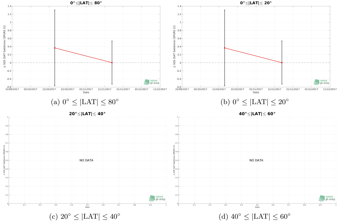
Figure 10: Monthly median (red curves) of \Delta SSS (Satellite - Sairdrone (SPURS 2)) and \pm 1 Std (black vertical thick bars) as function of time for all the collected Pi-MEP match-up pairs estimated over the SPURS 2 Pi-MEP region and for the full satellite product period are shown for different latitude bands: (a) 80^\circ\text{S}-80^\circ\text{N} , (b) 20^\circ\text{S}-20^\circ\text{N} , (c) 40^\circ\text{S}-20^\circ\text{S} and 20^\circ\text{N}-40^\circ\text{N} and (d) 60^\circ\text{S}-40^\circ\text{S} and 40^\circ\text{N}-60^\circ\text{N} .
