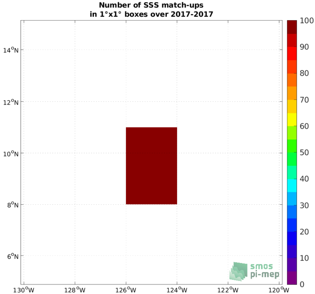
Figure 4: Number of SSS match-ups between Saildrone (SPURS 2) SSS and the SMOS SSS L2Q v331 - With FLAG (CMEMS-CATDS-CPDC) SSS product for the SPURS 2 Pi-MEP region over 1^\circ \times 1^\circ boxes and for the full satellite product period.
