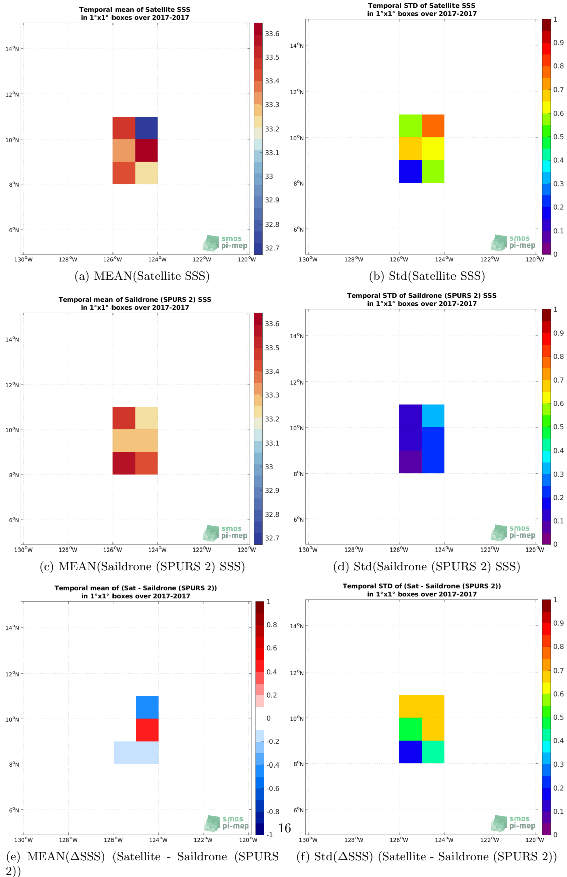
Figure 6: Temporal mean (left) and Std (right) of SSS from SMOS SSS L2Q v331 - With FLAG (CMEMS-CATDS-CPDC) (top), Saildrone (SPURS 2) (middle), and of \Delta SSS (Satellite - Saildrone (SPURS 2)). Only match-up pairs are used to generate these maps.
