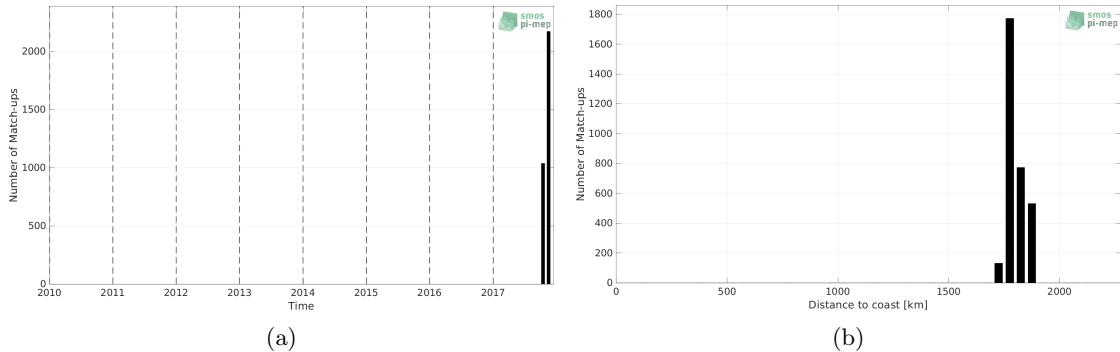
Figure 1: Number of match-ups between Saildrone (SPURS 2) and SMOS SSS L2Q v331 - With FLAG (CMEMS-CATDS-CPDC) SSS as a function of time (a) and as function of the distance to coast (b) over the SPURS 2 Pi-MEP region and for the full satellite product period.
