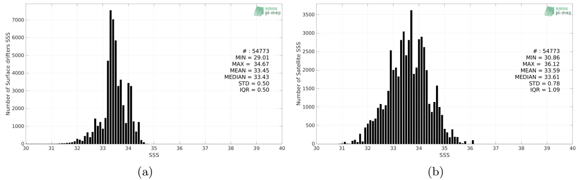
Figure 2: Histograms of SSS from Surface drifters (a) and SMOS SSS L2Q v331 - With FLAG (CMEMS-CATDS-CPDC) (b) considering all match-up pairs per bins of 0.1 over the SPURS 2 Pi-MEP region and for the full satellite product period.
