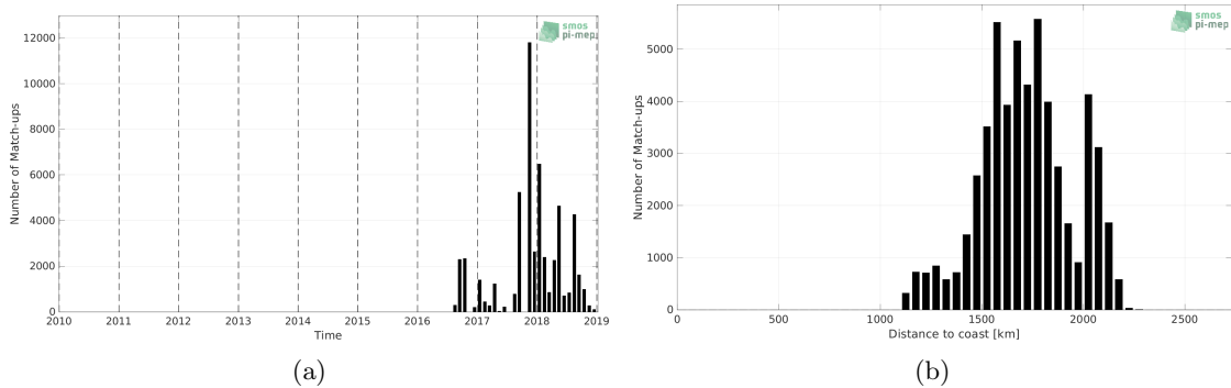
Figure 1: Number of match-ups between Surface drifters and SMOS SSS L2Q v331 - With FLAG (CMEMS-CATDS-CPDC) SSS as a function of time (a) and as function of the distance to coast (b) over the SPURS 2 Pi-MEP region and for the full satellite product period.
