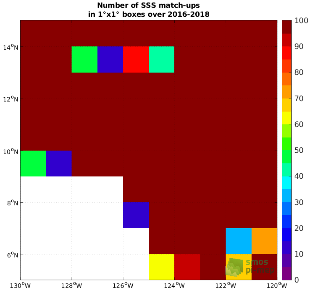
Figure 3: Number of SSS match-ups between Surface drifters SSS and the SMOS SSS L2Q v331 - With FLAG (CMEMS-CATDS-CPDC) SSS product for the SPURS 2 Pi-MEP region over 1^\circ \times 1^\circ boxes and for the full satellite product period.
