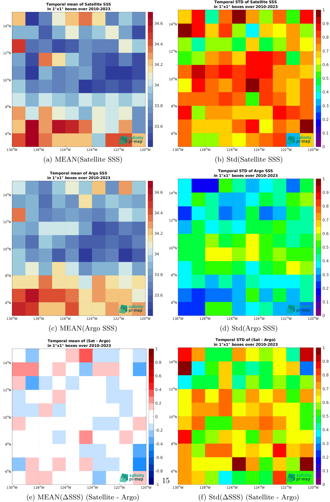
Figure 6: Temporal mean (left) and Std (right) of SSS from SMOS SSS L2Q v331 - With FLAG (CMEMS-CATDS-CPDC) (top), Argo (middle), and of \Delta SSS (Satellite - Argo). Only match-up pairs are used to generate these maps.
