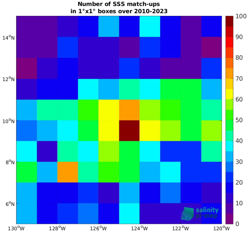
Figure 4: Number of SSS match-ups between Argo SSS and the SMOS SSS L2Q v331 - With FLAG (CMEMS-CATDS-CPDC) SSS product for the SPURS 2 Pi-MEP region over 1^\circ \times 1^\circ boxes and for the full satellite product period.
