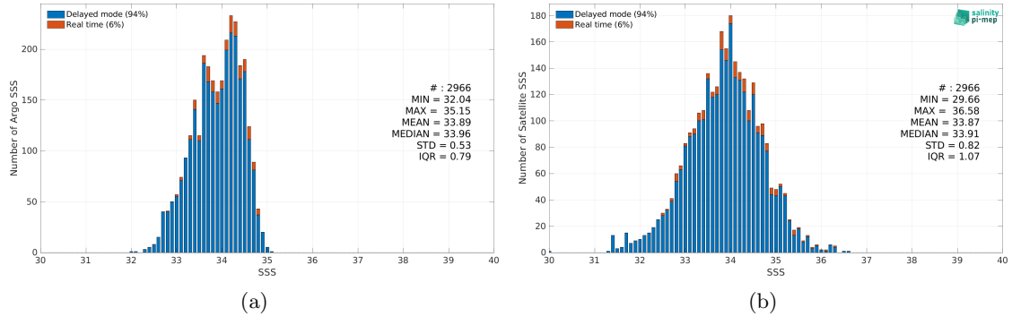
Figure 2: Histograms of SSS from Argo (a) and SMOS SSS L2Q v331 - With FLAG (CMEMS-CATDS-CPDC) (b) considering all match-up pairs per bins of 0.1 over the SPURS 2 Pi-MEP region and for the full satellite product period.
