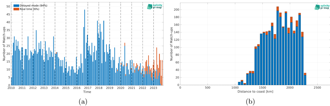
Figure 1: Number of match-ups between Argo and SMOS SSS L2Q v331 - With FLAG (CMEMS-CATDS-CPDC) SSS as a function of time (a) and as function of the distance to coast (b) over the SPURS 2 Pi-MEP region and for the full satellite product period.
