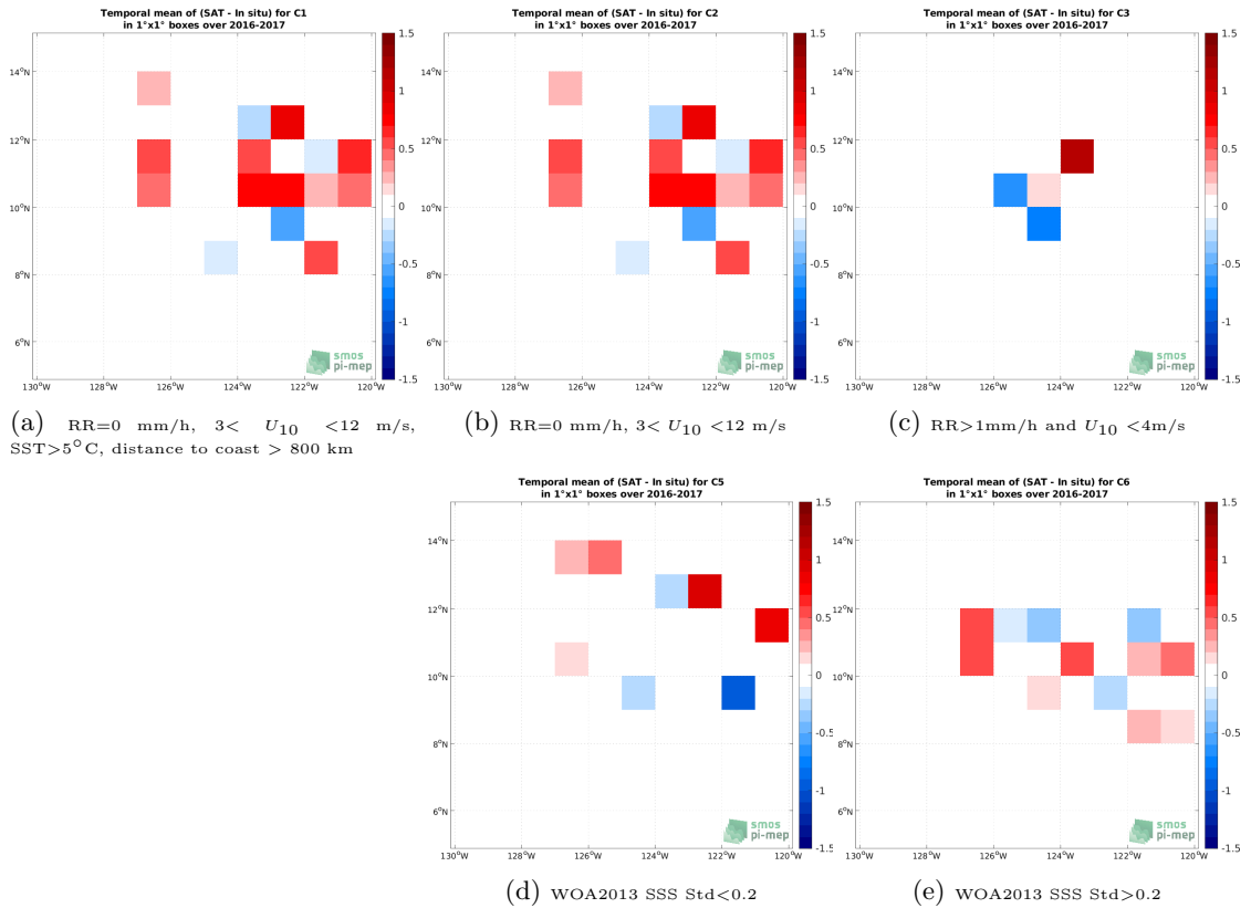
Figure 12: Temporal mean gridded over spatial boxes of size 1^{\circ}\times 1^{\circ} of \Delta\text{SSS} (SMOS SSS L2Q v331 - No FLAG (CMEMS-CATDS-CPDC) - Waveglider (SPURS 2)) for 5 different subdatasets corresponding to:RR=0 mm/h, 3 < U_{10} < 12 m/s, SST >5^{\circ}\text{C} , distance to coast > 800 km (a), RR=0 mm/h, 3 < U_{10} < 12 m/s (b), RR >1 mm/h and U_{10} < 4 m/s (c), WOA2013 SSS Std <0.2 (d), WOA2013 SSS Std >0.2 (e).
