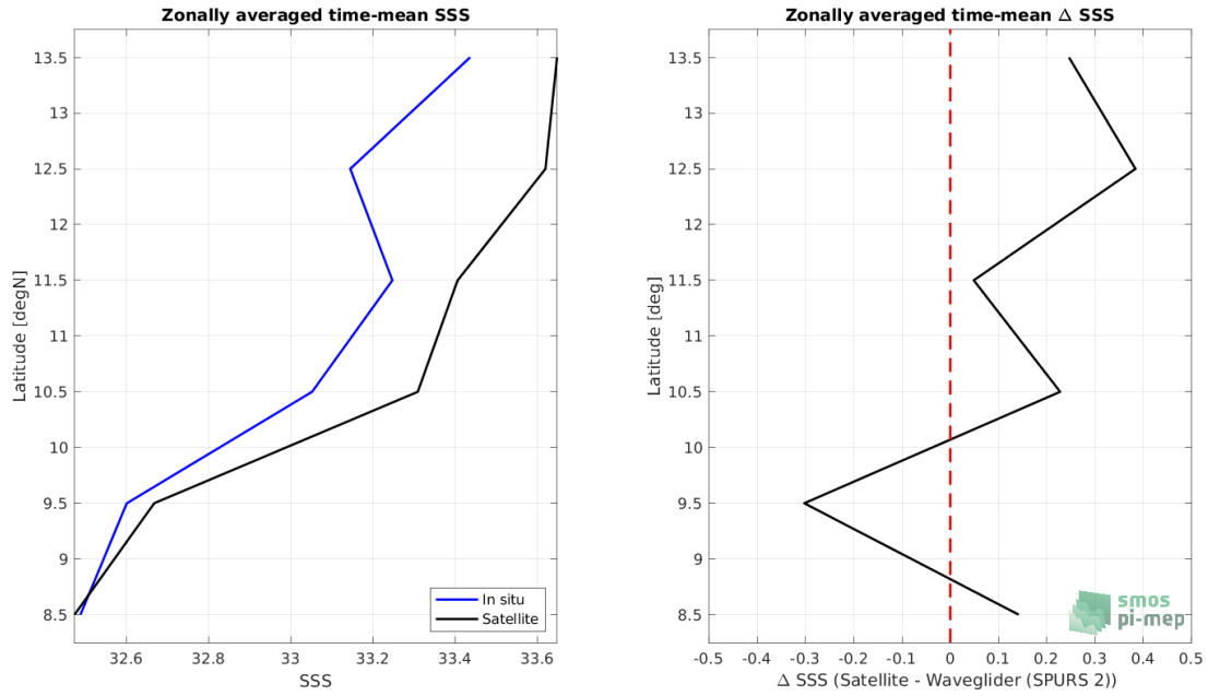
Figure 8: Left panel: Zonal mean SSS from SMOS SSS L2Q v331 - No FLAG (CMEMS-CATDS-CPDC) satellite product (black) and from Waveglider (SPURS 2) (blue). Right panel: Zonal mean of \Delta SSS (Satellite - Waveglider (SPURS 2)) for all the collected Pi-MEP match-up pairs estimated over the full satellite product period.
