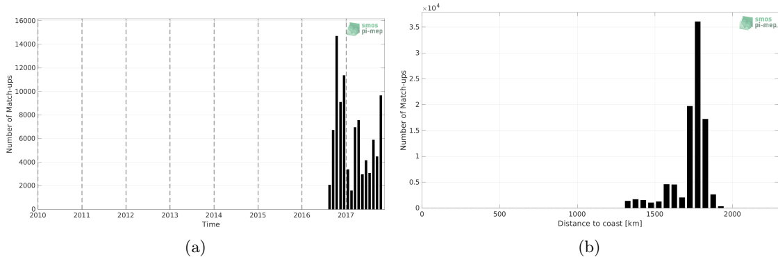
Figure 1: Number of match-ups between Waveglider (SPURS 2) and SMOS SSS L2Q v331 - No FLAG (CMEMS-CATDS-CPDC) SSS as a function of time (a) and as function of the distance to coast (b) over the SPURS 2 Pi-MEP region and for the full satellite product period.
