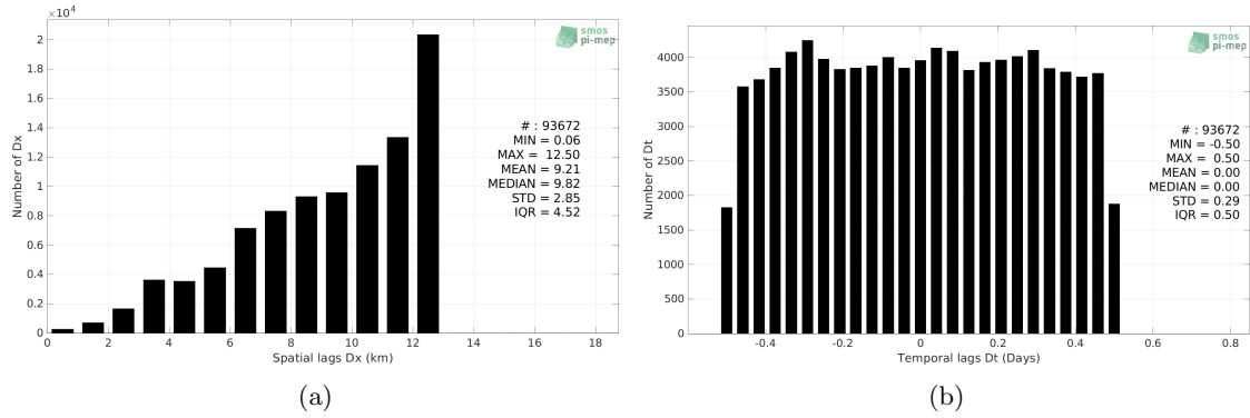
Figure 5: Histograms of the spatial (a) and temporal (b) lags between the location/time of the Waveglider (SPURS 2) measurement and the date of the corresponding SMOS SSS L2Q v331 - No FLAG (CMEMS-CATDS-CPDC) SSS pixel.
