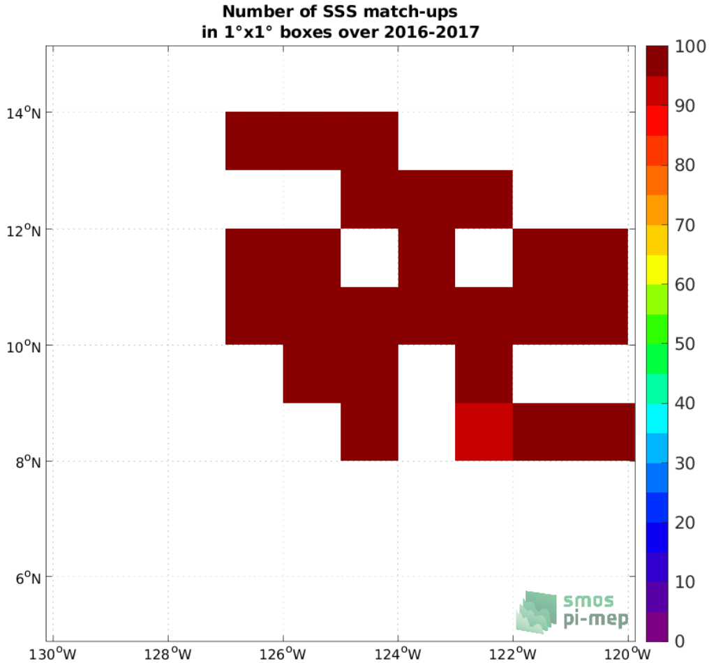
Figure 4: Number of SSS match-ups between Waveglider (SPURS 2) SSS and the SMOS SSS L2Q v331 - No FLAG (CMEMS-CATDS-CPDC) SSS product for the SPURS 2 Pi-MEP region over 1^\circ \times 1^\circ boxes and for the full satellite product period.
