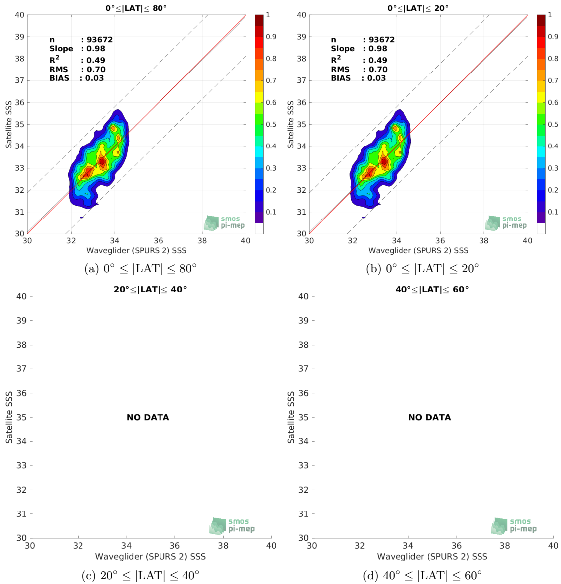
Figure 9: Contour maps of the concentration of SMOS SSS L2Q v331 - No FLAG (CMEMS-CATDS-CPDC) SSS (y-axis) versus Waveglider (SPURS 2) SSS (x-axis) at match-up pairs for different latitude bands. For each plot, the red line shows x=y . The black thin and dashed lines indicate a linear fit through the data cloud and the \pm 95\% confidence levels, respectively. The number match-up pairs n , the slope and R^2 coefficient of the linear fit, the root mean square (RMS) and the mean bias between satellite and in situ data are indicated for each latitude band in each plots.
