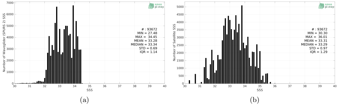
Figure 2: Histograms of SSS from Waveglider (SPURS 2) (a) and SMOS SSS L2Q v331 - No FLAG (CMEMS-CATDS-CPDC) (b) considering all match-up pairs per bins of 0.1 over the SPURS 2 Pi-MEP region and for the full satellite product period.
