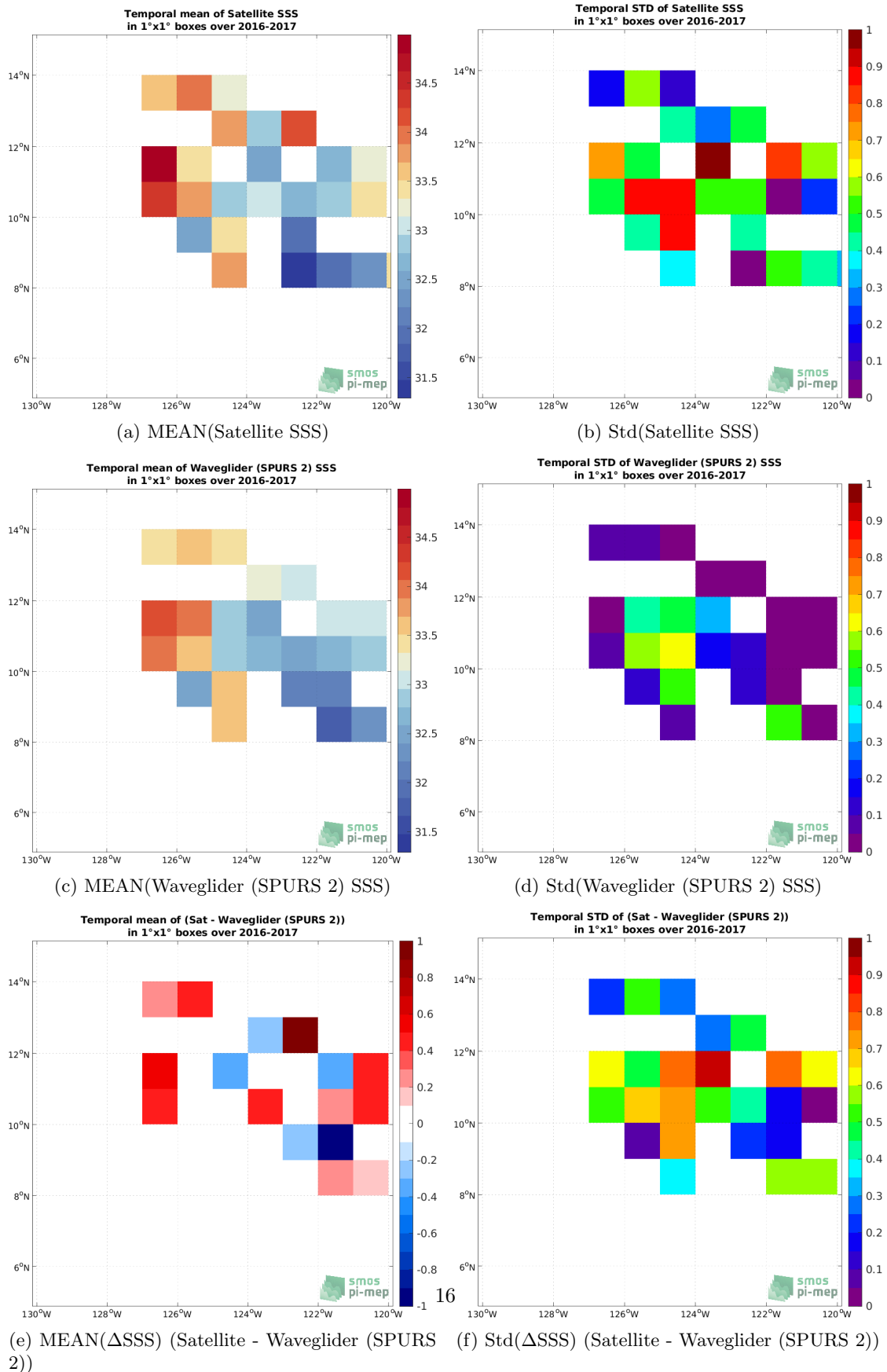
Figure 6: Temporal mean (left) and Std (right) of SSS from SMOS SSS L2Q v331 - No FLAG (CMEMS-CATDS-CPDC) (top), Waveglider (SPURS 2) (middle), and of \Delta SSS (Satellite - Waveglider (SPURS 2)). Only match-up pairs are used to generate these maps.
