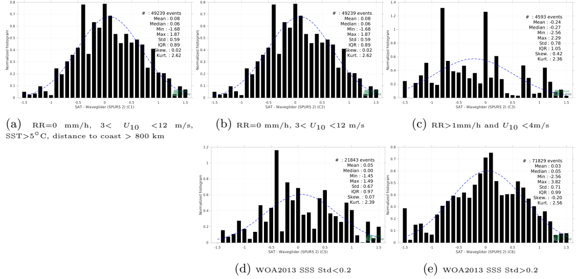
Figure 13: Normalized histogram of \Delta SSS (SMOS SSS L2Q v331 - No FLAG (CMEMS-CATDS-CPDC) - Waveglider (SPURS 2)) for 5 different subdatasets corresponding to: RR=0 mm/h, 3 < U_{10} < 12 m/s, SST > 5°C, distance to coast > 800 km (a), RR=0 mm/h, 3 < U_{10} < 12 m/s (b), RR > 1mm/h and U_{10} < 4 m/s (c), WOA2013 SSS Std < 0.2 (d), WOA2013 SSS Std > 0.2 (e).
