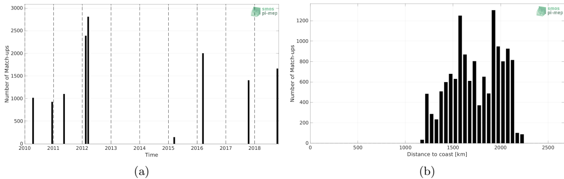
Figure 1: Number of match-ups between TSG (SAMOS) and SMOS SSS L2Q v331 - No FLAG (CMEMS-CATDS-CPDC) SSS as a function of time (a) and as function of the distance to coast (b) over the SPURS 2 Pi-MEP region and for the full satellite product period.
