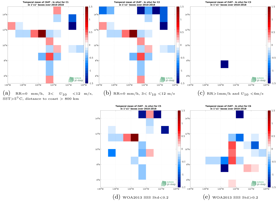
Figure 12: Temporal mean gridded over spatial boxes of size 1^{\circ}\times 1^{\circ} of \Delta\text{SSS} (SMOS SSS L2Q v331 - No FLAG (CMEMS-CATDS-CPDC) - TSG (SAMOS)) for 5 different subdatasets corresponding to:RR=0 mm/h, 3 < U_{10} < 12 m/s, SST >5^{\circ}\text{C} , distance to coast > 800 km (a), RR=0 mm/h, 3 < U_{10} < 12 m/s (b), RR >1 mm/h and U_{10} < 4 m/s (c), WOA2013 SSS Std <0.2 (d), WOA2013 SSS Std >0.2 (e).
