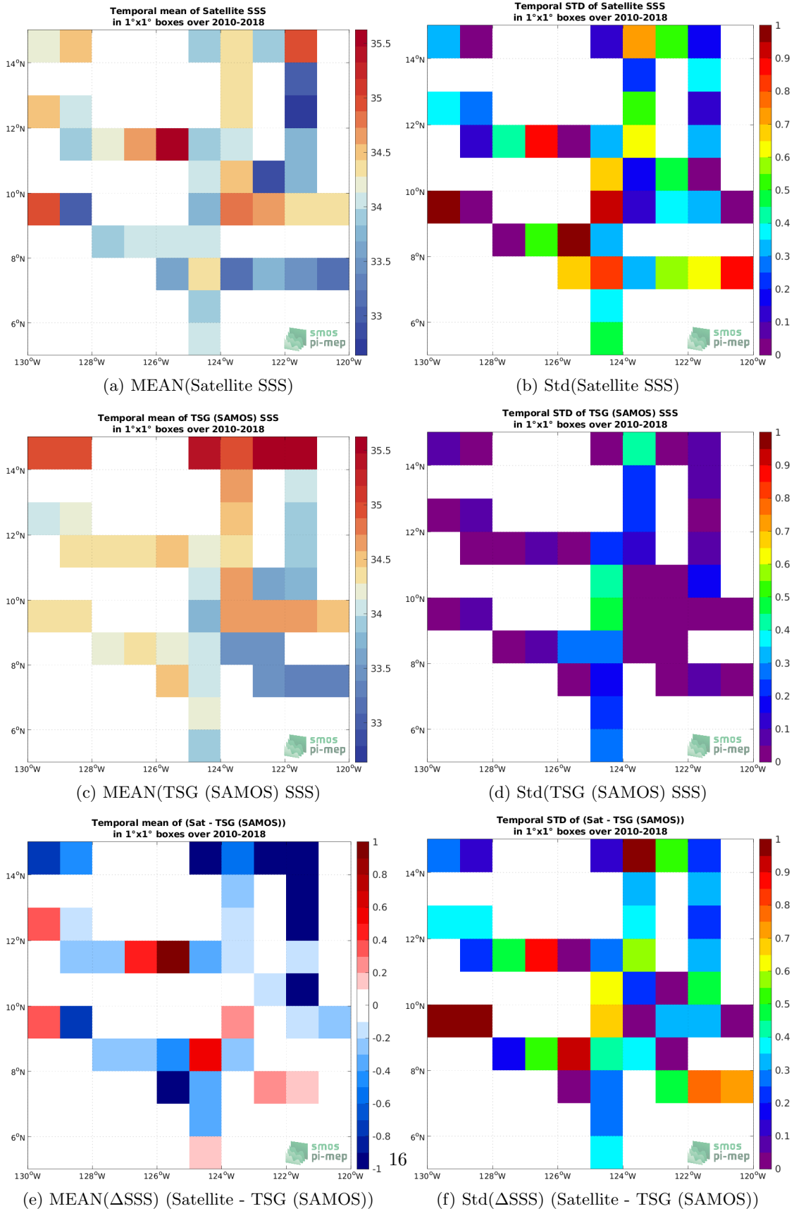
Figure 6: Temporal mean (left) and Std (right) of SSS from SMOS SSS L2Q v331 - No FLAG (CMEMS-CATDS-CPDC) (top), TSG (SAMOS) (middle), and of \Delta SSS (Satellite - TSG (SAMOS)). Only match-up pairs are used to generate these maps.
