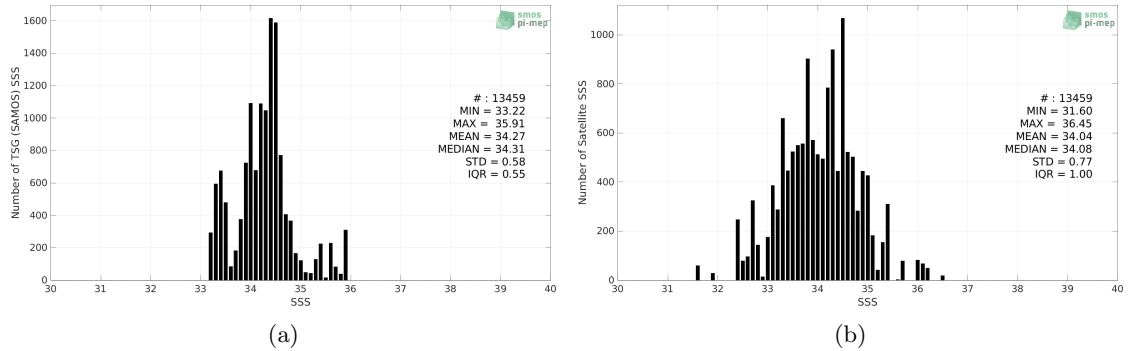
Figure 2: Histograms of SSS from TSG (SAMOS) (a) and SMOS SSS L2Q v331 - No FLAG (CMEMS-CATDS-CPDC) (b) considering all match-up pairs per bins of 0.1 over the SPURS 2 Pi-MEP region and for the full satellite product period.
