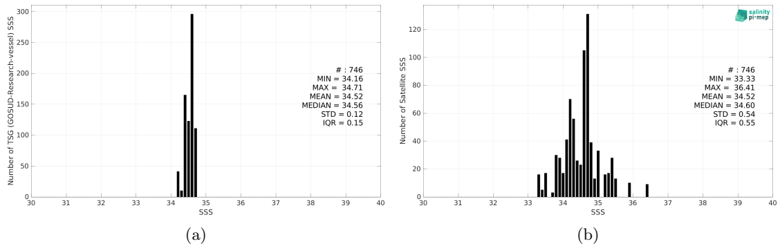
Figure 2: Histograms of SSS from TSG (GOSUD-Research-vessel) (a) and SMOS SSS L2Q v331 - No FLAG (CMEMS-CATDS-CPDC) (b) considering all match-up pairs per bins of 0.1 over the SPURS 2 Pi-MEP region and for the full satellite product period.
