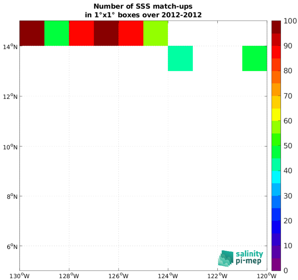
Figure 4: Number of SSS match-ups between TSG (GOSUD-Research-vessel) SSS and the SMOS SSS L2Q v331 - No FLAG (CMEMS-CATDS-CPDC) SSS product for the SPURS 2 Pi-MEP region over 1^\circ \times 1^\circ boxes and for the full satellite product period.
