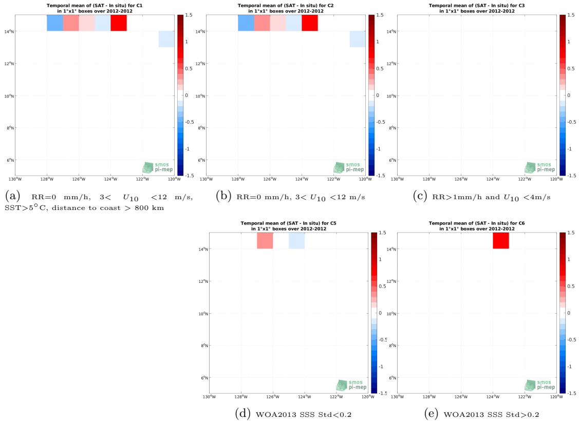
Figure 12: Temporal mean gridded over spatial boxes of size 1^{\circ} \times 1^{\circ} of \Delta SSS (SMOS SSS L2Q v331 - No FLAG (CMEMS-CATDS-CPDC) - TSG (GOSUD-Research-vessel)) for 5 different subdatasets corresponding to: RR=0 mm/h, 3 < U_{10} < 12 m/s, SST > 5^{\circ}C , distance to coast > 800 km (a), RR=0 mm/h, 3 < U_{10} < 12 m/s (b), RR > 1 mm/h and U_{10} < 4 m/s (c), WOA2013 SSS Std < 0.2 (d), WOA2013 SSS Std > 0.2 (e).
