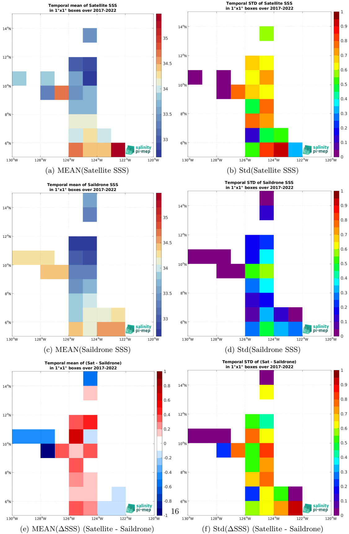
Figure 7: Temporal mean (left) and Std (right) of SSS from SMOS SSS L2Q v331 - No FLAG (CMEMS-CATDS-CPDC) (top), Saildrone (middle), and of \Delta SSS (Satellite - Saildrone). Only match-up pairs are used to generate these maps.
