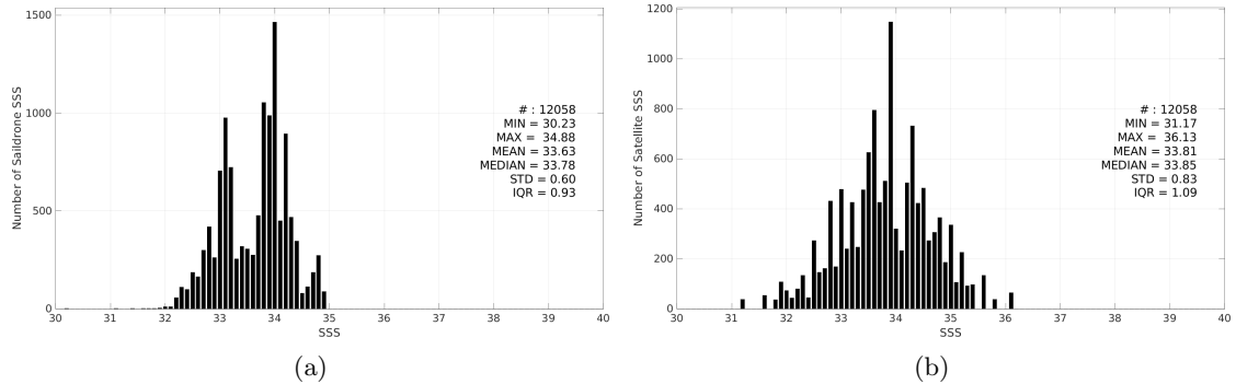
Figure 3: Histograms of SSS from Saildrone (a) and SMOS SSS L2Q v331 - No FLAG (CMEMS-CATDS-CPDC) (b) considering all match-up pairs per bins of 0.1 over the SPURS 2 Pi-MEP region and for the full satellite product period.
