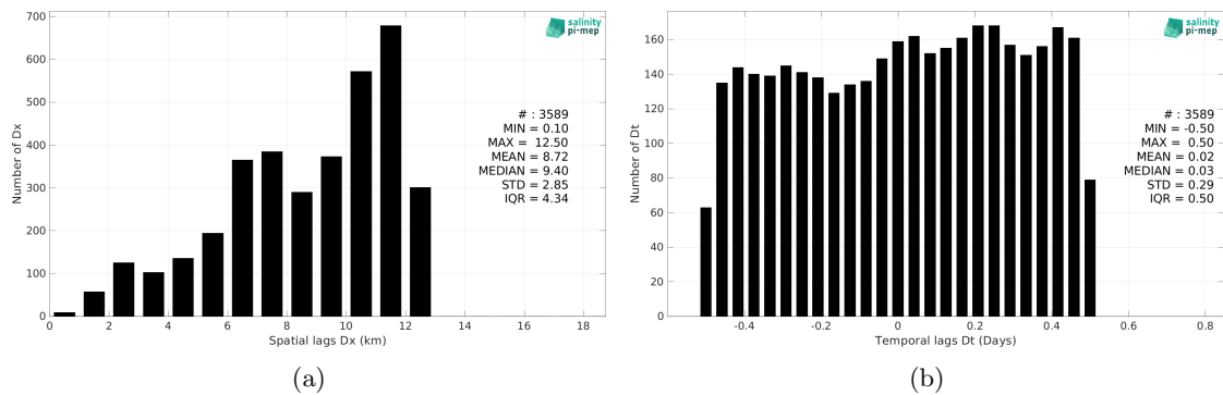
Figure 6: Histograms of the spatial (a) and temporal (b) lags between the location/time of the Saildrone (SPURS 2) measurement and the date of the corresponding SMOS SSS L2Q v331 - No FLAG (CMEMS-CATDS-CPDC) SSS pixel.
