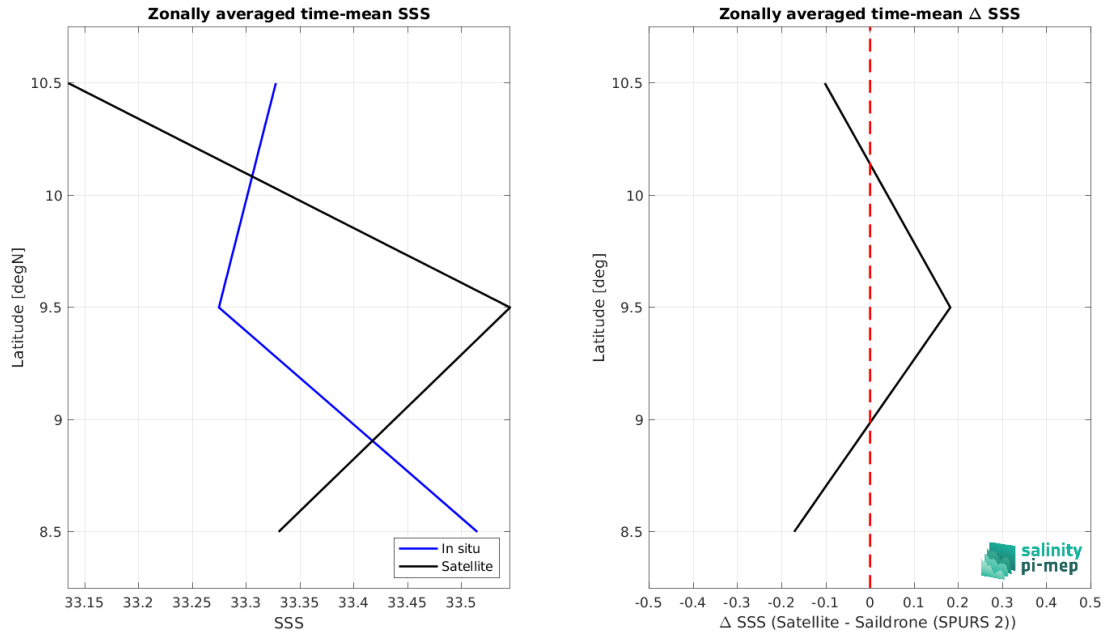
Figure 9: Left panel: Zonal mean SSS from SMOS SSS L2Q v331 - No FLAG (CMEMS-CATDS-CPDC) satellite product (black) and from Sairdron (SPURS 2) (blue). Right panel: Zonal mean of \Delta SSS (Satellite - Sairdron (SPURS 2)) for all the collected Pi-MEP match-up pairs estimated over the full satellite product period.
