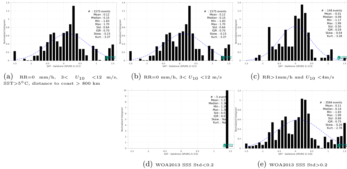
Figure 15: Normalized histogram of \Delta SSS (SMOS SSS L2Q v331 - No FLAG (CMEMS-CATDS-CPDC) - Saildrone (SPURS 2)) for 5 different subdatasets corresponding to: RR=0 mm/h, 3 < U_{10} < 12 m/s, SST>5°C, distance to coast > 800 km (a), RR=0 mm/h, 3 < U_{10} < 12 m/s (b), RR>1mm/h and U_{10} < 4 m/s (c), WOA2013 SSS Std<0.2 (d), WOA2013 SSS Std>0.2 (e).
