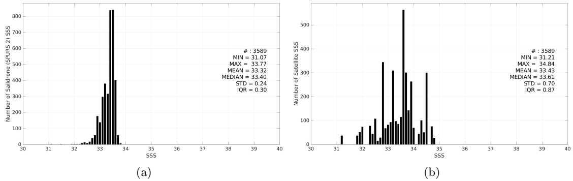
Figure 3: Histograms of SSS from Saildrone (SPURS 2) (a) and SMOS SSS L2Q v331 - No FLAG (CMEMS-CATDS-CPDC) (b) considering all match-up pairs per bins of 0.1 over the SPURS 2 Pi-MEP region and for the full satellite product period.
