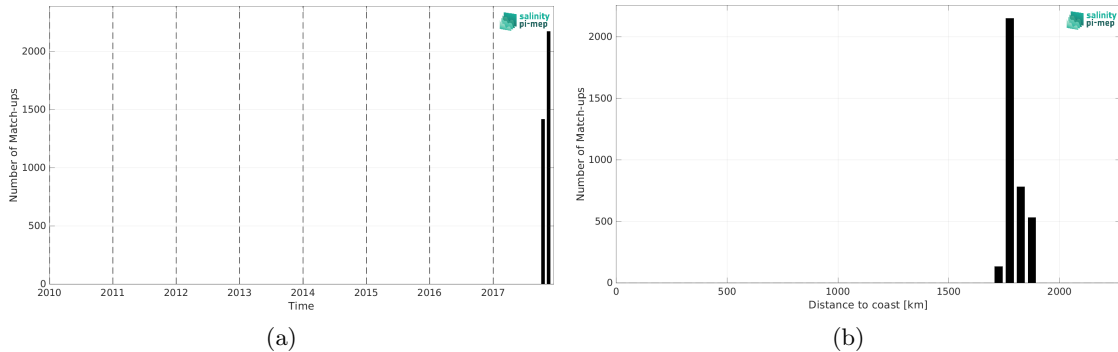
Figure 2: Number of match-ups between Sairdrone (SPURS 2) and SMOS SSS L2Q v331 - No FLAG (CMEMS-CATDS-CPDC) SSS as a function of time (a) and as function of the distance to coast (b) over the SPURS 2 Pi-MEP region and for the full satellite product period.
