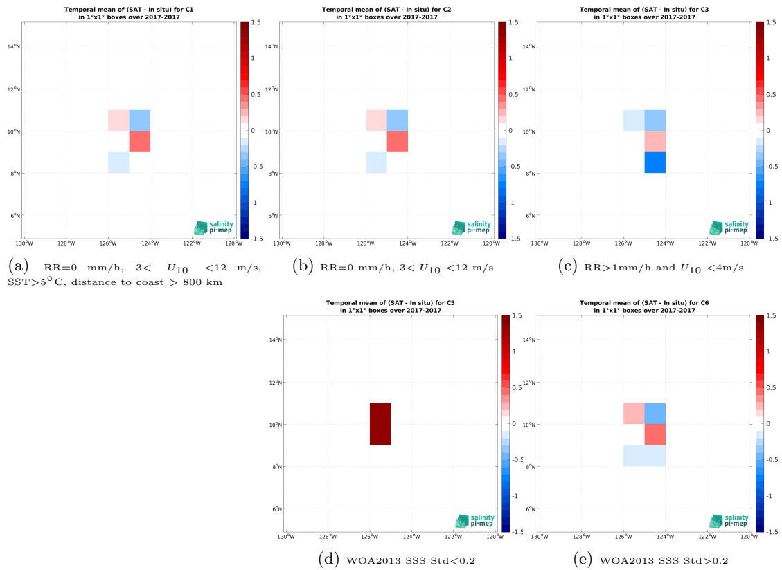
Figure 14: Temporal mean gridded over spatial boxes of size 1^\circ \times 1^\circ of \Delta SSS (SMOS SSS L2Q v331 - No FLAG (CMEMS-CATDS-CPDC) - Saildrone (SPURS 2)) for 5 different subdatasets corresponding to:RR=0 mm/h, 3 < U_{10} < 12 m/s, SST >5^\circ C, distance to coast > 800 km (a), RR=0 mm/h, 3 < U_{10} < 12 m/s (b), RR >1 mm/h and U_{10} < 4 m/s (c), WOA2013 SSS Std <0.2 (d), WOA2013 SSS Std >0.2 (e).
