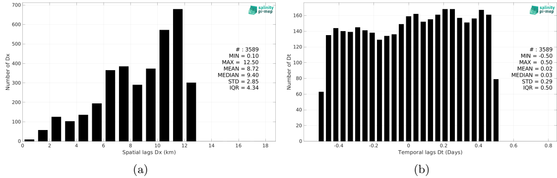
Figure 5: Histograms of the spatial (a) and temporal (b) lags between the location/time of the Saildrone (SPURS 2) measurement and the date of the corresponding SMOS SSS L2Q v331 - No FLAG (CMEMS-CATDS-CPDC) SSS pixel.
