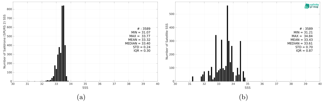
Figure 2: Histograms of SSS from Saildrone (SPURS 2) (a) and SMOS SSS L2Q v331 - No FLAG (CMEMS-CATDS-CPDC) (b) considering all match-up pairs per bins of 0.1 over the SPURS 2 Pi-MEP region and for the full satellite product period.
