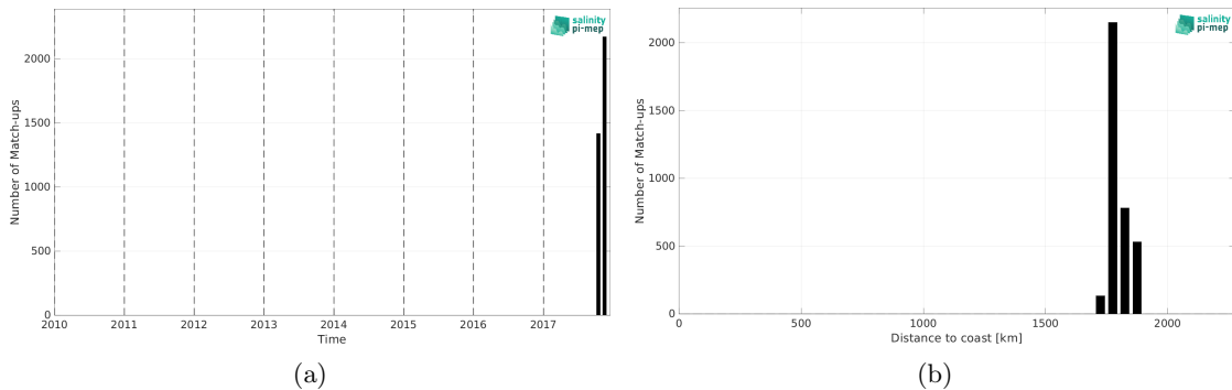
Figure 1: Number of match-ups between Saildrone (SPURS 2) and SMOS SSS L2Q v331 - No FLAG (CMEMS-CATDS-CPDC) SSS as a function of time (a) and as function of the distance to coast (b) over the SPURS 2 Pi-MEP region and for the full satellite product period.
