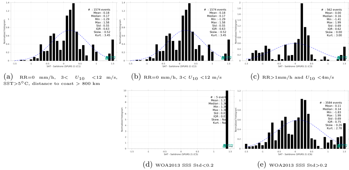
Figure 13: Normalized histogram of \Delta SSS (SMOS SSS L2Q v331 - No FLAG (CMEMS-CATDS-CPDC) - Saildrone (SPURS 2)) for 5 different subdatasets corresponding to: RR=0 mm/h, 3 < U_{10} < 12 m/s, SST > 5°C, distance to coast > 800 km (a), RR=0 mm/h, 3 < U_{10} < 12 m/s (b), RR > 1mm/h and U_{10} < 4 m/s (c), WOA2013 SSS Std < 0.2 (d), WOA2013 SSS Std > 0.2 (e).
