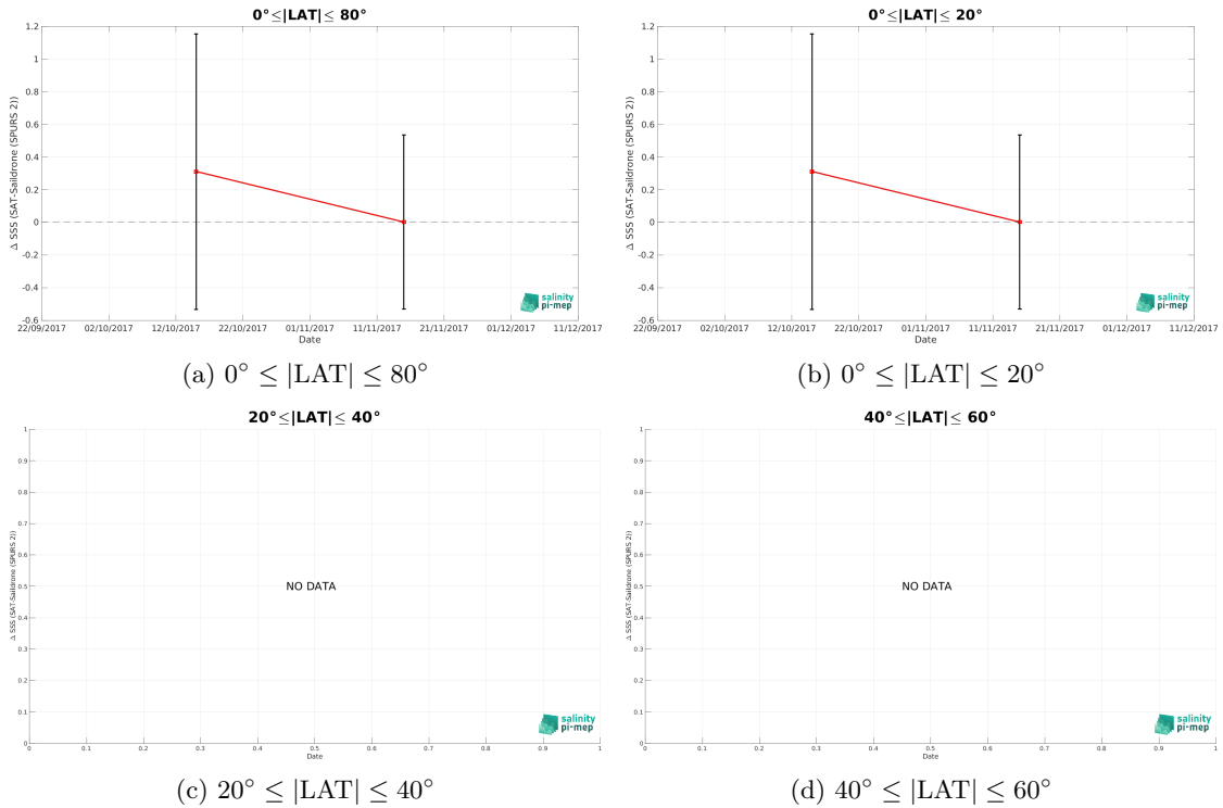
Figure 10: Monthly median (red curves) of \Delta SSS (Satellite - Saildrone (SPURS 2)) and \pm 1 Std (black vertical thick bars) as function of time for all the collected Pi-MEP match-up pairs estimated over the SPURS 2 Pi-MEP region and for the full satellite product period are shown for different latitude bands: (a) 80°S-80°N, (b) 20°S-20°N, (c) 40°S-20°S and 20°N-40°N and (d) 60°S-40°S and 40°N-60°N.
