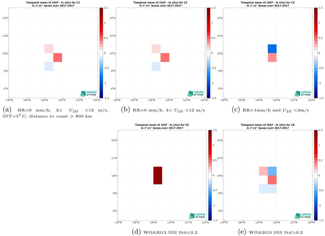
Figure 12: Temporal mean gridded over spatial boxes of size 1^{\circ}\times 1^{\circ} of \Delta\text{SSS} (SMOS SSS L2Q v331 - No FLAG (CMEMS-CATDS-CPDC) - Saildrone (SPURS 2)) for 5 different subdatasets corresponding to:RR=0 mm/h, 3 < U_{10} < 12 m/s, SST >5^{\circ}\text{C} , distance to coast > 800 km (a), RR=0 mm/h, 3 < U_{10} < 12 m/s (b), RR >1 mm/h and U_{10} < 4 m/s (c), WOA2013 SSS Std <0.2 (d), WOA2013 SSS Std >0.2 (e).
