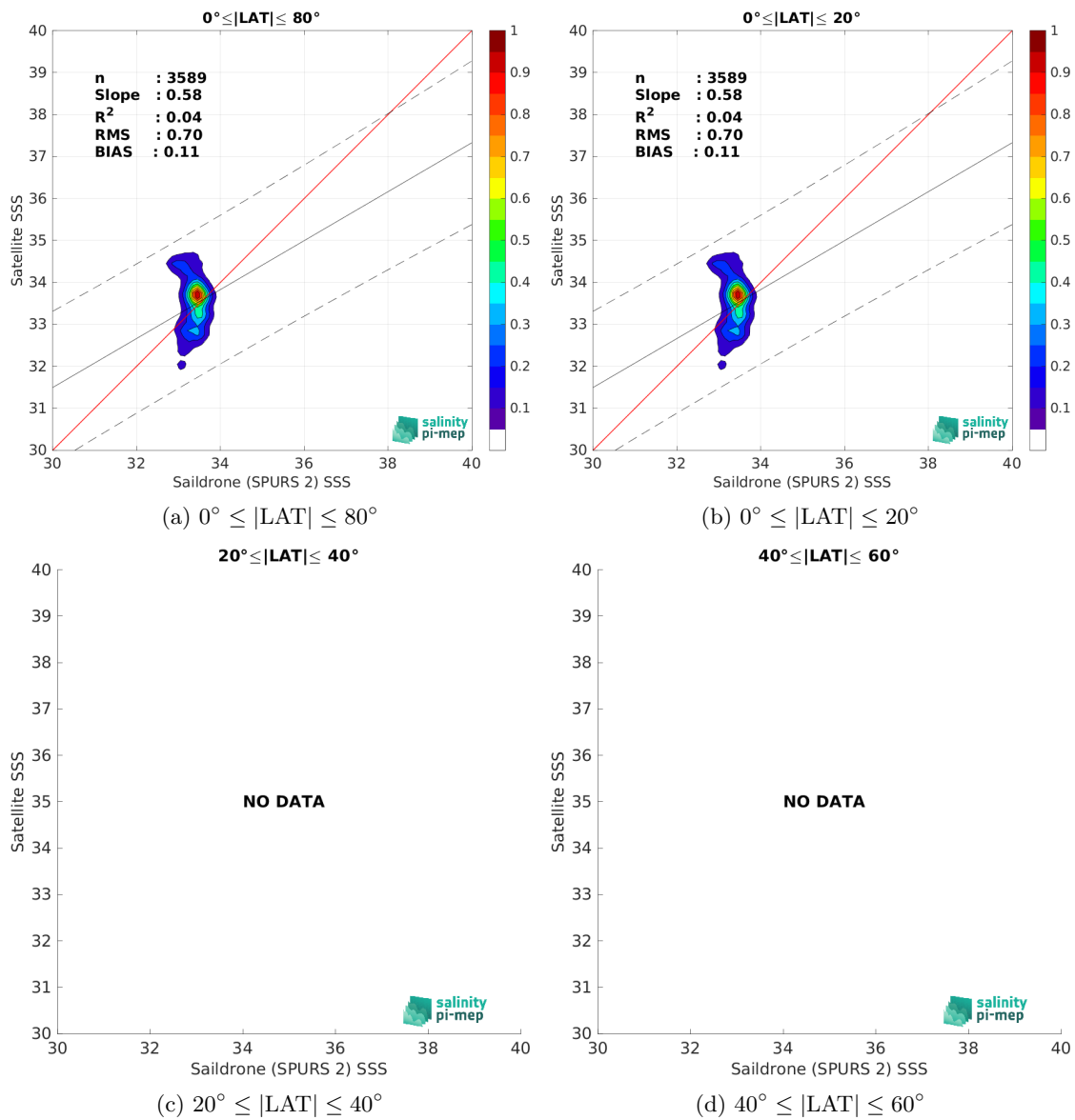
Figure 9: Contour maps of the concentration of SMOS SSS L2Q v331 - No FLAG (CMEMS-CATDS-CPDC) SSS (y-axis) versus Saildrone (SPURS 2) SSS (x-axis) at match-up pairs for different latitude bands. For each plot, the red line shows x=y . The black thin and dashed lines indicate a linear fit through the data cloud and the \pm 95\% confidence levels, respectively. The number match-up pairs n , the slope and R^2 coefficient of the linear fit, the root mean square (RMS) and the mean bias between satellite and in situ data are indicated for each latitude band in each plots.
