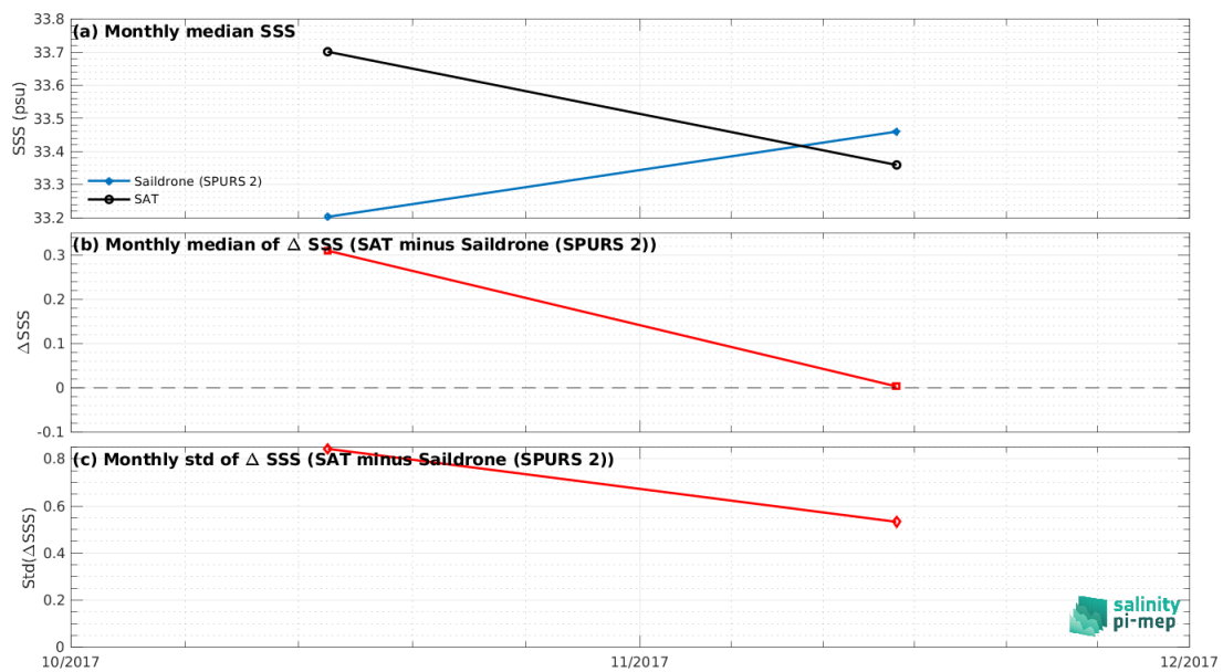
Figure 7: Time series of the monthly median SSS (top), median of \Delta SSS (Satellite - Sairdronne (SPURS 2)) and Std of \Delta SSS (Satellite - Sairdronne (SPURS 2)) over the SPURS 2 Pi-MEP region considering all match-ups collected by the Pi-MEP.
