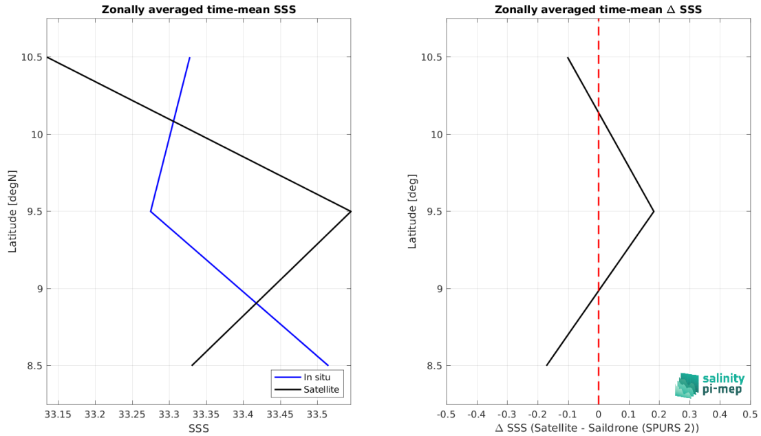
Figure 8: Left panel: Zonal mean SSS from SMOS SSS L2Q v331 - No FLAG (CMEMS-CATDS-CPDC) satellite product (black) and from Sairdron (SPURS 2) (blue). Right panel: Zonal mean of \Delta SSS (Satellite - Sairdron (SPURS 2)) for all the collected Pi-MEP match-up pairs estimated over the full satellite product period.
