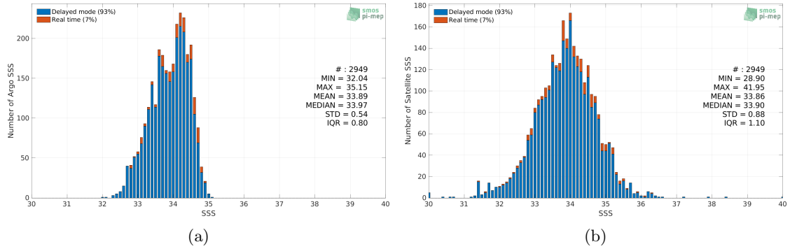
Figure 2: Histograms of SSS from Argo (a) and SMOS SSS L2Q v331 - No FLAG (CMEMS-CATDS-CPDC) (b) considering all match-up pairs per bins of 0.1 over the SPURS 2 Pi-MEP region and for the full satellite product period.
