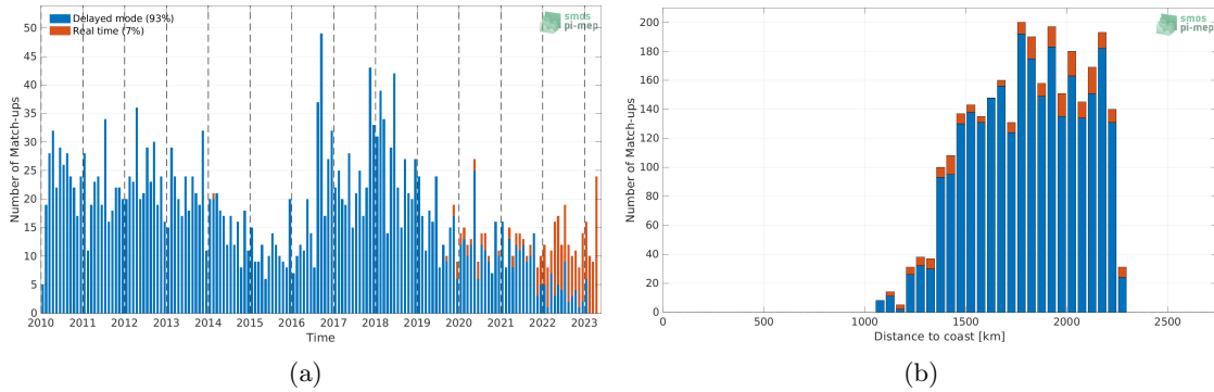
Figure 1: Number of match-ups between Argo and SMOS SSS L2Q v331 - No FLAG (CMEMS-CATDS-CPDC) SSS as a function of time (a) and as function of the distance to coast (b) over the SPURS 2 Pi-MEP region and for the full satellite product period.
