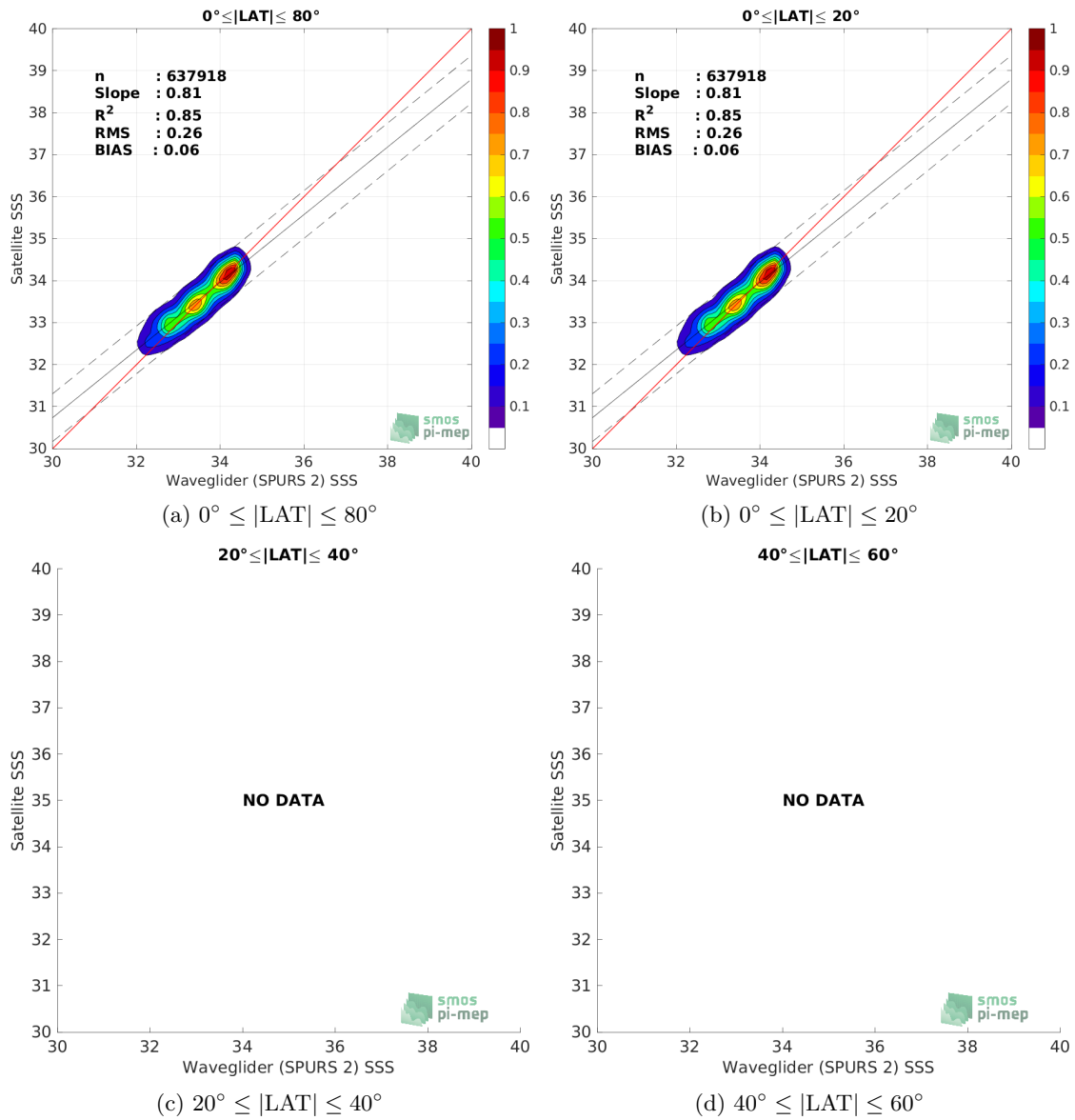
Figure 9: Contour maps of the concentration of SMOS SSS L3 v8 - 18 Days (CATDS-CECOS-LOCEAN) SSS (y-axis) versus Waveglider (SPURS 2) SSS (x-axis) at match-up pairs for different latitude bands. For each plot, the red line shows x=y . The black thin and dashed lines indicate a linear fit through the data cloud and the \pm 95\% confidence levels, respectively. The number match-up pairs n , the slope and R^2 coefficient of the linear fit, the root mean square (RMS) and the mean bias between satellite and in situ data are indicated for each latitude band in each plots.
