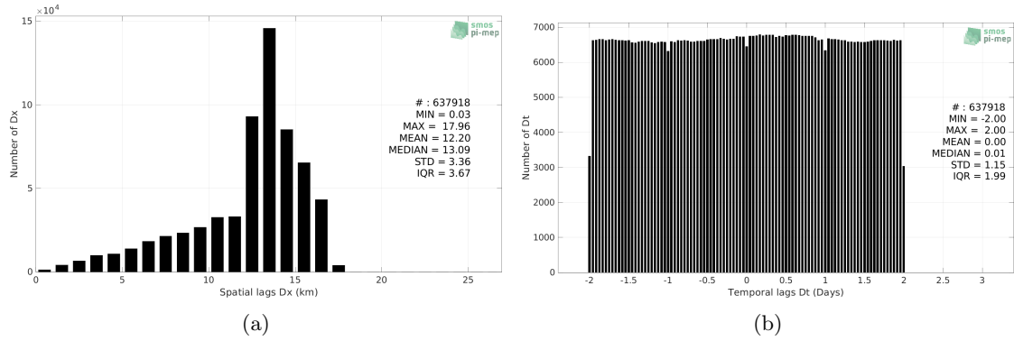
Figure 5: Histograms of the spatial (a) and temporal (b) lags between the location/time of the Waveglider (SPURS 2) measurement and the date of the corresponding SMOS SSS L3 v8 - 18 Days (CATDS-CECOS-LOCEAN) SSS pixel.
