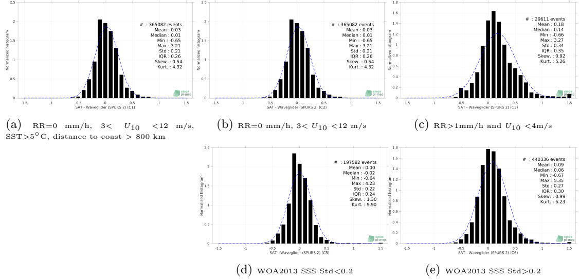
Figure 13: Normalized histogram of \Delta SSS (SMOS SSS L3 v8 - 18 Days (CATDS-CECOS-LOCEAN) - Waveglider (SPURS 2)) for 5 different subdatasets corresponding to: RR=0 mm/h, 3 < U_{10} < 12 m/s, SST>5°C, distance to coast > 800 km (a), RR=0 mm/h, 3 < U_{10} < 12 m/s (b), RR>1mm/h and U_{10} < 4 m/s (c), WOA2013 SSS Std<0.2 (d), WOA2013 SSS Std>0.2 (e).
