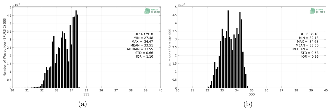
Figure 2: Histograms of SSS from Waveglider (SPURS 2) (a) and SMOS SSS L3 v8 - 18 Days (CATDS-CECOS-LOCEAN) (b) considering all match-up pairs per bins of 0.1 over the SPURS 2 Pi-MEP region and for the full satellite product period.
