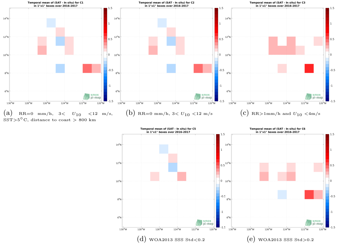
Figure 12: Temporal mean gridded over spatial boxes of size 1^{\circ}\times 1^{\circ} of \Delta\text{SSS} (SMOS SSS L3 v8 - 18 Days (CATDS-CECOS-LOCEAN) - Waveglider (SPURS 2)) for 5 different subdatasets corresponding to:RR=0 mm/h, 3 < U_{10} < 12 m/s, SST >5^{\circ}\text{C} , distance to coast > 800 km (a), RR=0 mm/h, 3 < U_{10} < 12 m/s (b), RR >1 mm/h and U_{10} < 4 m/s (c), WOA2013 SSS Std <0.2 (d), WOA2013 SSS Std >0.2 (e).
