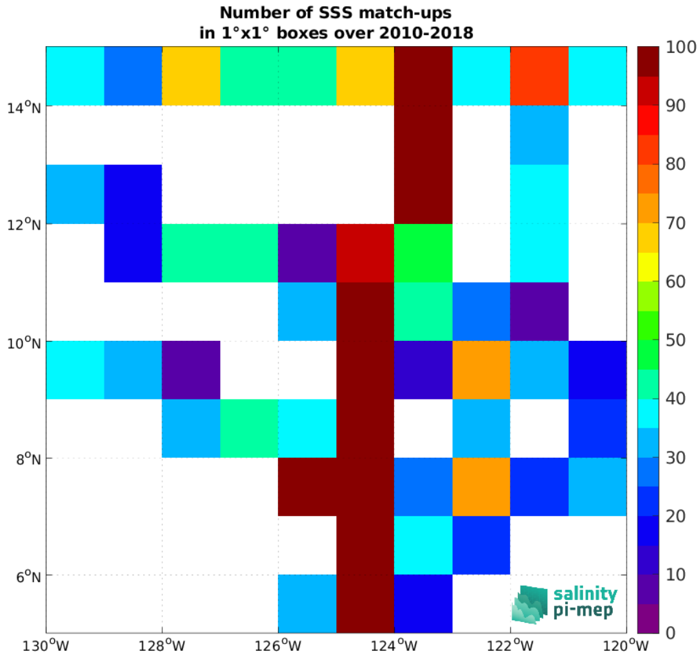
Figure 4: Number of SSS match-ups between TSG (SAMOS) SSS and the SMOS SSS L3 v8 - 18 Days (CATDS-CEC-LOCEAN) SSS product for the SPURS 2 Pi-MEP region over 1^\circ \times 1^\circ boxes and for the full satellite product period.
