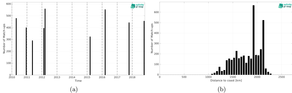
Figure 1: Number of match-ups between TSG (SAMOS) and SMOS SSS L3 v8 - 18 Days (CATDS-CEC-LOCEAN) SSS as a function of time (a) and as function of the distance to coast (b) over the SPURS 2 Pi-MEP region and for the full satellite product period.
