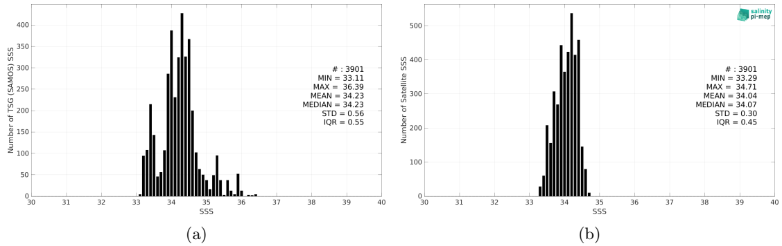
Figure 2: Histograms of SSS from TSG (SAMOS) (a) and SMOS SSS L3 v8 - 18 Days (CATDS-CEC-LOCEAN) (b) considering all match-up pairs per bins of 0.1 over the SPURS 2 Pi-MEP region and for the full satellite product period.
